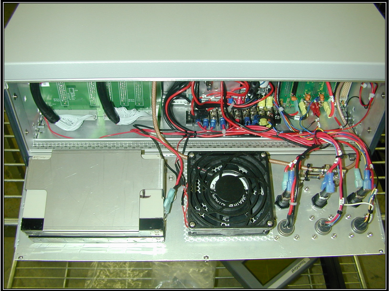
PHOTOGRAPH 5: BACK OF EUT WITH COVER OPEN
