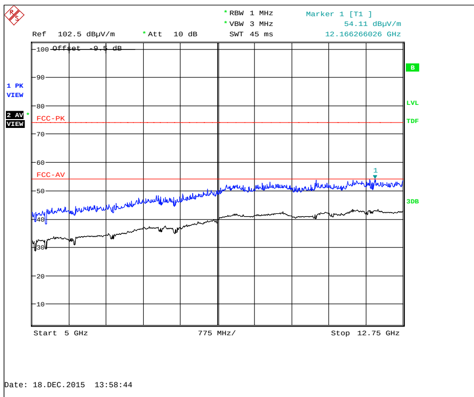
802.11 Channel 11 : 5 GHz to 12.75 GHz
