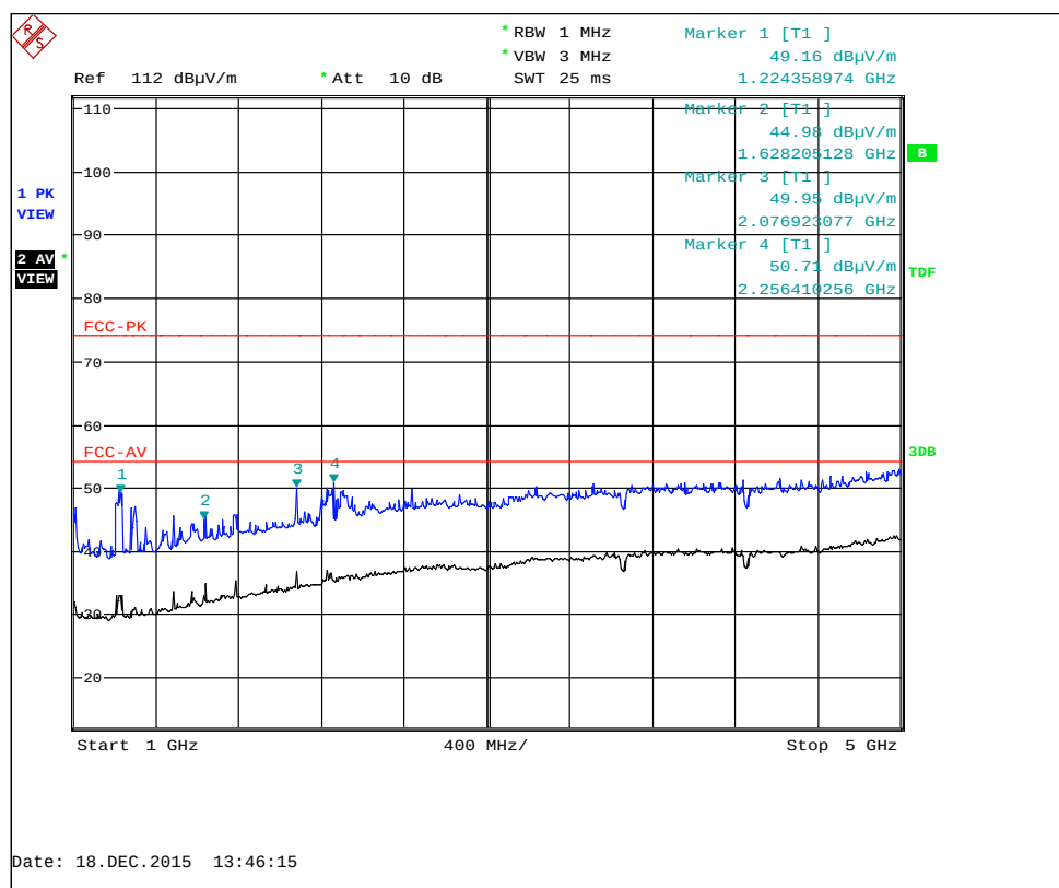
802.11 Channel 6 : 1 GHz to 5 GHz
