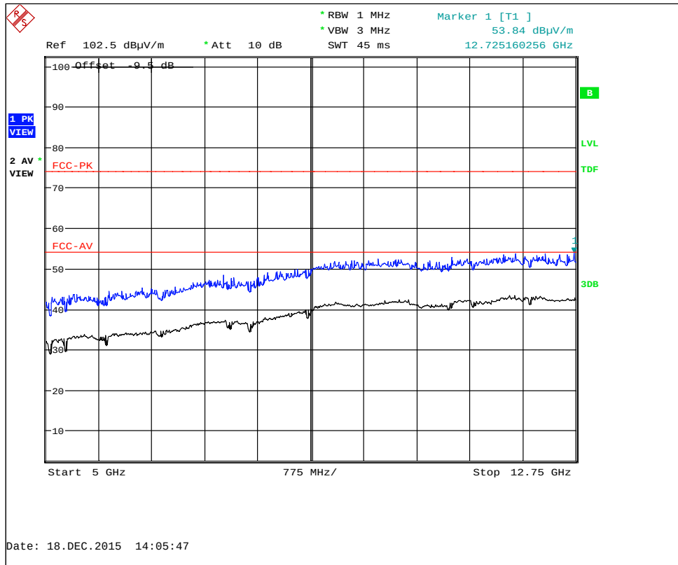
802.11 Channel 6 : 5 GHz to 12.75 GHz
