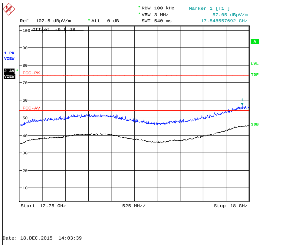
802.11 Channel 6 : 12.75 GHz to 18 GHz
