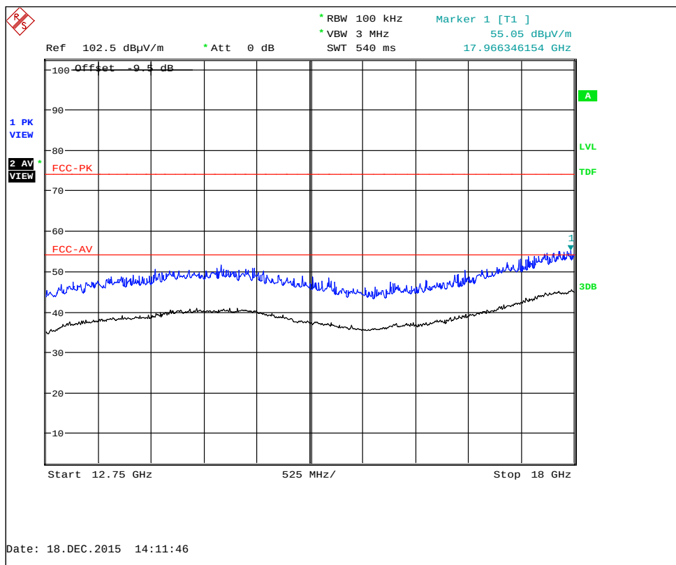
802.11 Channel 1 : 12.75 GHz to 18 GHz
