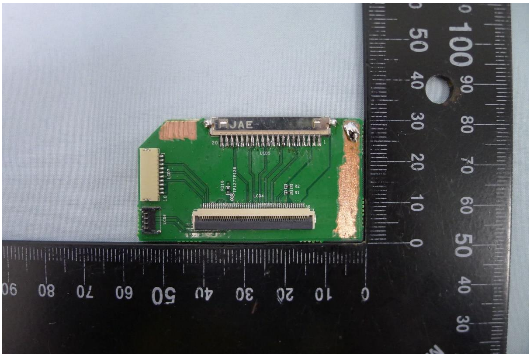
( 34 ) EUT Photo_Monarch 8 inch (BUTTERFLYMX.M08)
