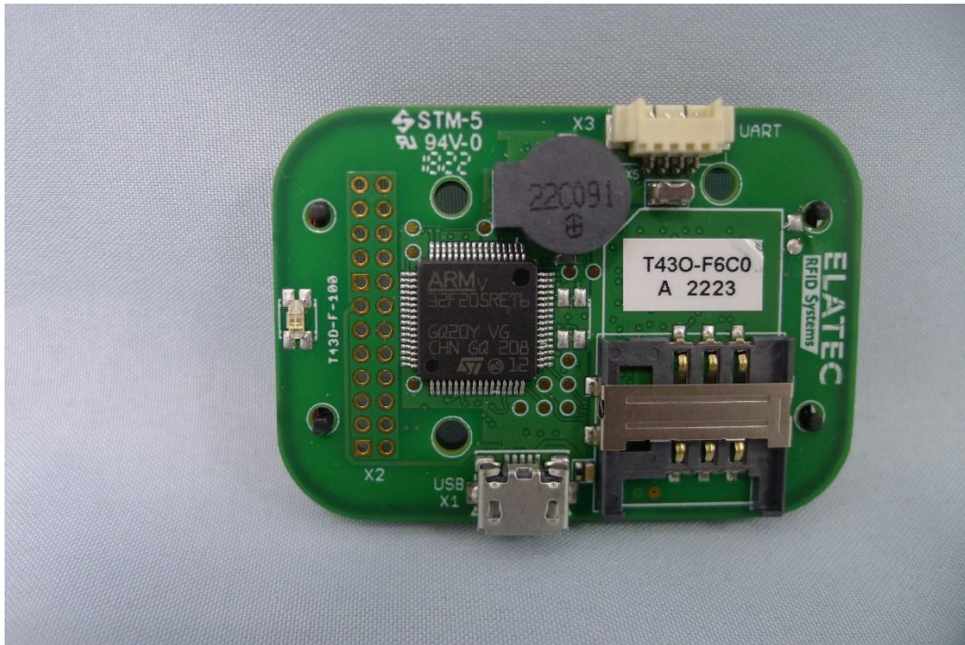
( 42 ) EUT Photo_Monarch 8 inch (BUTTERFLYMX.M08)
