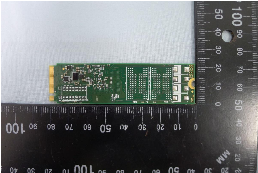
( 8 ) EUT Photo_Monarch 8 inch (BUTTERFLYMX.M08)
