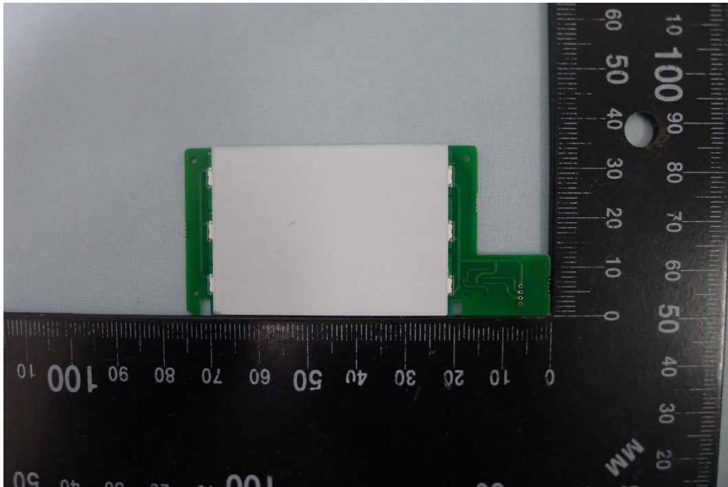
( 40 ) EUT Photo_Monarch 8 inch (BUTTERFLYMX.M08)
