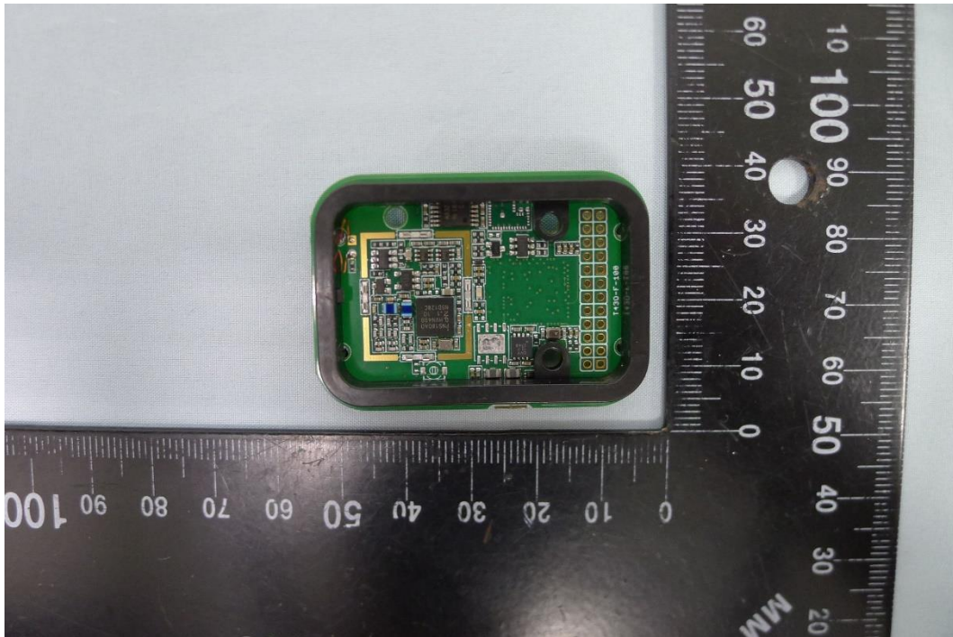
( 46 ) EUT Photo_Monarch 8 inch (BUTTERFLYMX.M08)
