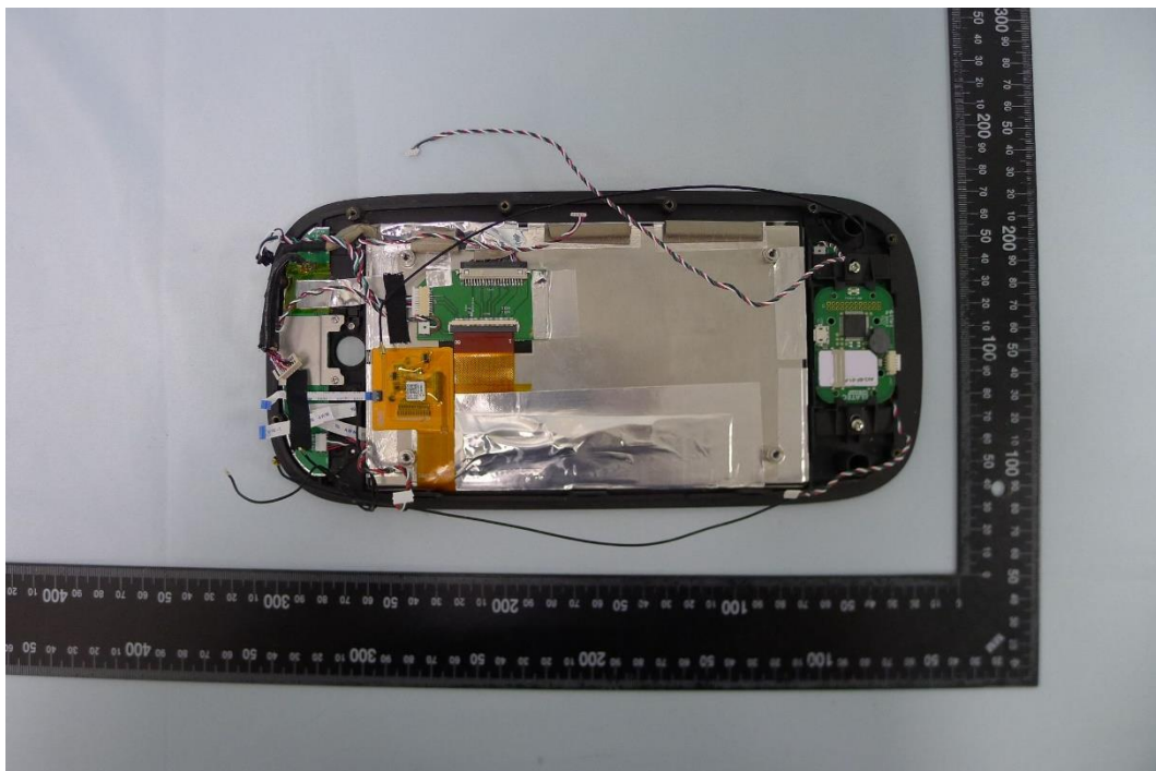
( 32 ) EUT Photo_Monarch 8 inch (BUTTERFLYMX.M08)
