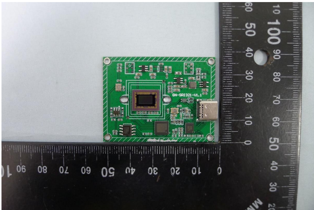
( 30 ) EUT Photo_Monarch 8 inch (BUTTERFLYMX.M08)
