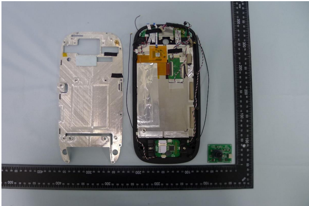
( 28 ) EUT Photo_Monarch 8 inch (BUTTERFLYMX.M08)
