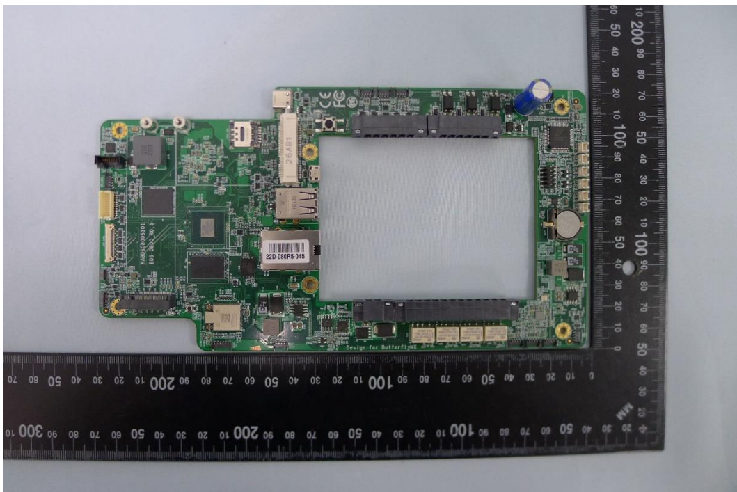
( 18 ) EUT Photo_Monarch 8 inch (BUTTERFLYMX.M08)
