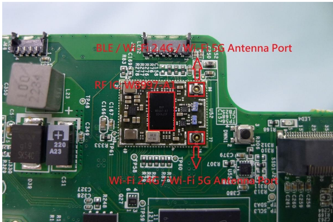
( 22 ) EUT Photo_Monarch 8 inch (BUTTERFLYMX.M08)
