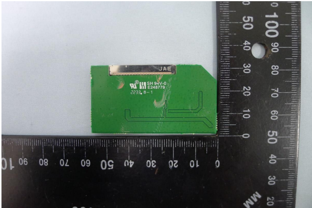
( 36 ) EUT Photo_Monarch 8 inch (BUTTERFLYMX.M08)
