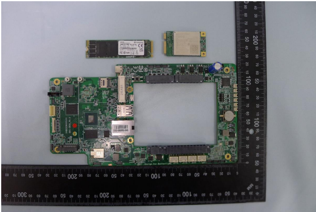
( 6 ) EUT Photo_Monarch 8 inch (BUTTERFLYMX.M08)
