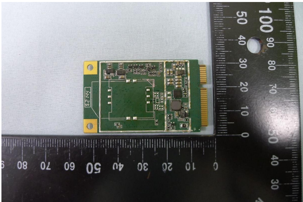
( 14 ) EUT Photo_Monarch 8 inch (BUTTERFLYMX.M08)
