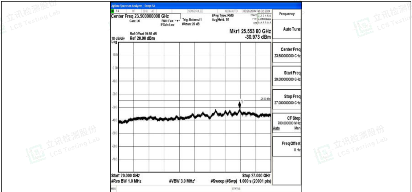
Band41_15MHz_QPSK_41515_1RB#0_20000~27000_20000~27000
