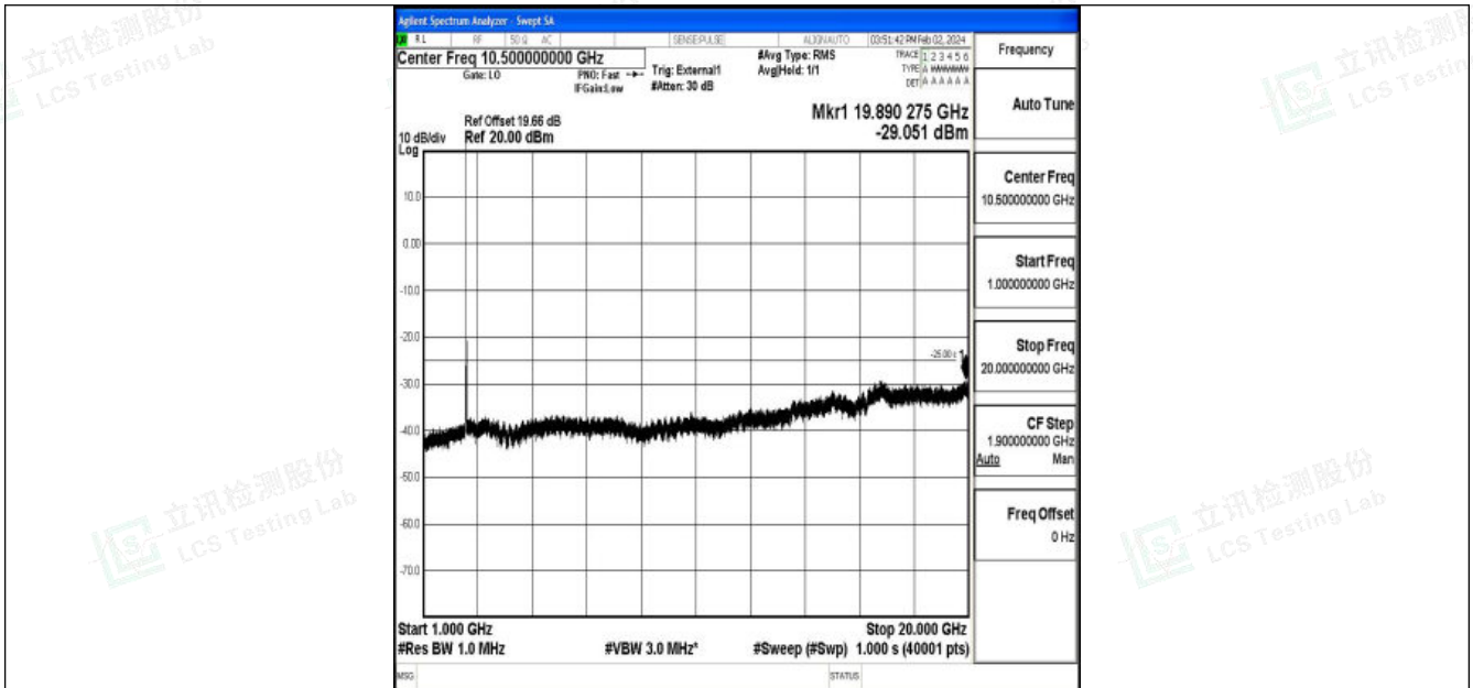
Band41_20MHz_16QAM_39750_1RB#0_1000~20000_1000~20000
