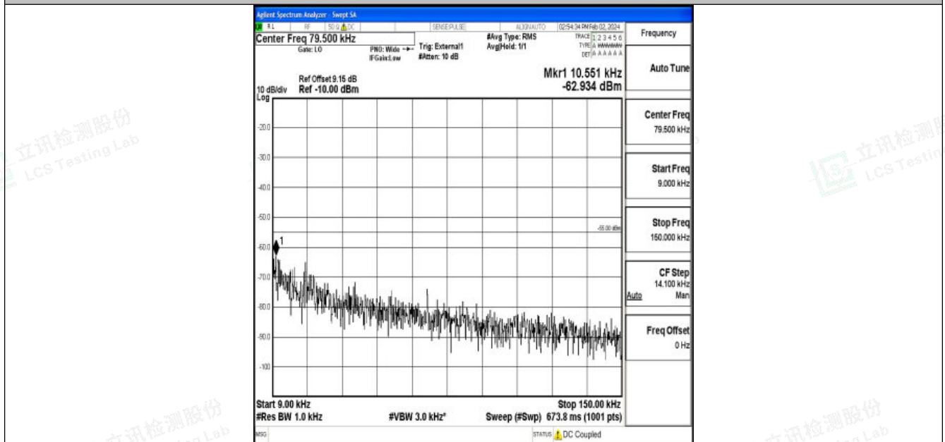
Band41_10MHz_16QAM_41540_1RB#0_0.009~0.15_0.009~0.15
