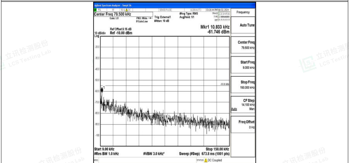
Band41_15MHz_16QAM_41515_1RB#0_0.009~0.15_0.009~0.15
