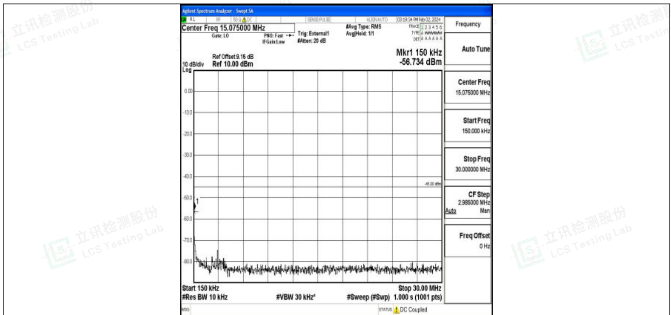
Band41_15MHz_16QAM_39725_1RB#0_0.15~30_0.15~30
