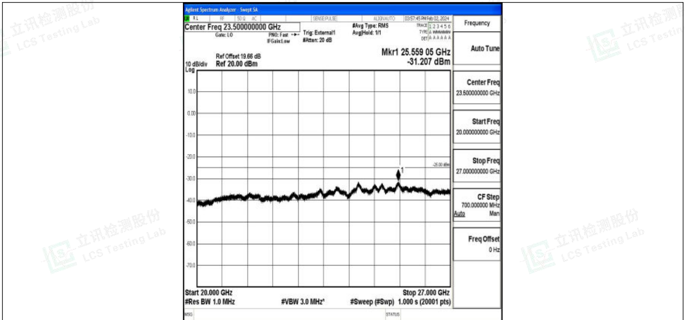
Band41_20MHz_QPSK_41490_1RB#0_20000~27000_20000~27000
