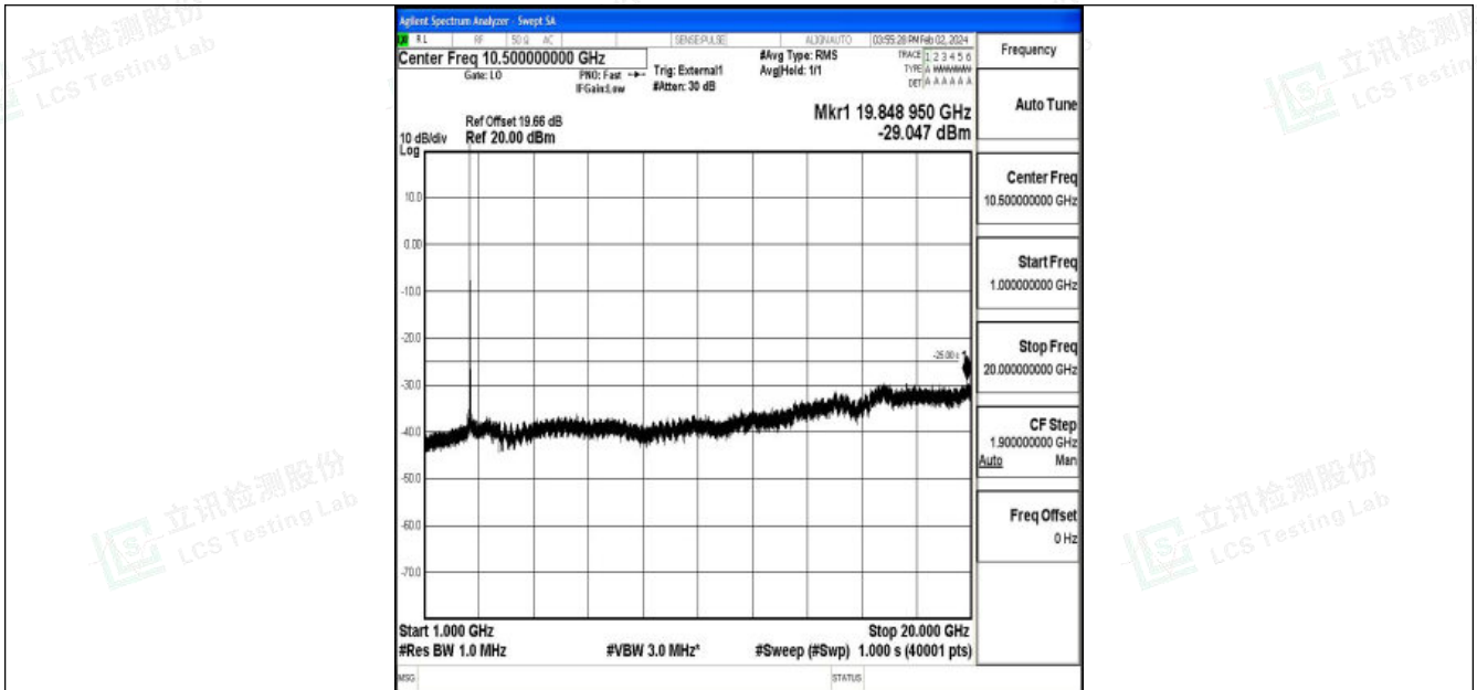
Band41_20MHz_16QAM_40620_1RB#0_1000~20000_1000~20000
