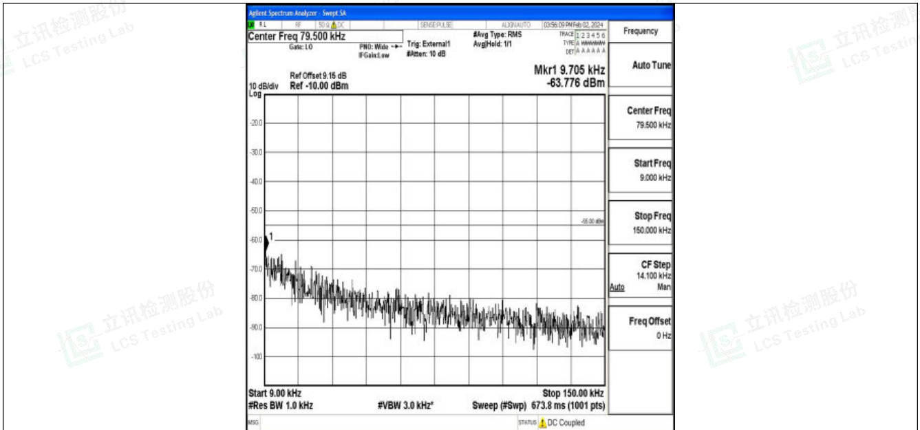
Band41_20MHz_QPSK_41490_1RB#0_0.009~0.15_0.009~0.15
