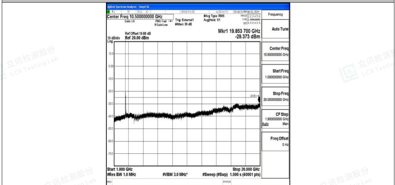
Band41_15MHz_QPSK_39725_1RB#0_1000~20000_1000~20000
