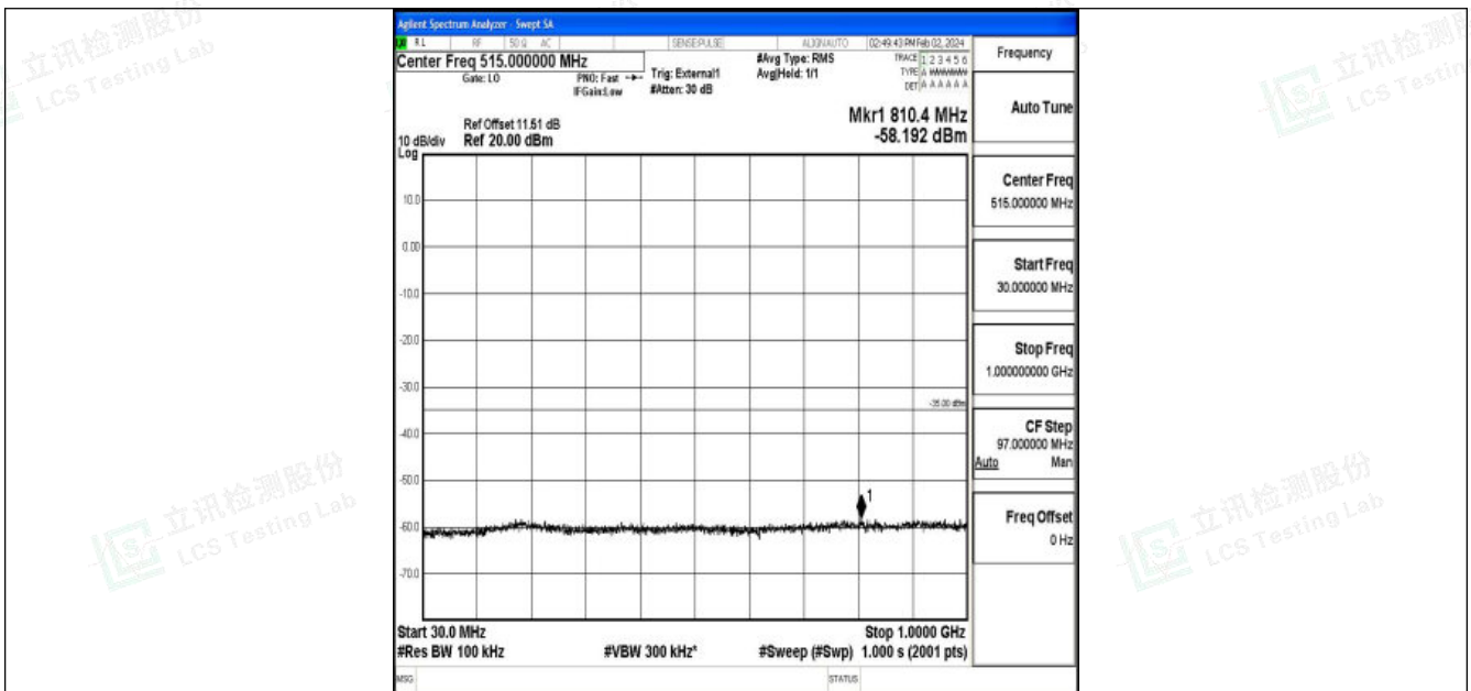
Band41_10MHz_QPSK_40620_1RB#0_30~1000_30~1000
