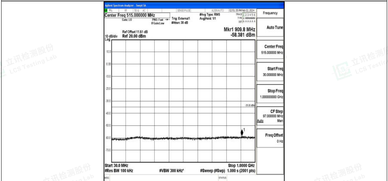
Band41_10MHz_16QAM_40620_1RB#0_30~1000_30~1000
