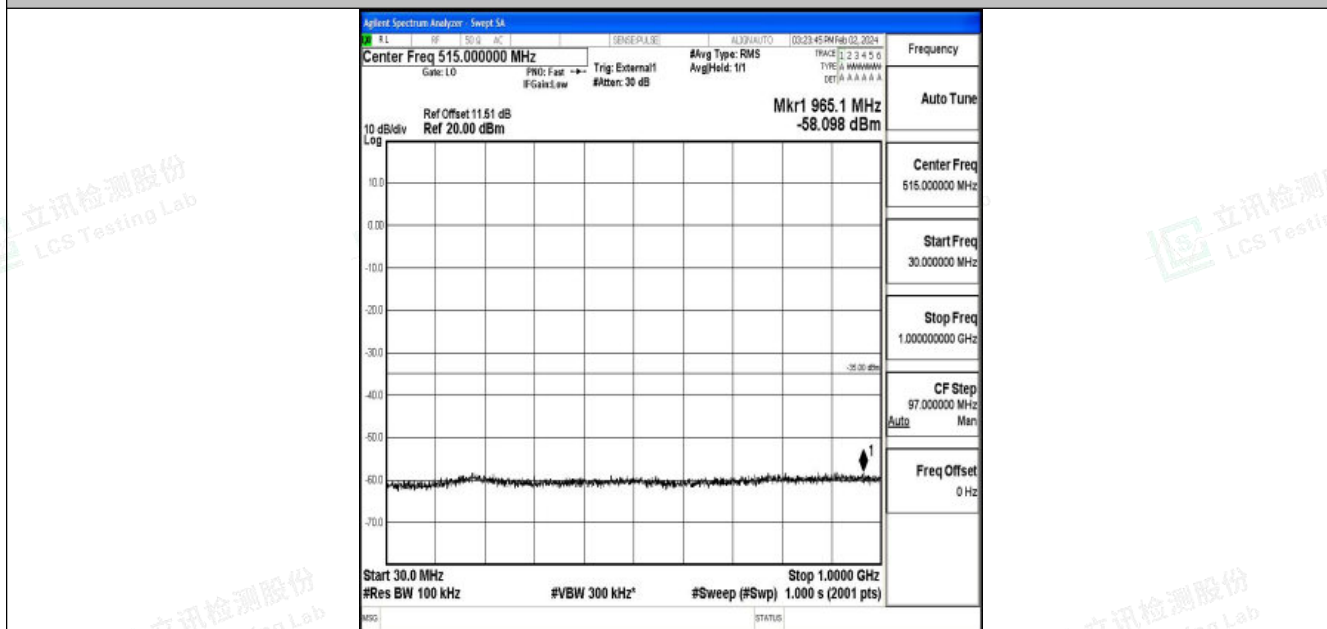
Band41_15MHz_16QAM_40620_1RB#0_30~1000_30~1000
