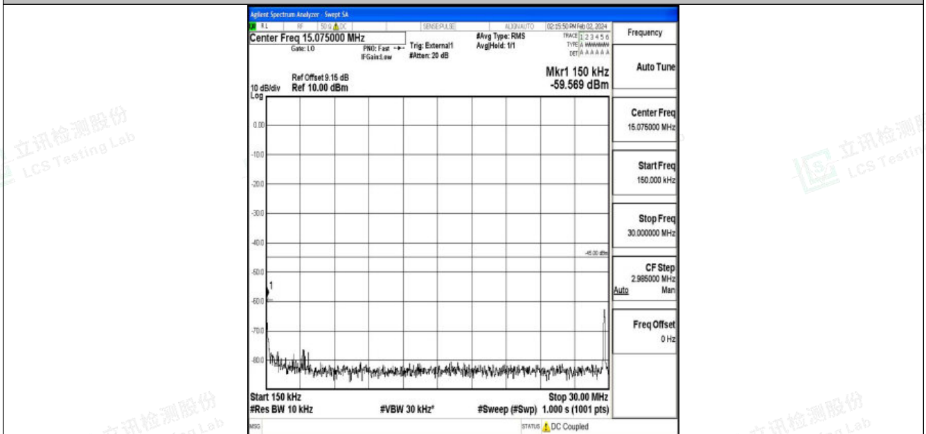
Band41_5MHz_QPSK_40620_1RB#0_0.15~30_0.15~30
