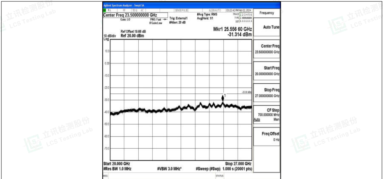
Band41_15MHz_QPSK_40620_1RB#0_20000~27000_20000~27000
