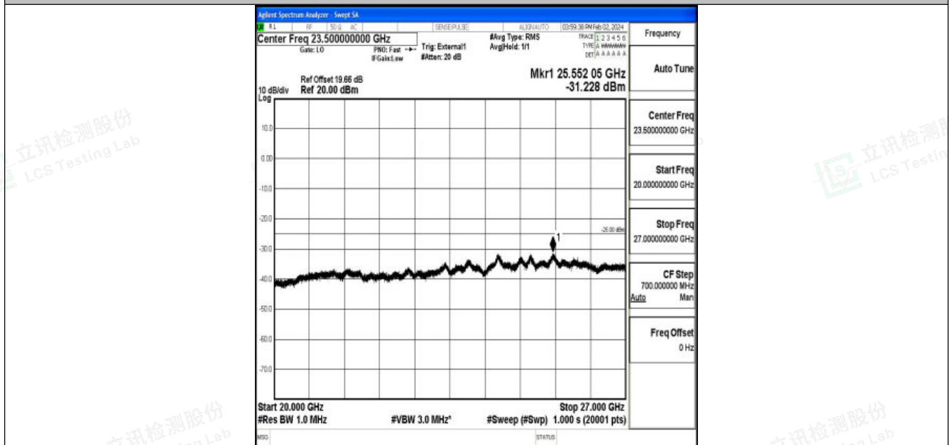
Band41_20MHz_16QAM_41490_1RB#0_20000~27000_20000~27000
