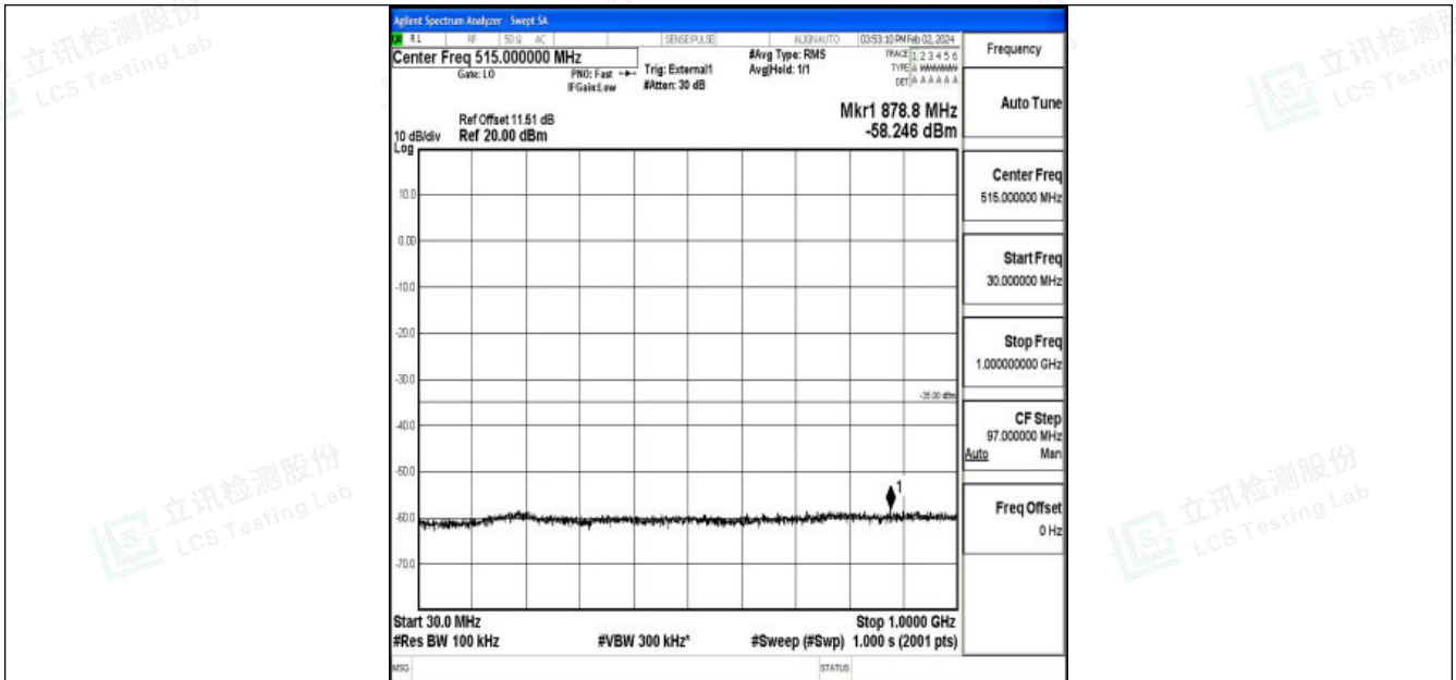
Band41_20MHz_QPSK_40620_1RB#0_30~1000_30~1000
