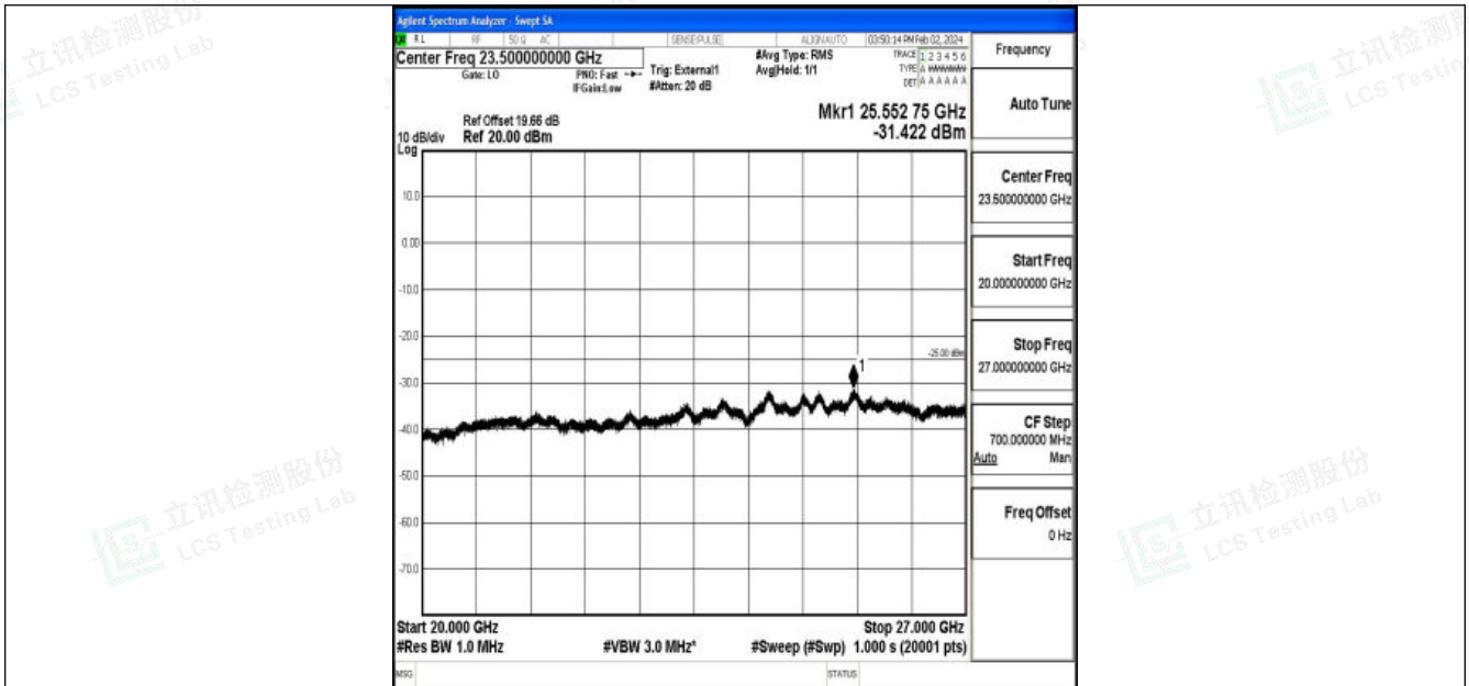
Band41_20MHz_QPSK_39750_1RB#0_20000~27000_20000~27000
