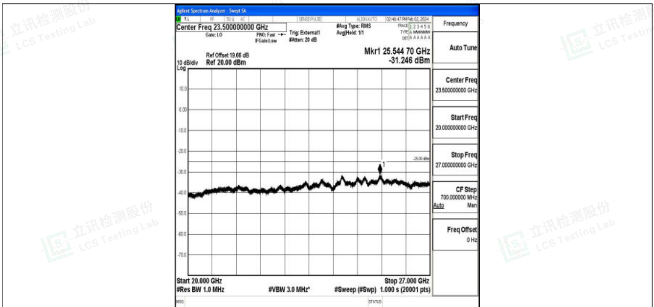
Band41_10MHz_QPSK_39700_1RB#0_20000~27000_20000~27000
