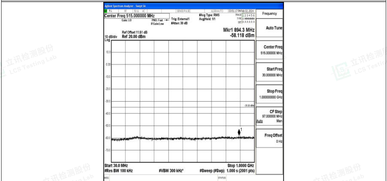
Band41_20MHz_16QAM_39750_1RB#0_30~1000_30~1000
