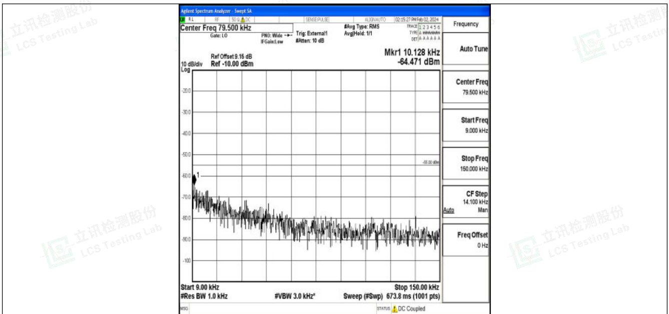
Band41_5MHz_QPSK_40620_1RB#0_0.009~0.15_0.009~0.15
