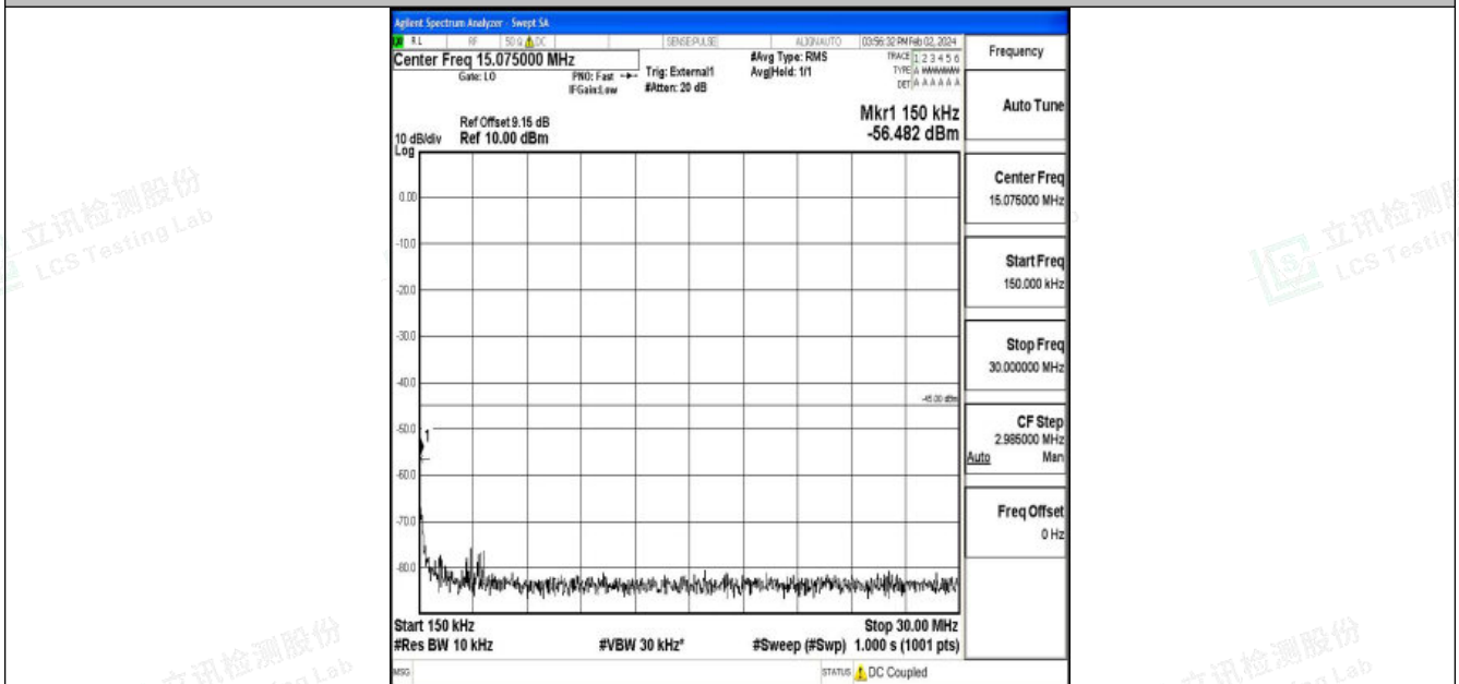
Band41_20MHz_QPSK_41490_1RB#0_0.15~30_0.15~30
