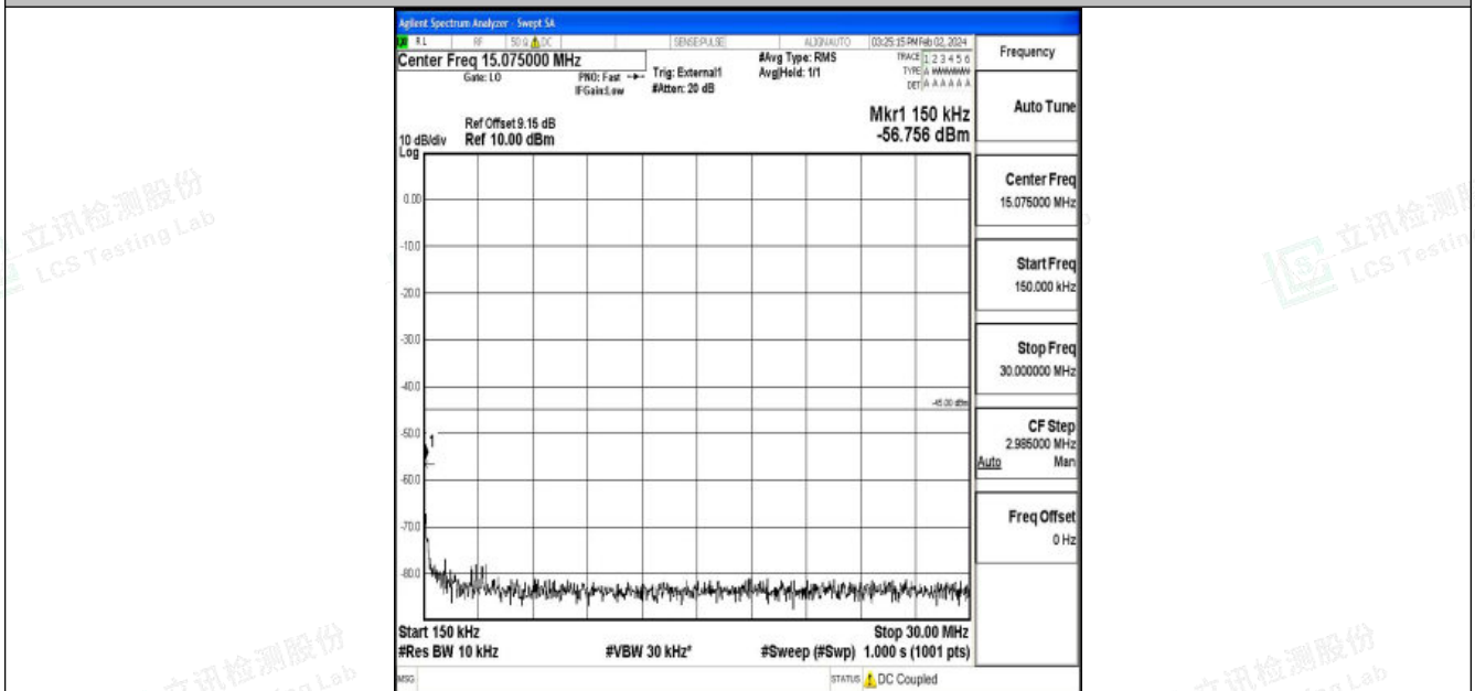
Band41_15MHz_QPSK_41515_1RB#0_0.15~30_0.15~30
