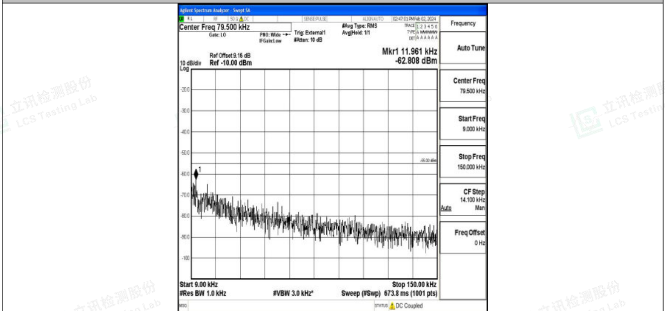
Band41_10MHz_16QAM_39700_1RB#0_0.009~0.15_0.009~0.15
