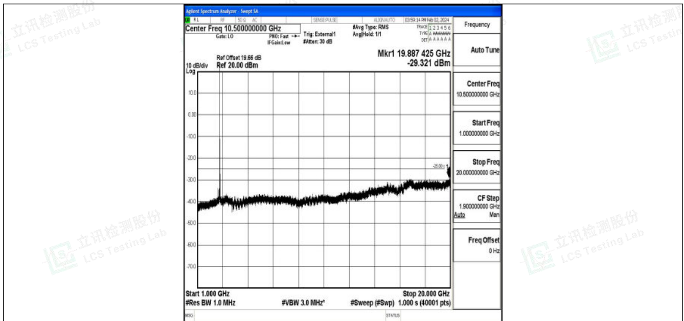
Band41_20MHz_16QAM_41490_1RB#0_1000~20000_1000~20000
