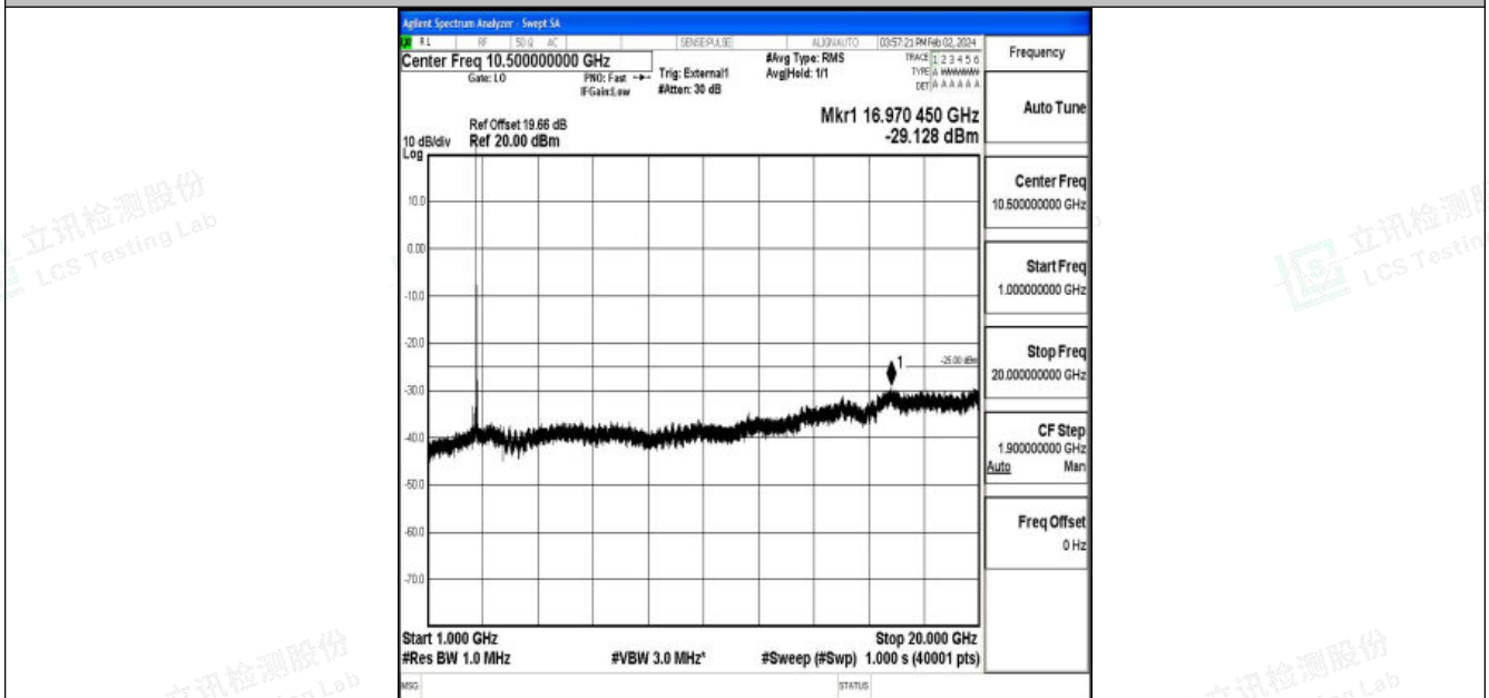
Band41_20MHz_QPSK_41490_1RB#0_1000~20000_1000~20000
