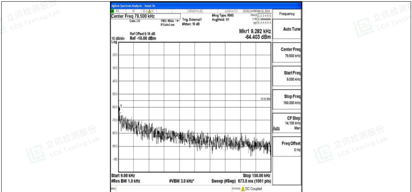
Band41_20MHz_QPSK_40620_1RB#0_0.009~0.15_0.009~0.15
