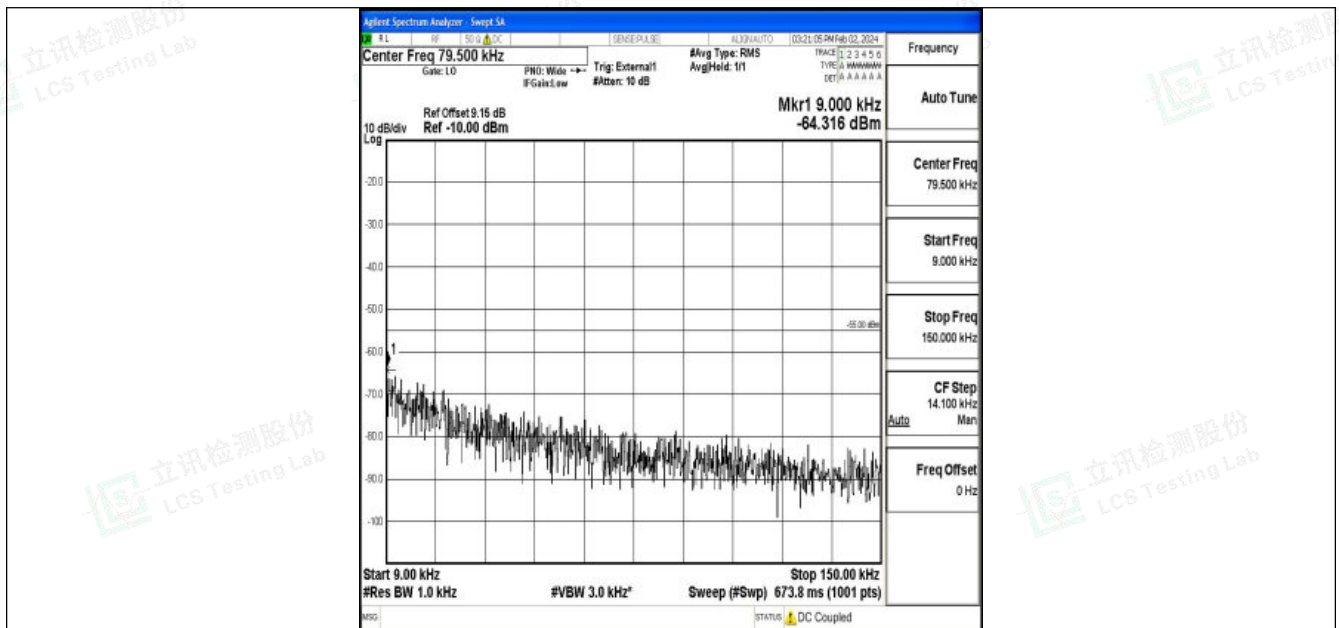
Band41_15MHz_QPSK_40620_1RB#0_0.009~0.15_0.009~0.15
