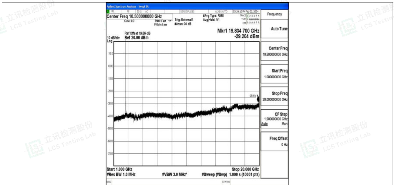
Band41_15MHz_16QAM_40620_1RB#0_1000~20000_1000~20000
