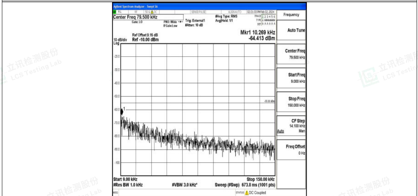
Band41_5MHz_16QAM_41565_1RB#0_0.009~0.15_0.009~0.15
