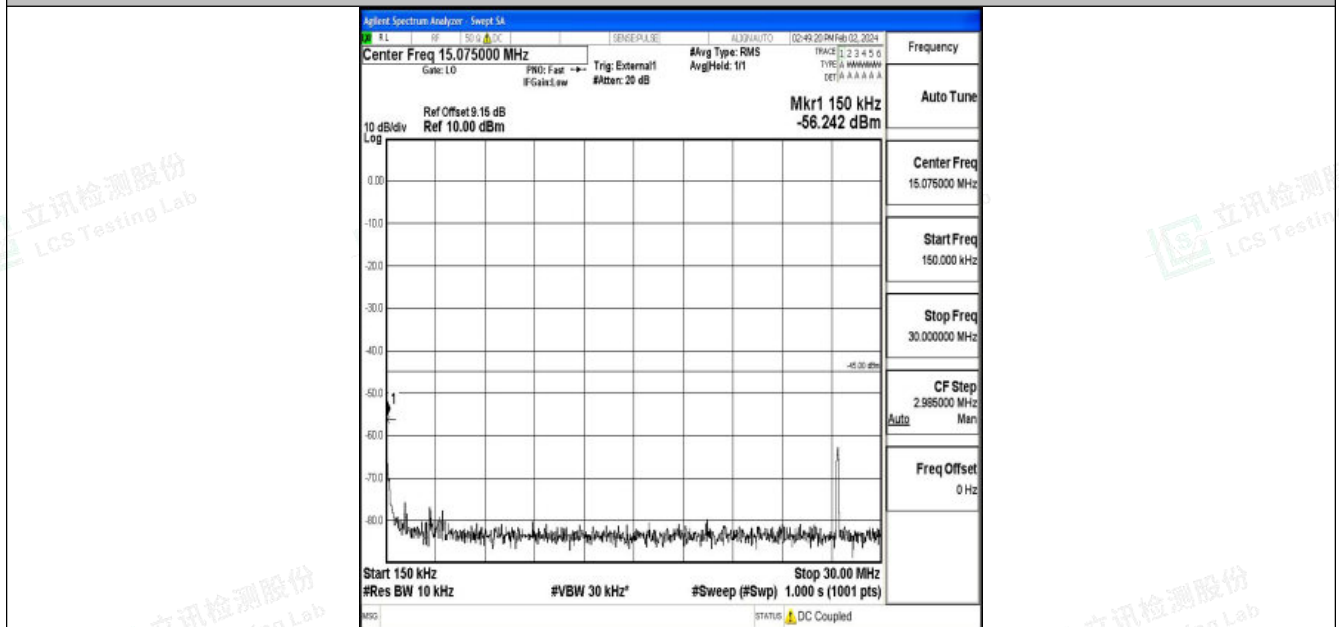
Band41_10MHz_QPSK_40620_1RB#0_0.15~30_0.15~30
