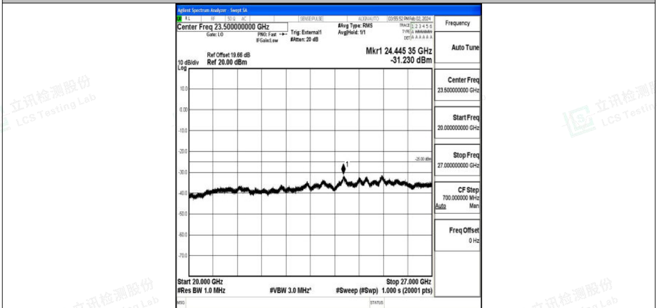
Band41_20MHz_16QAM_40620_1RB#0_20000~27000_20000~27000
