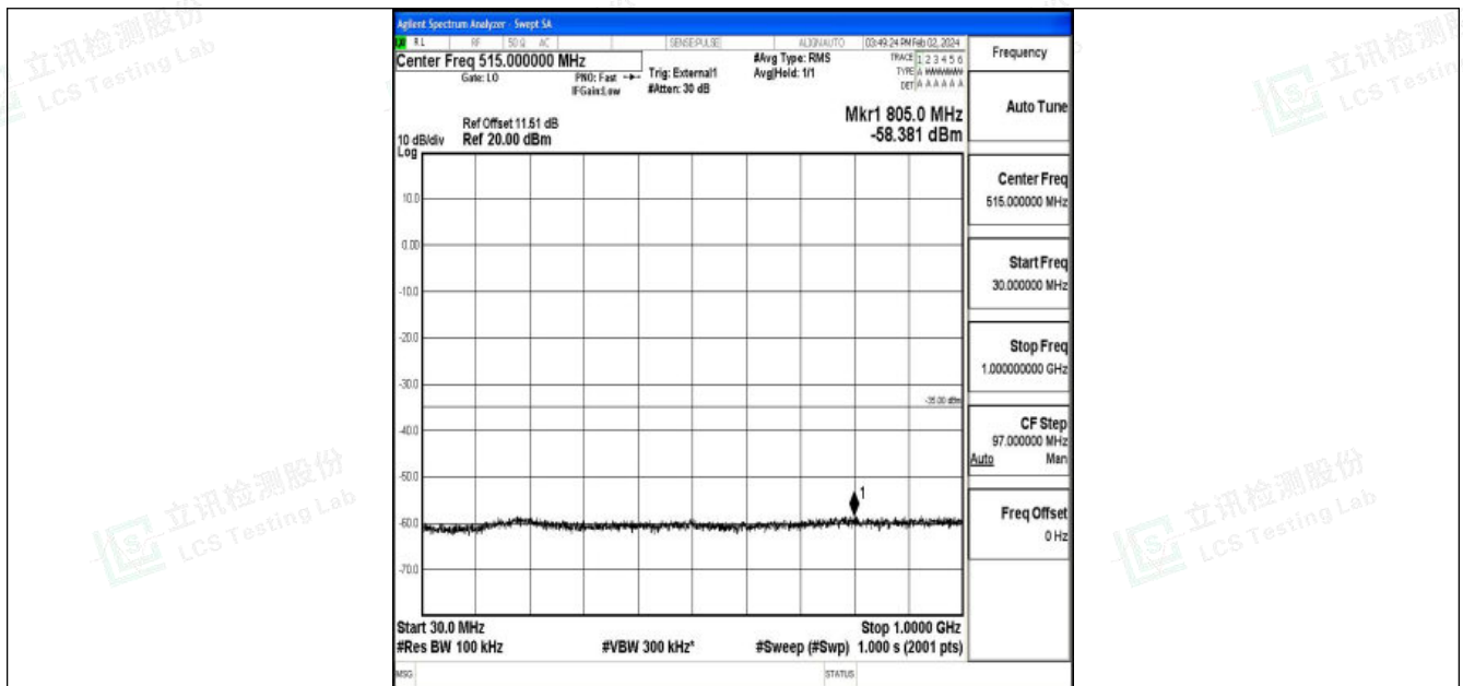
Band41_20MHz_QPSK_39750_1RB#0_30~1000_30~1000
