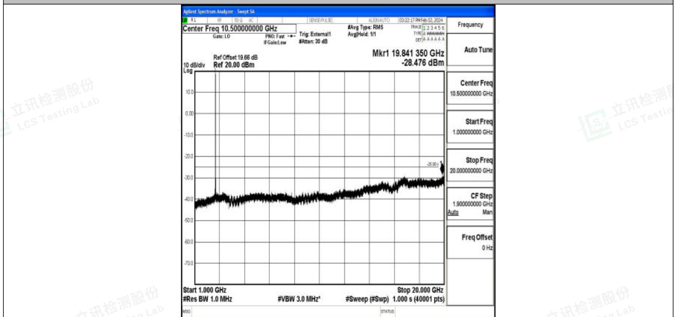
Band41_15MHz_QPSK_40620_1RB#0_1000~20000_1000~20000
