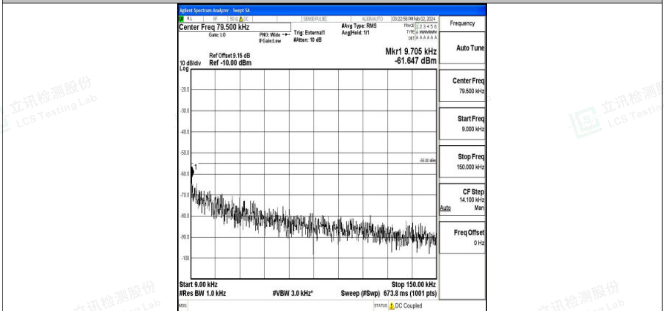
Band41_15MHz_16QAM_40620_1RB#0_0.009~0.15_0.009~0.15
