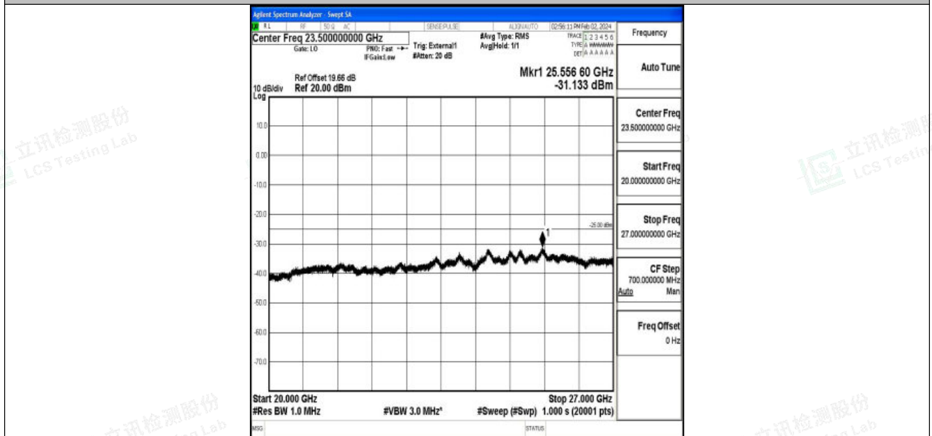
Band41_10MHz_16QAM_41540_1RB#0_20000~27000_20000~27000
