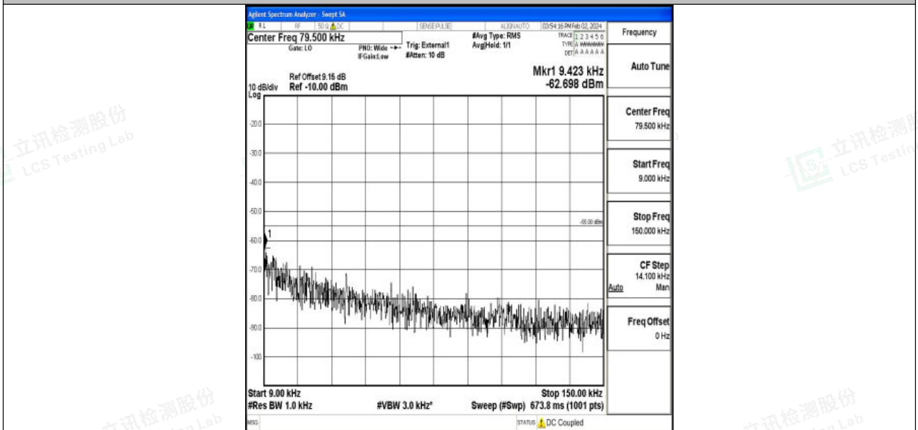
Band41_20MHz_16QAM_40620_1RB#0_0.009~0.15_0.009~0.15
