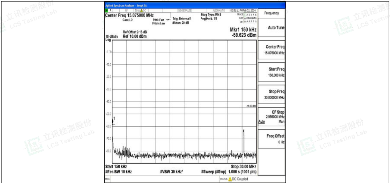
Band41_10MHz_16QAM_40620_1RB#0_0.15~30_0.15~30
