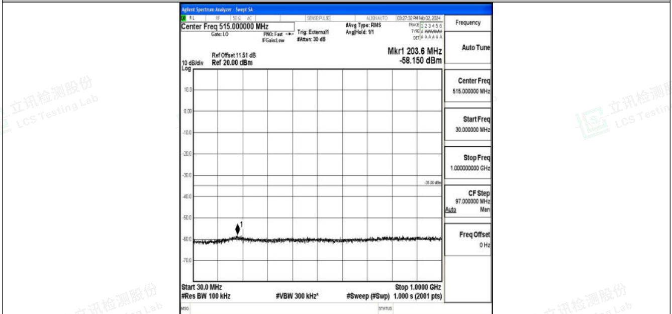
Band41_15MHz_16QAM_41515_1RB#0_30~1000_30~1000
