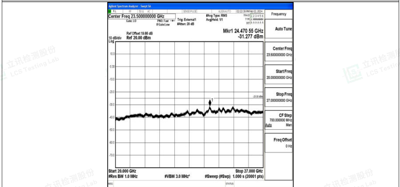
Band41_5MHz_16QAM_41565_1RB#0_20000~27000_20000~27000
