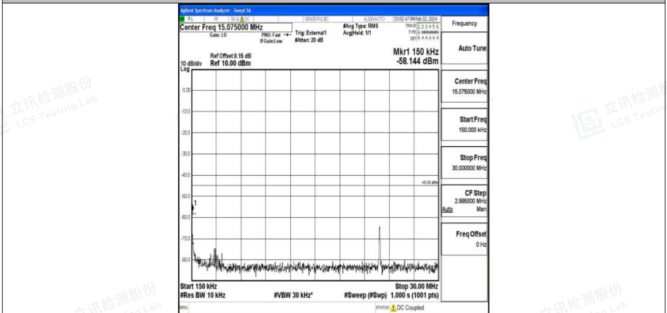
Band41_20MHz_QPSK_40620_1RB#0_0.15~30_0.15~30
