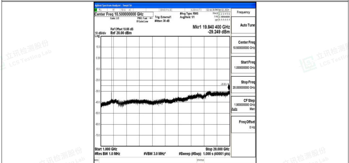
Band41_5MHz_QPSK_40620_1RB#0_1000~20000_1000~20000
