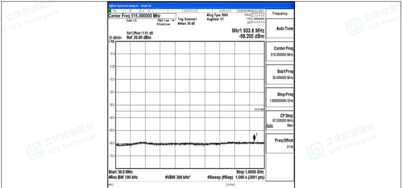
Band41_20MHz_QPSK_41490_1RB#0_30~1000_30~1000
