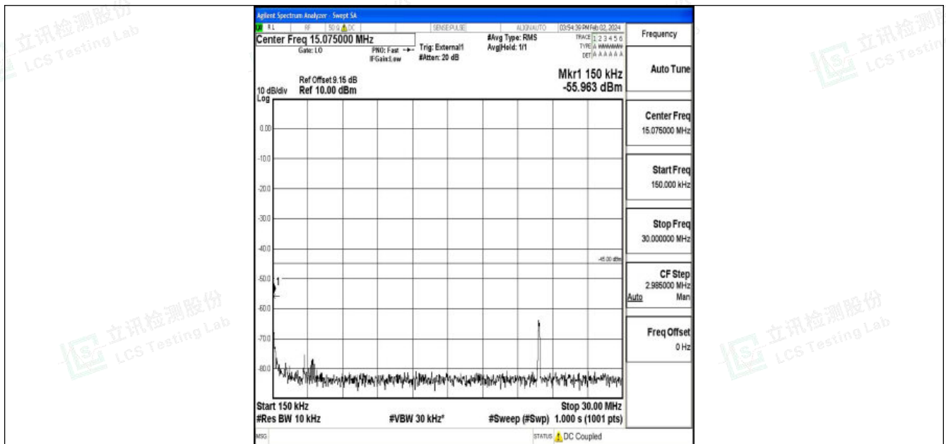
Band41_20MHz_16QAM_40620_1RB#0_0.15~30_0.15~30
