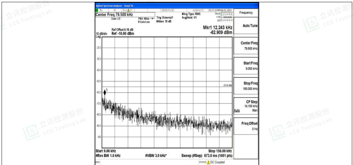
Band41_15MHz_QPSK_39725_1RB#0_0.009~0.15_0.009~0.15
