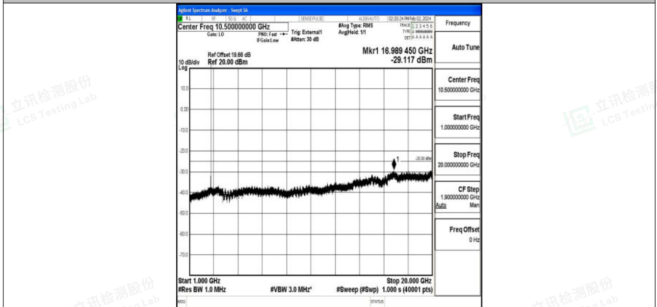
Band41_5MHz_QPSK_41565_1RB#0_1000~20000_1000~20000
