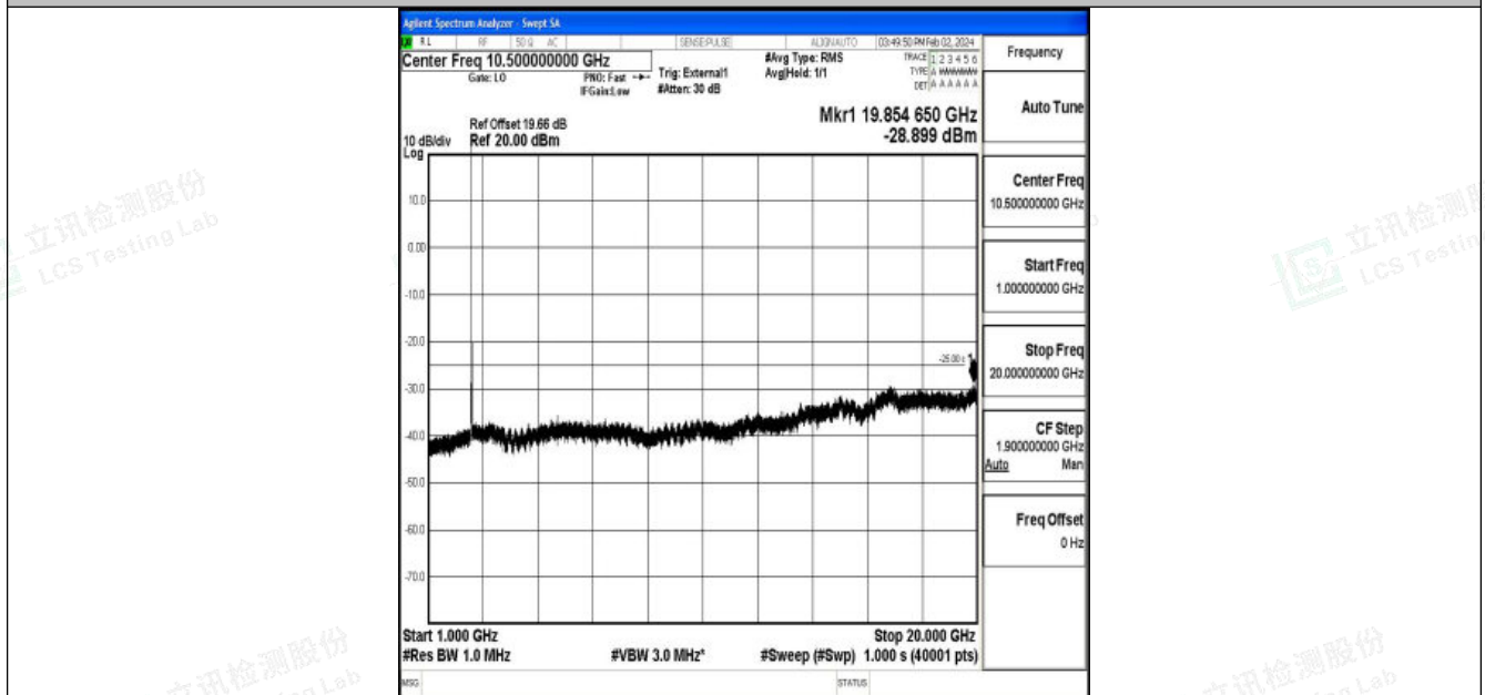
Band41_20MHz_QPSK_39750_1RB#0_1000~20000_1000~20000
