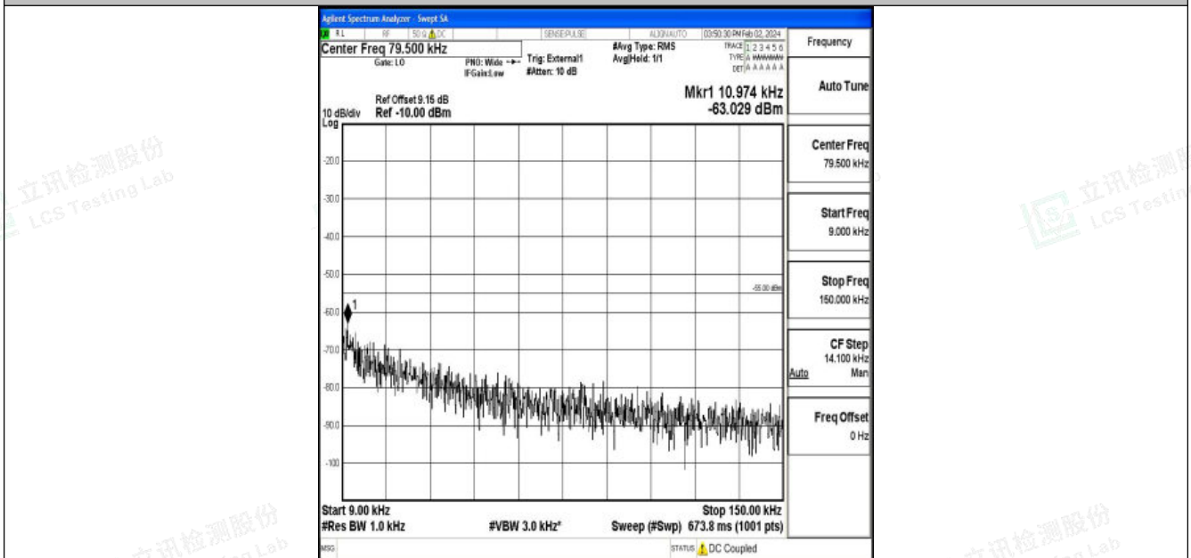
Band41_20MHz_16QAM_39750_1RB#0_0.009~0.15_0.009~0.15
