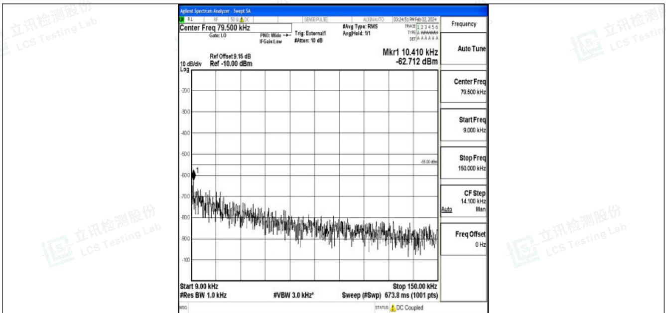
Band41_15MHz_QPSK_41515_1RB#0_0.009~0.15_0.009~0.15
