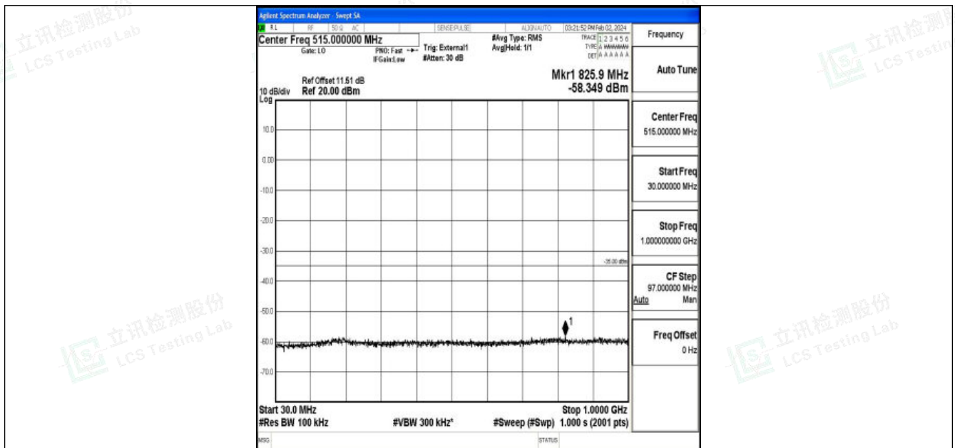
Band41_15MHz_QPSK_40620_1RB#0_30~1000_30~1000
