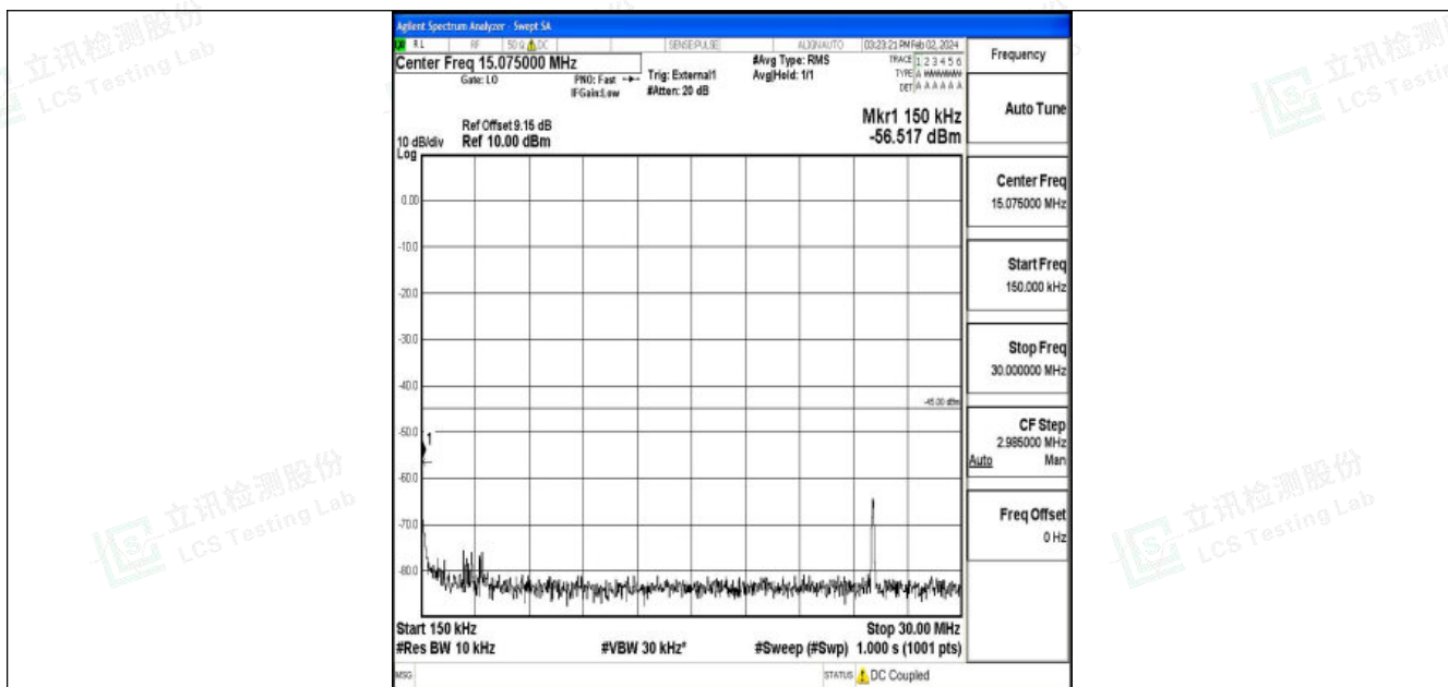
Band41_15MHz_16QAM_40620_1RB#0_0.15~30_0.15~30
