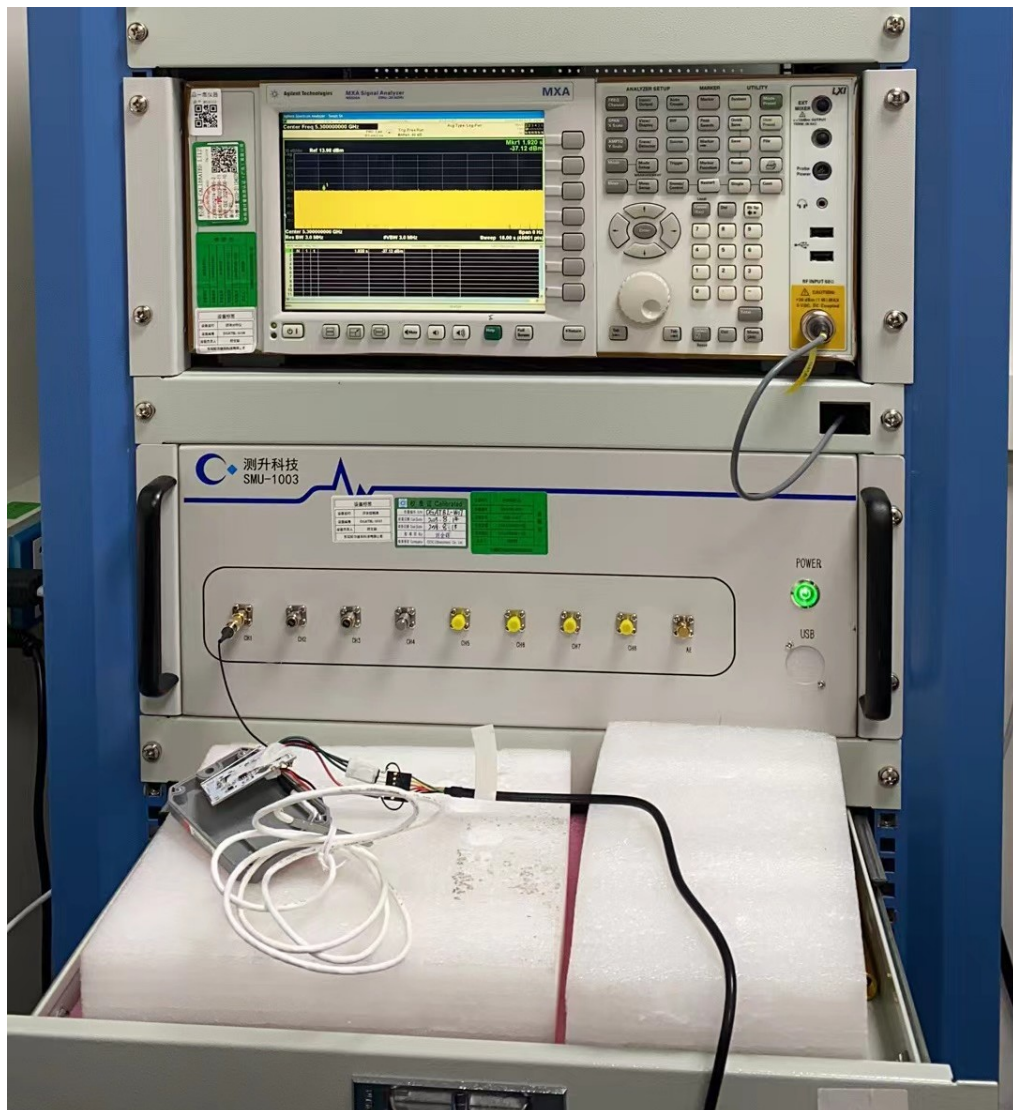
Photograph 3: Set-up for Conducted Test
