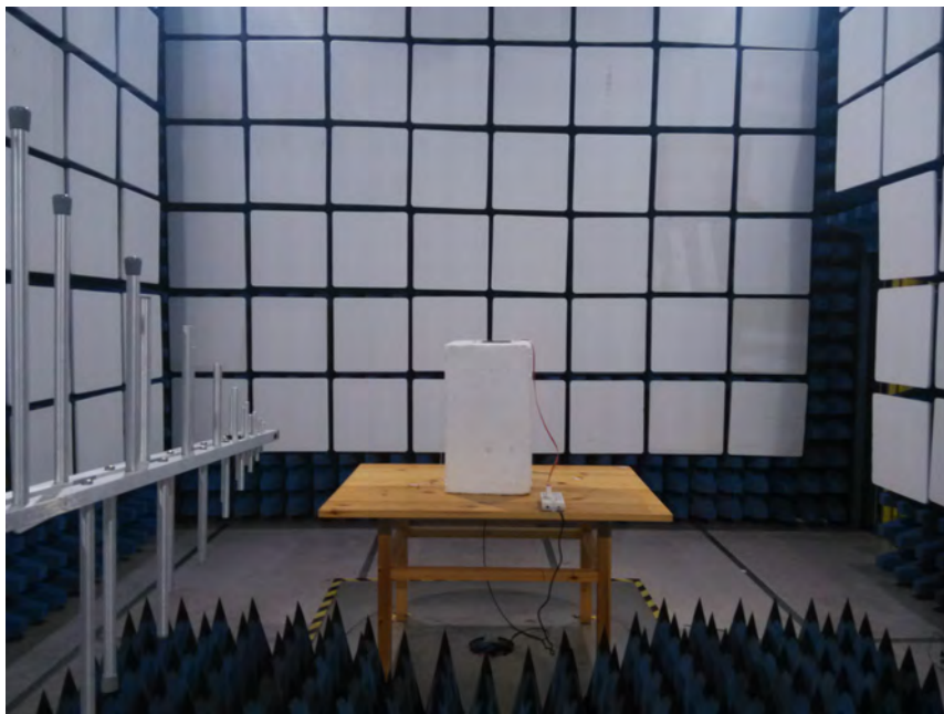
30 MHz-1 GHz
