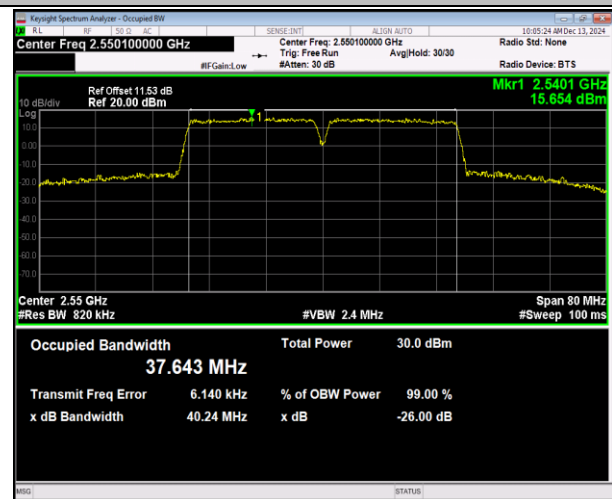
7-7-20MHz-20MHz-16QAM-16QAM-21152-21350-100RB# 0-100RB#0-PASS
