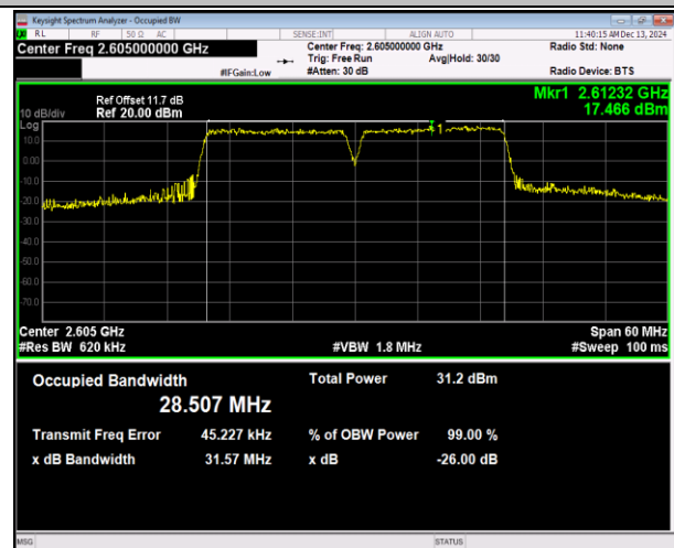
38-38-15MHz-15MHz-16QAM-16QAM-38025-38175-75RB #0-75RB#0-PASS
