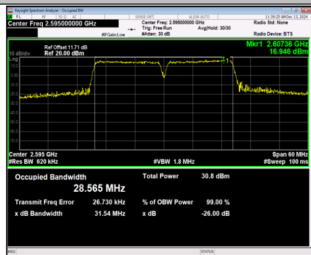
38-38-15MHz-15MHz-16QAM-16QAM-37925-38075-75RB #0-75RB#0-PASS
