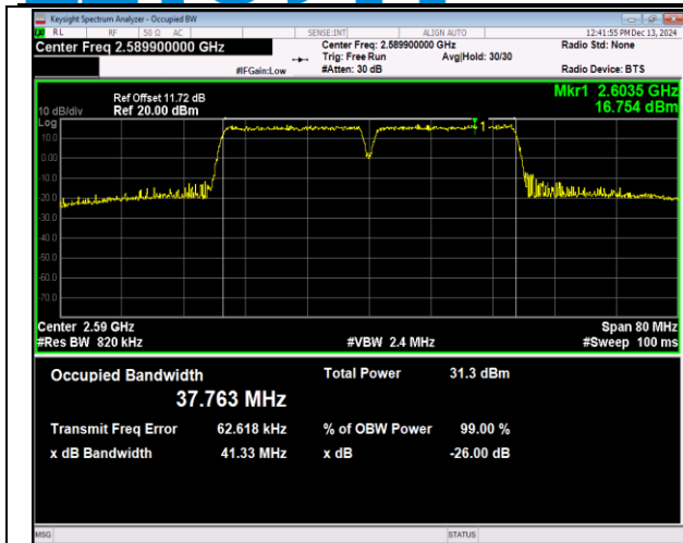
38-38-20MHz-20MHz-QPSK-QPSK-37850-38048-100RB #0-100RB#0-PASS
