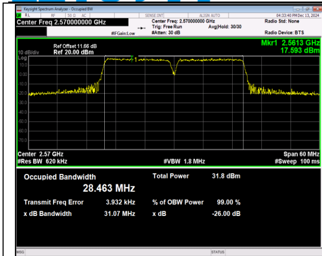
41(2555-2655)-41(2555-2655)-15MHz-15MHz-QPSK-QP SK-40315-40465-75RB#0-75RB#0-PASS
