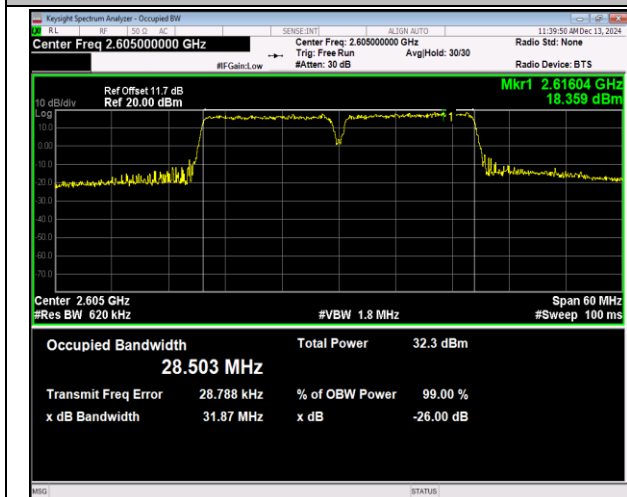
38-38-15MHz-15MHz-QPSK-QPSK-38025-38175-75RB# 0-75RB#0-PASS
