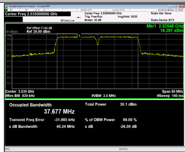
7-7-20MHz-20MHz-16QAM-16QAM-21001-21199-100RB# 0-100RB#0-PASS
