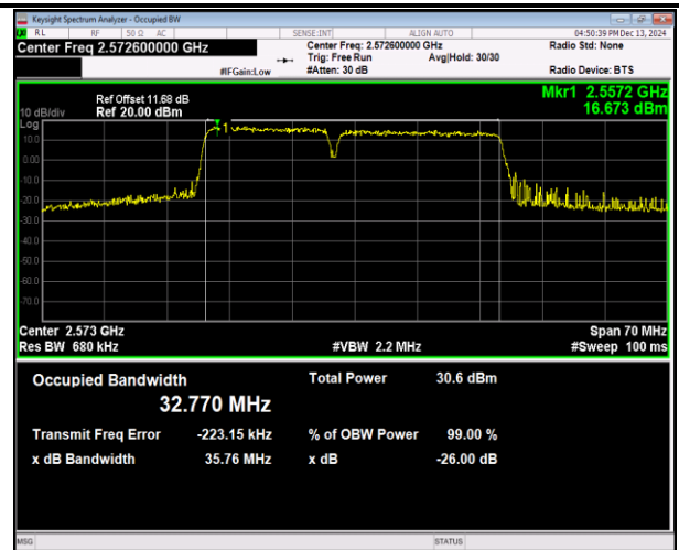
41(2555-2655)-41(2555-2655)-15MHz-20MHz-16QAM-16Q AM-40318-40489-75RB#0-100RB#0-PASS
