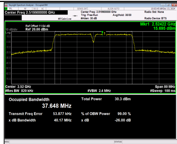
7-7-20MHz-20MHz-16QAM-16QAM-20850-21048-100RB# 0-100RB#0-PASS
