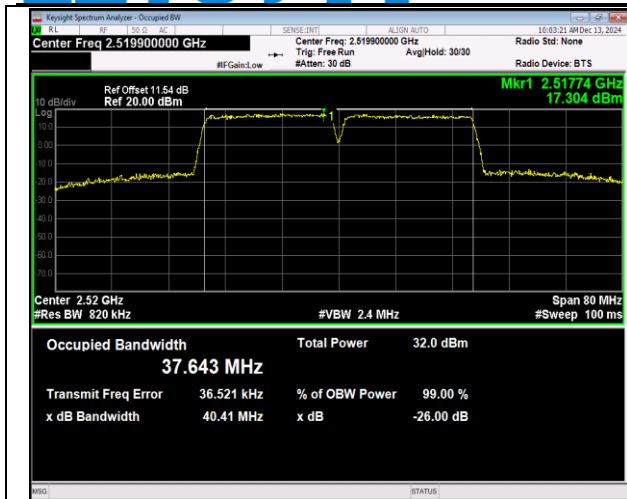
7-7-20MHz-20MHz-QPSK-QPSK-20850-21048-100RB#0- 100RB#0-PASS
