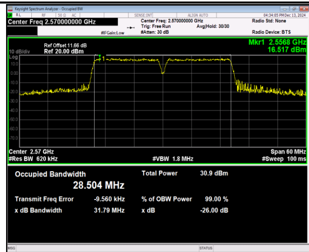
41(2555-2655)-41(2555-2655)-15MHz-15MHz-16QAM-16Q AM-40315-40465-75RB#0-75RB#0-PASS
