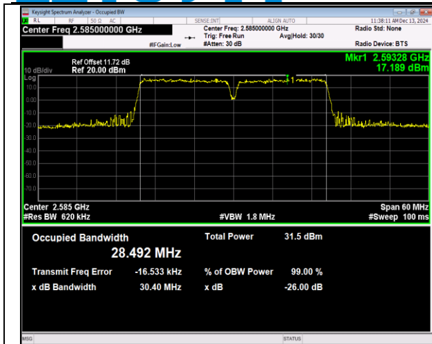
38-38-15MHz-15MHz-QPSK-QPSK-37825-37975-75RB# 0-75RB#0-PASS
