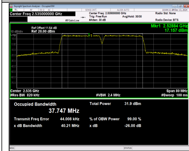
7-7-20MHz-20MHz-QPSK-QPSK-21001-21199-100RB#0- 100RB#0-PASS
