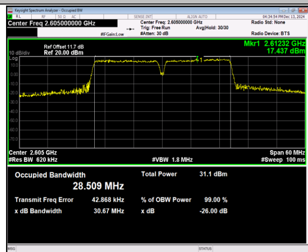
41(2555-2655)-41(2555-2655)-15MHz-15MHz-16QAM-16Q AM-40665-40815-75RB#0-75RB#0-PASS
