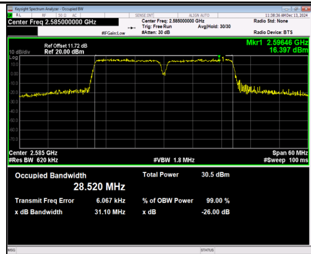
38-38-15MHz-15MHz-16QAM-16QAM-37825-37975-75RB #0-75RB#0-PASS
