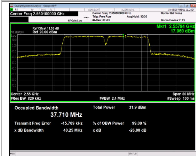
7-7-20MHz-20MHz-QPSK-QPSK-21152-21350-100RB#0- 100RB#0-PASS
