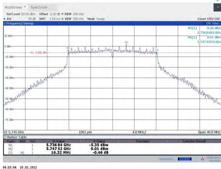
11a-CDD Ant3 5745
