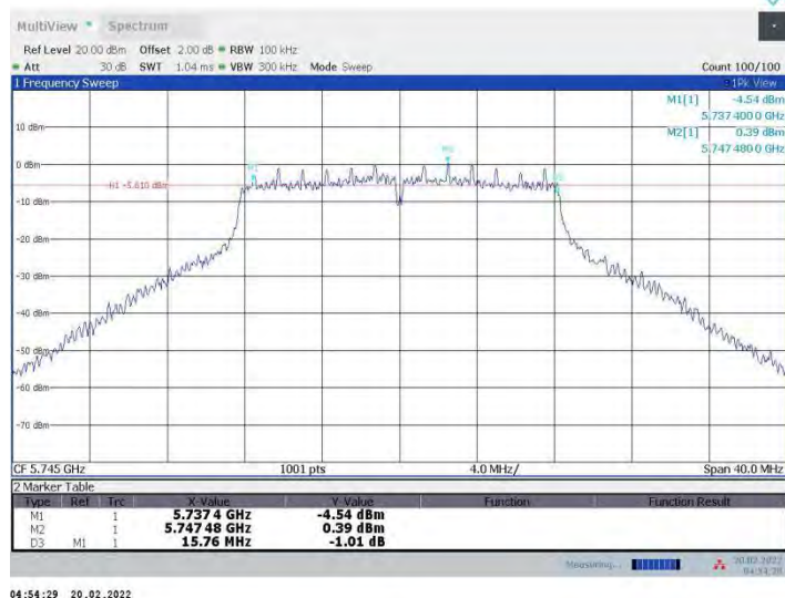
11a-CDD Ant2 5745
