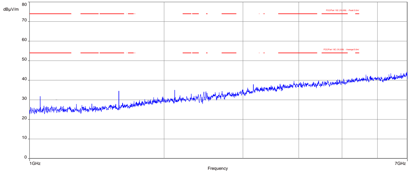
Plot 1: 1 GHz to 7 GHz, RX / idle – mode, vertical & horizontal polarization
