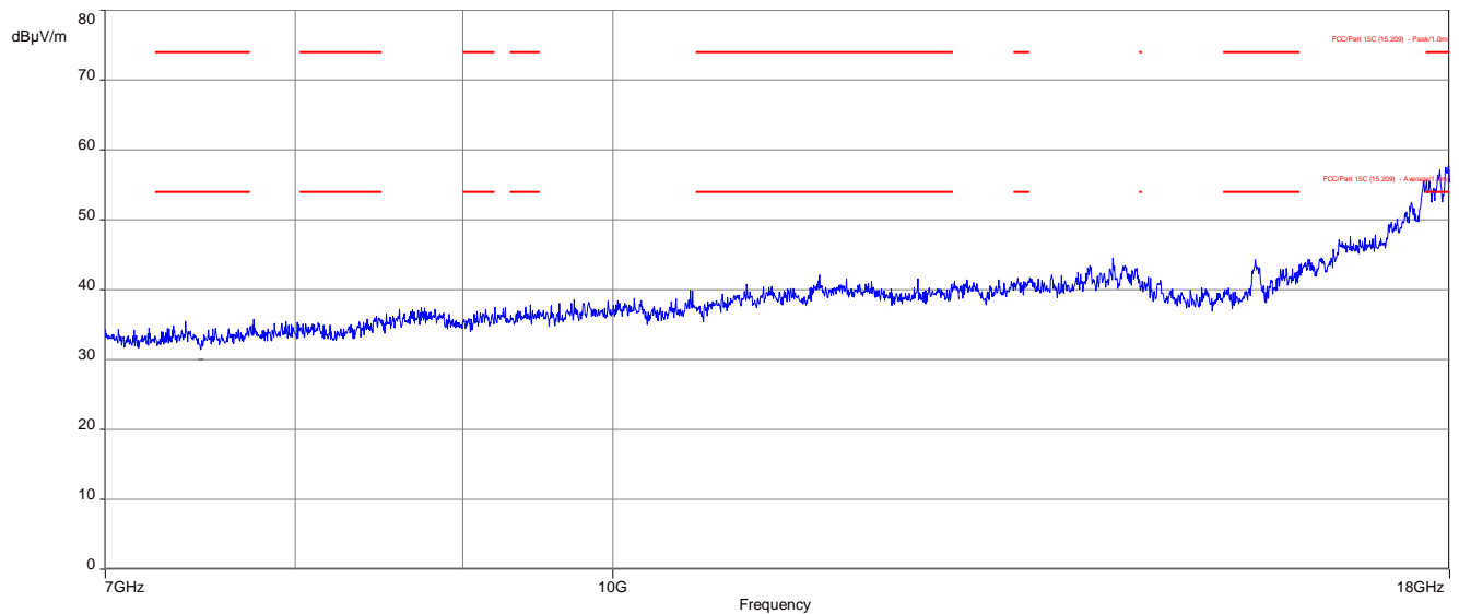
Plot 2: 7 GHz to 18 GHz, RX / idle – mode, vertical & horizontal polarization
