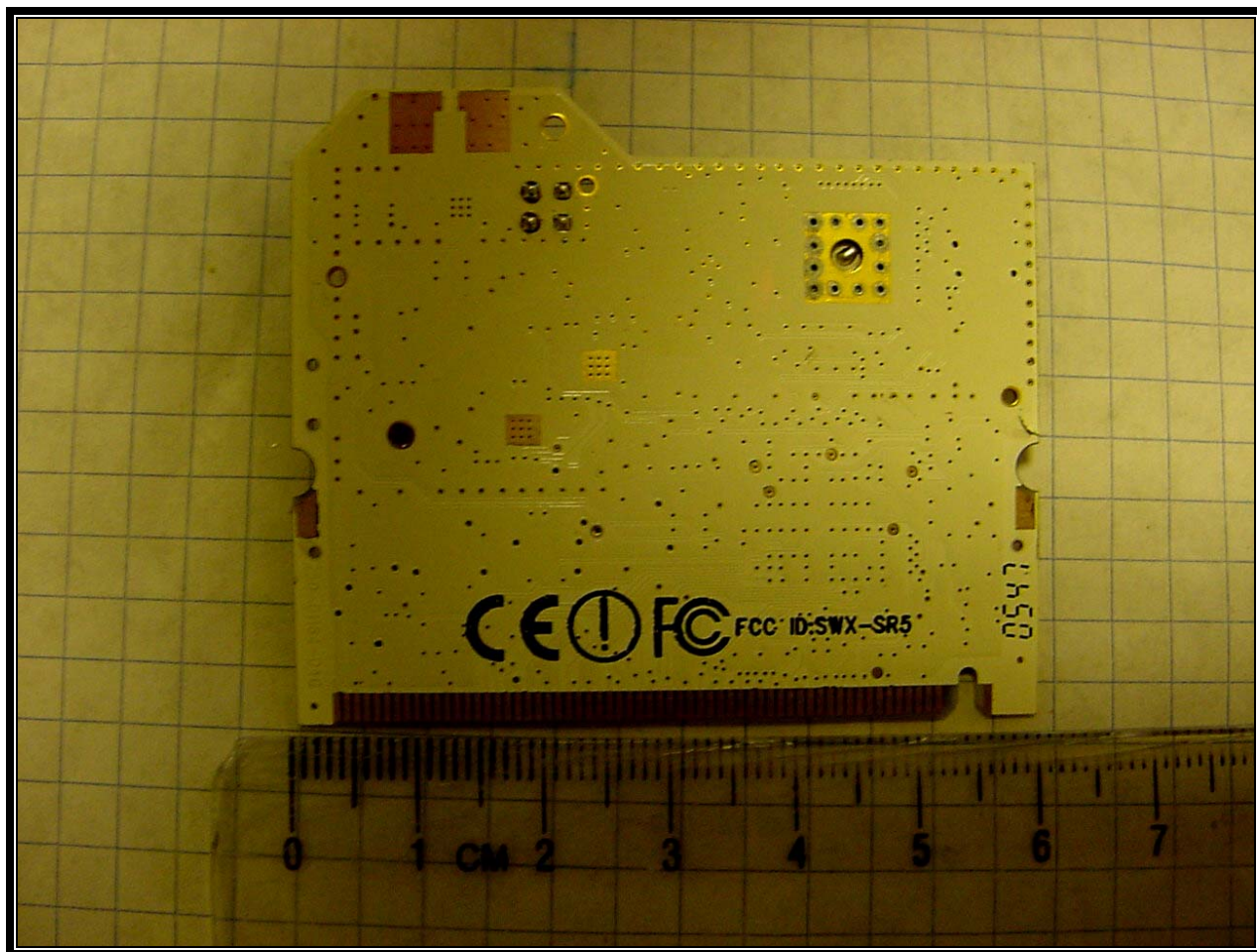
Photograph 20: 5.7 GHz Radio Bottom without Heat Sink
