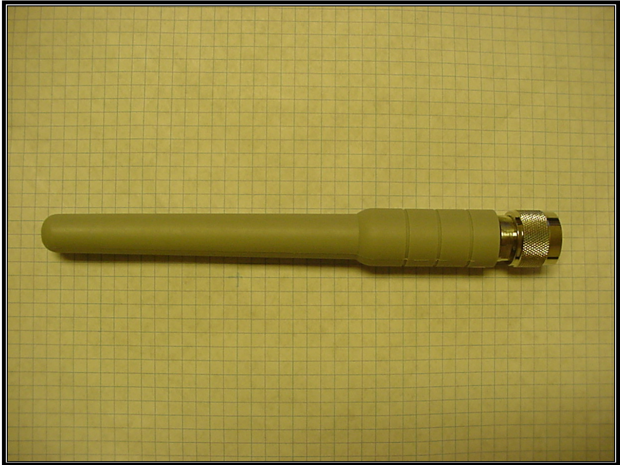
Photograph 25: 5.7 GHz Antenna
