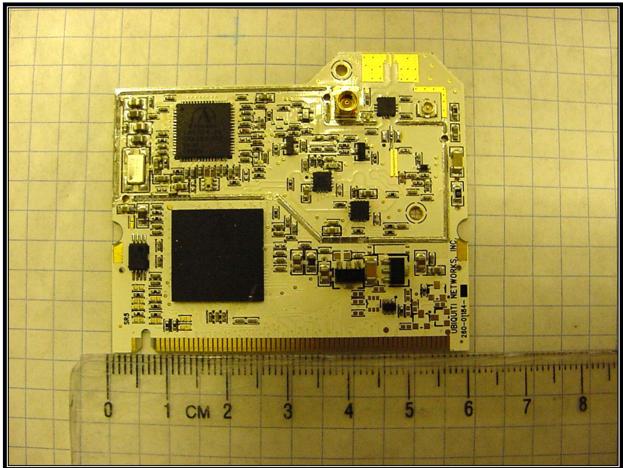
Photograph 18: 5.7 GHz Radio Top without Shield
