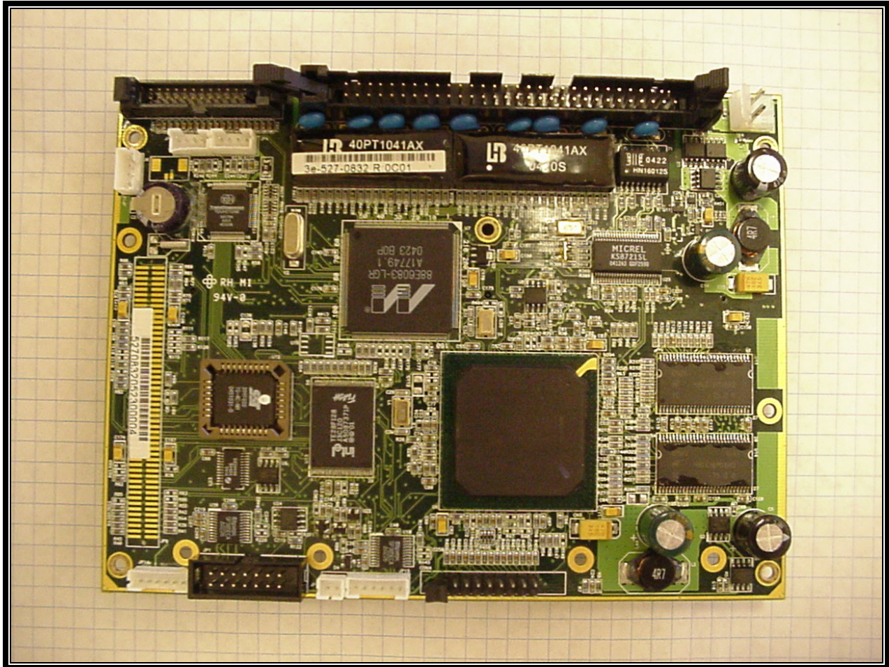
Photograph 10: Top of PCB
