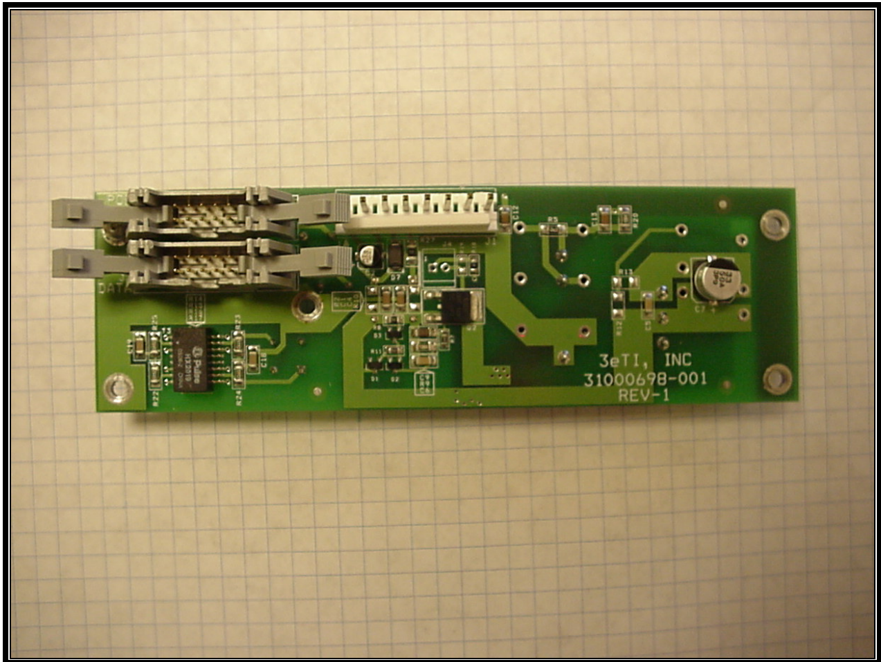
Photograph 14: Front of Power PCB
