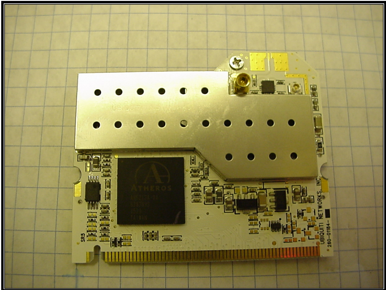
Photograph 17: 5.7 GHz Radio Top
