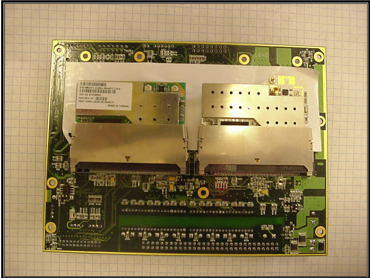
Photograph 11: Bottom of PCB with Radios and Shields
