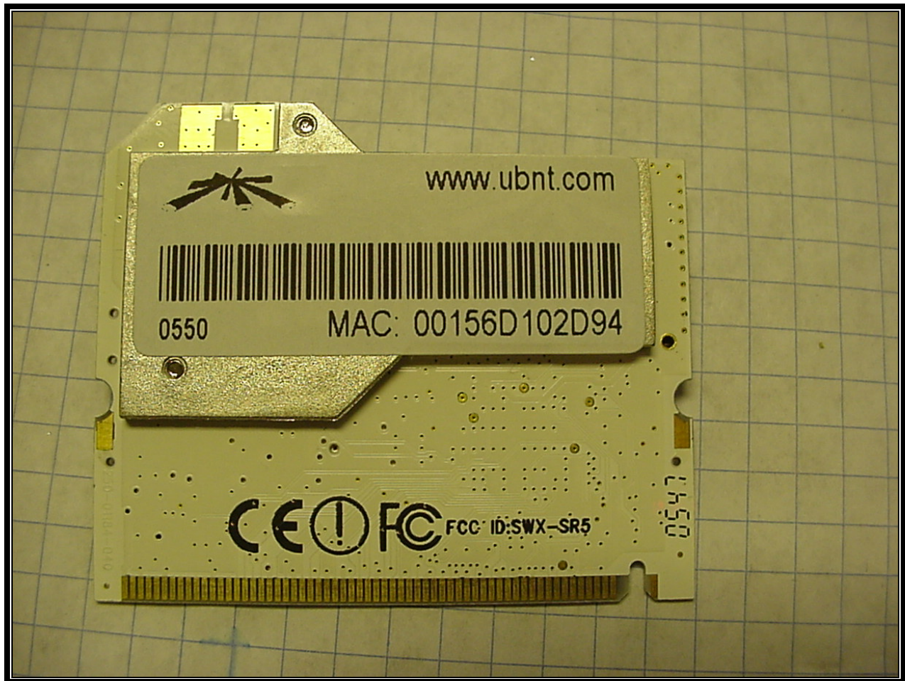
Photograph 19: 5.7 GHz Radio Bottom
