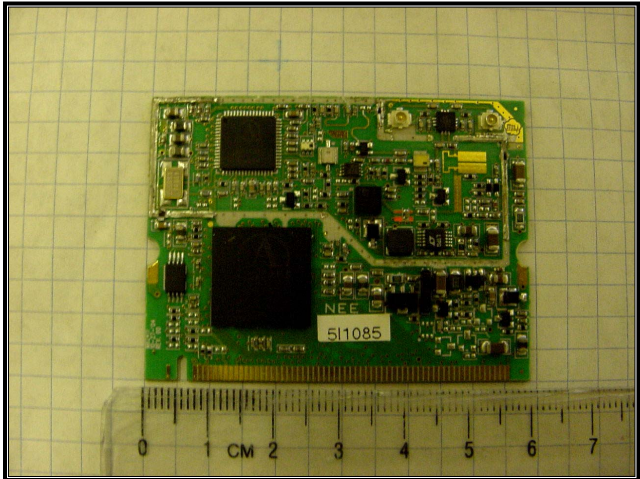
Photograph 22: 2.4 GHz Radio Top without Shield
