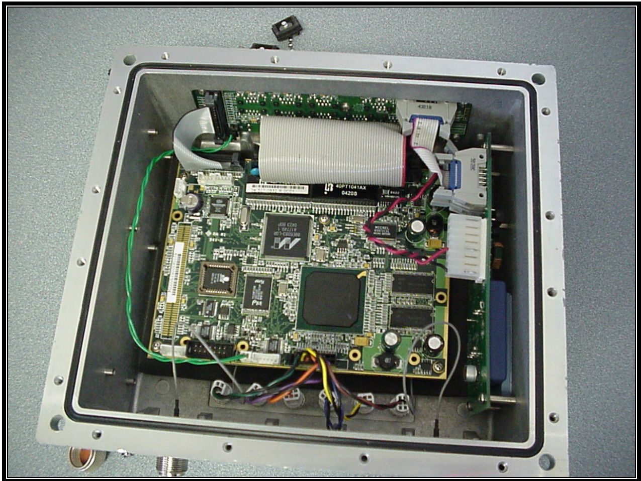
Photograph 9: Inside Bottom Removed
