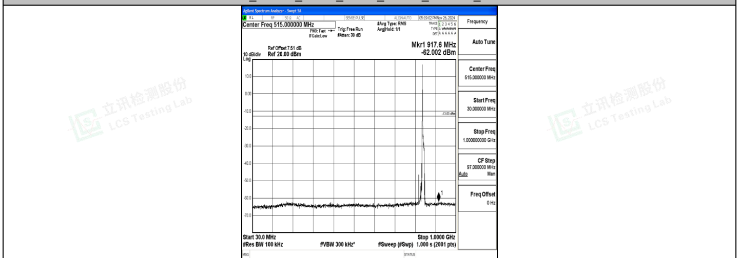
Band5_10MHz_QPSK_20600_1RB#0_30~1000_30~1000
