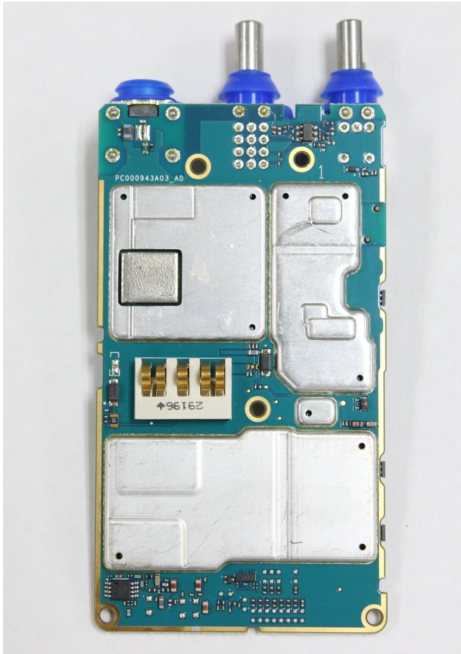
RF board with Shields (Bottom)
