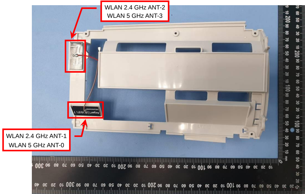
EUT Photo (28)
