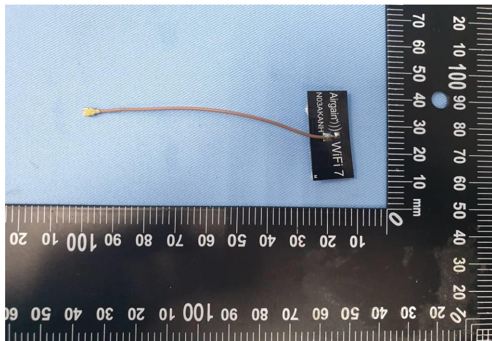
EUT Photo (28)
