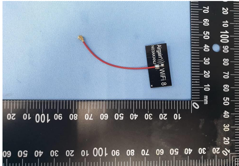
EUT Photo (32)
