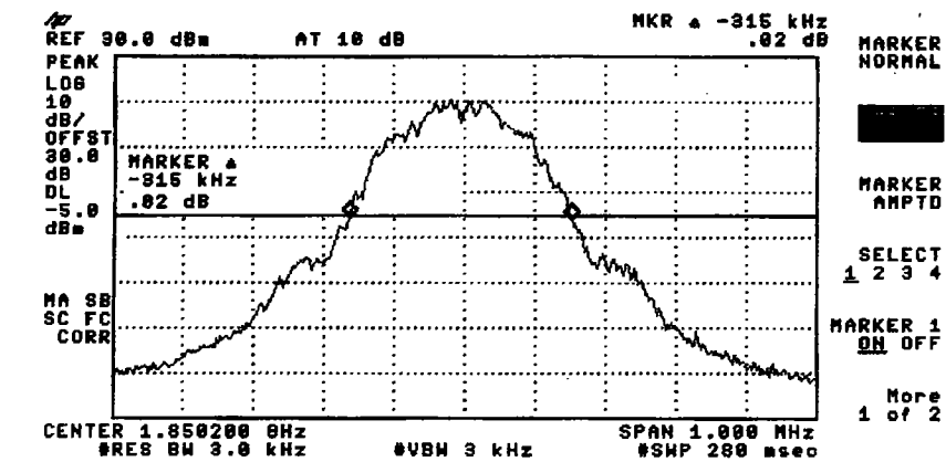
Fig.8.4: Channel 512, -26dB Bandwidth
