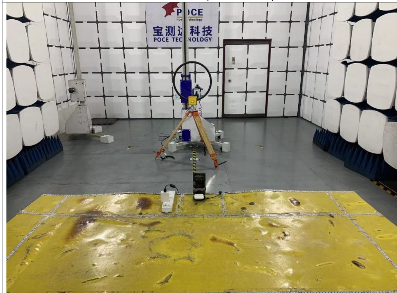
Radiated emissions (0.009MHz-30MHz)
