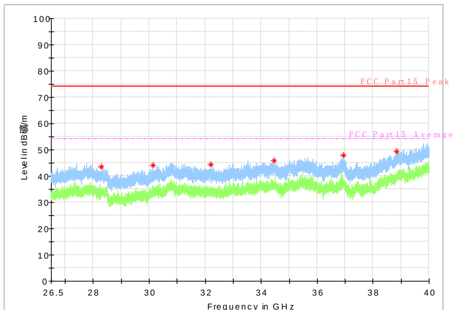
Fig. 33 Radiated Spurious Emission (802.11a, ch36, 26.5 GHz-40 GHz)
