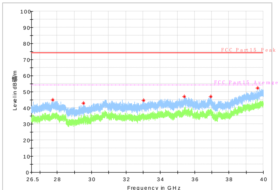
Fig. 43 Radiated Spurious Emission (802.11n-HT40, ch38, 26.5 GHz-40 GHz)
