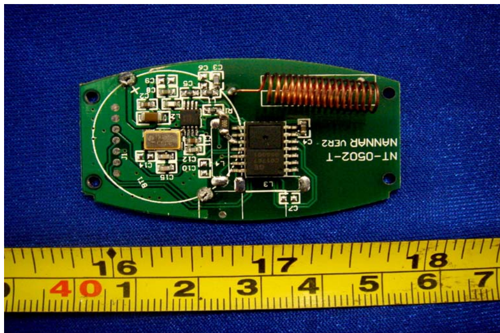
PCB-Front View
