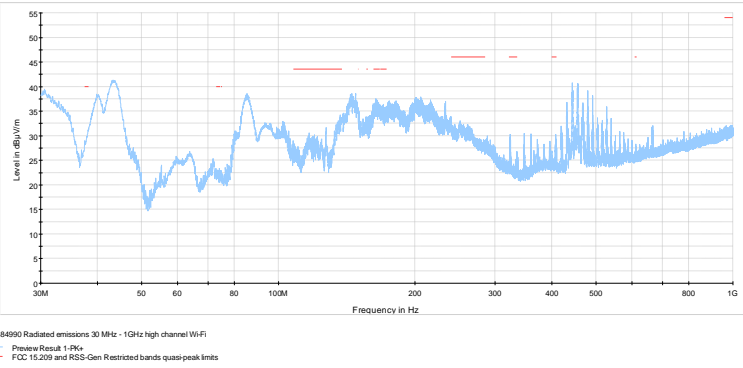
Figure 8.5-15: Radiated spurious emissions below 1 GHz, high channel
