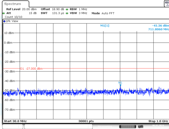
11A-CDD_Ant1_5700_30~1000
