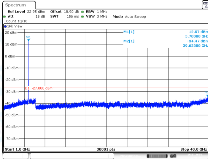
11A-CDD_Ant1_5700_1000~40000
