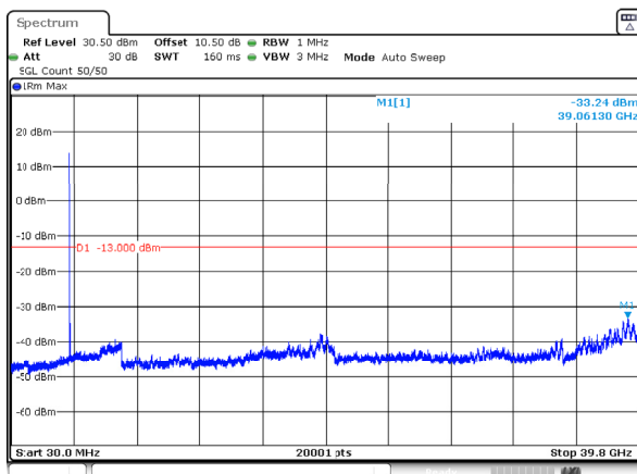
n77_3_50MHz_30kHz_3725MHz_DFT-s-OFDM QPSK_RB1@0 -33.24dBm
