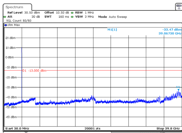
n77_3_30MHz_30kHz_3965MHz_DFT-s-OFDM QPSK_RB1@77 -33.47dBm
