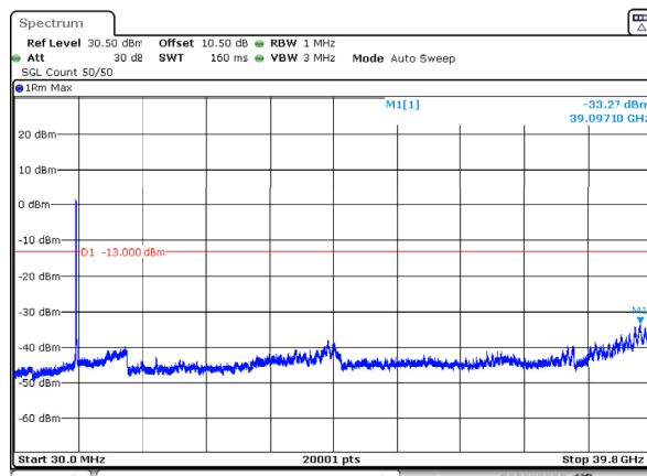
n77_3_60MHz_30kHz_3840MHz_DFT-s-OFDM QPSK_RB162@0 -33.27dBm
