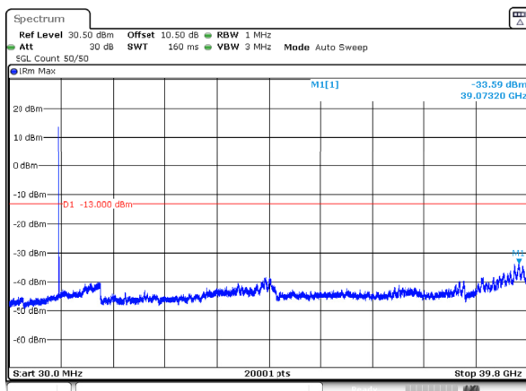
n77_3_40MHz_30kHz_3840MHz_DFT-s-OFDM QPSK_RB1@0 -33.59dBm
