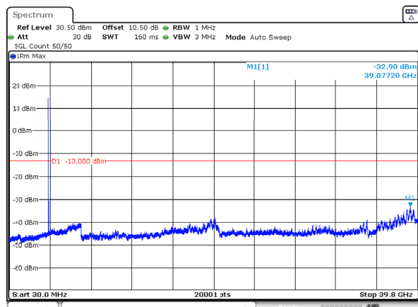
n77_3_30MHz_30kHz_3840MHz_DFT-s-OFDM QPSK_RB1@0 -32.90dBm
