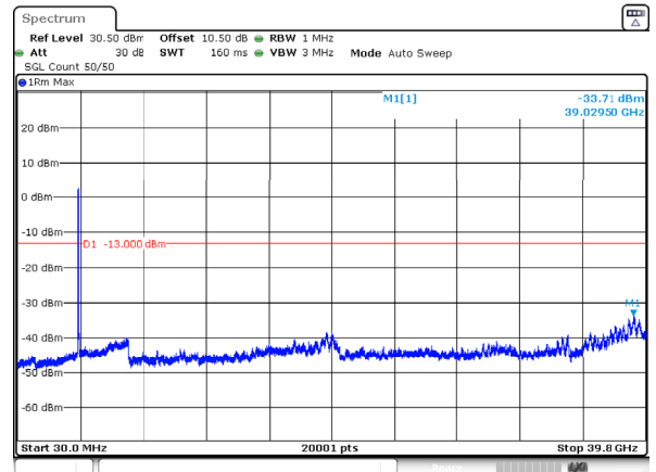
n77_3_40MHz_30kHz_3840MHz_DFT-s-OFDM QPSK_RB100@0 -33.71dBm
