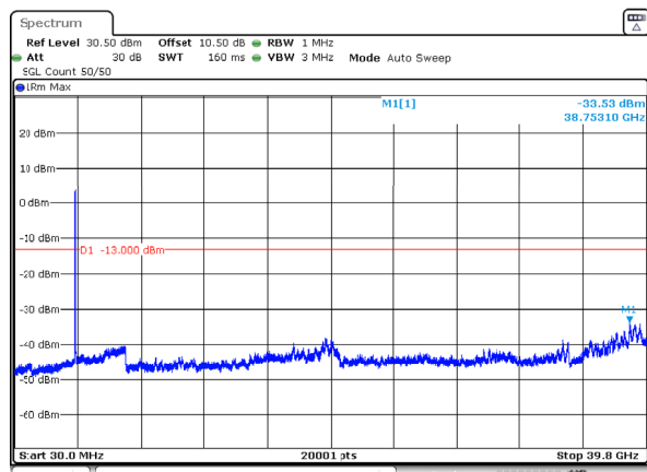
n77_3_30MHz_30kHz_3840MHz_DFT-s-OFDM QPSK_RB75@0 -33.53dBm
