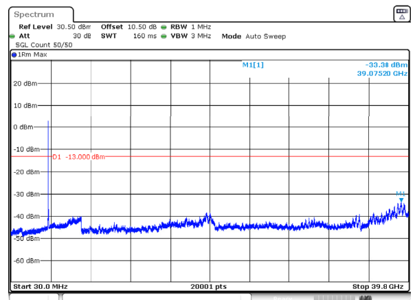
n77_3_30MHz_30kHz_3715MHz_DFT-s-OFDM QPSK_RB75@0 -33.38dBm
