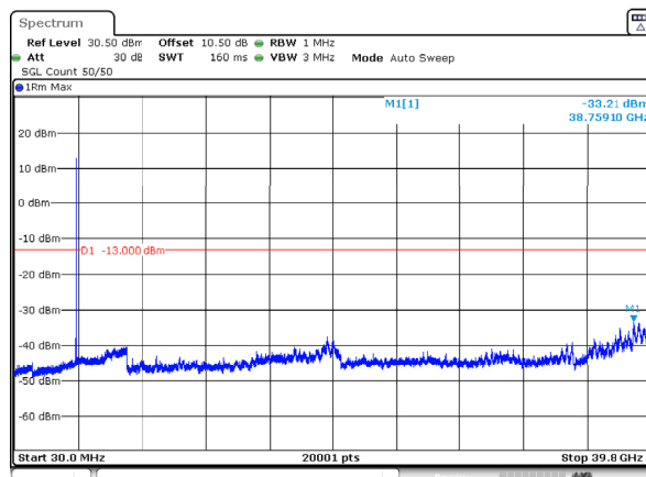
n77_3_30MHz_30kHz_3840MHz_DFT-s-OFDM QPSK_RB1@77 -33.21dBm
