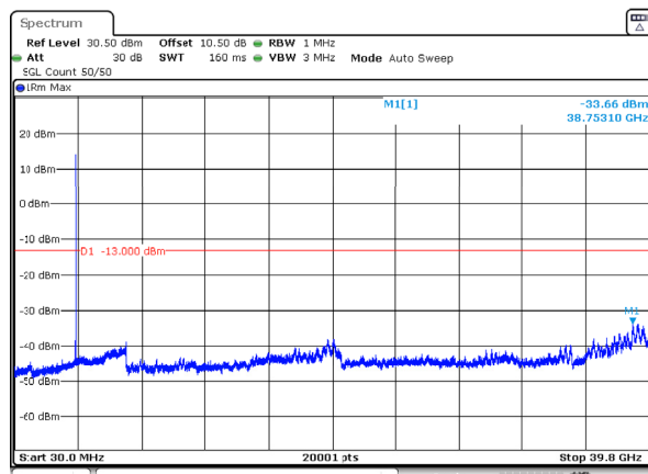
n77_3_70MHz_30kHz_3840MHz_DFT-s-OFDM QPSK_RB1@188 -33.66dBm
