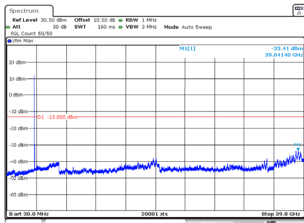
n77_3_80MHz_30kHz_3740MHz_DFT-s-OFDM QPSK_RB1@0 -33.41dBm
