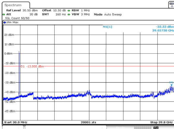
n77_3_40MHz_30kHz_3720MHz_DFT-s-OFDM QPSK_RB100@0 -33.53dBm
