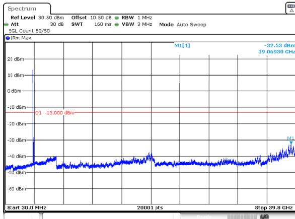
n77_3_90MHz_30kHz_3840MHz_DFT-s-OFDM QPSK_RB1@0 -32.53dBm
