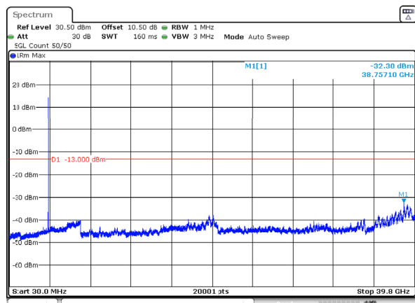
n77_3_80MHz_30kHz_3840MHz_DFT-s-OFDM QPSK_RB1@216 -32.30dBm
