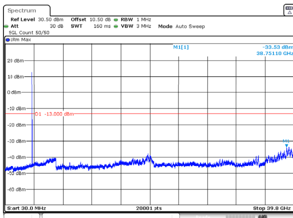
n77_3_30MHz_30kHz_3715MHz_DFT-s-OFDM QPSK_RB1@77 -33.53dBm
