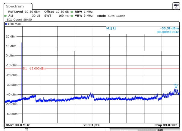
n77_3_50MHz_30kHz_3725MHz_DFT-s-OFDM QPSK_RB1@132 -33.58dBm
