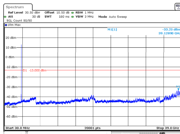
n77_3_70MHz_30kHz_3735MHz_DFT-s-OFDM QPSK_RB1@188 -33.23dBm
