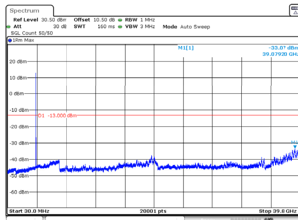
n77_3_70MHz_30kHz_3840MHz_DFT-s-OFDM QPSK_RB1@0 -33.07dBm
