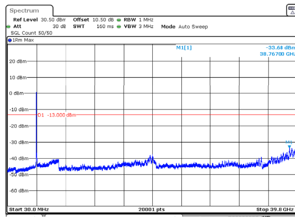
n77_3_70MHz_30kHz_3945MHz_DFT-s-OFDM QPSK_RB180@0 -33.68dBm
