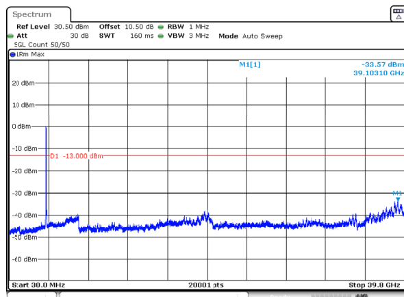
n77_3_60MHz_30kHz_3730MHz_DFT-s-OFDM QPSK_RB162@0 -33.57dBm
