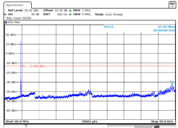
n77_3_90MHz_30kHz_3745MHz_DFT-s-OFDM QPSK_RB1@0 -32.89dBm
