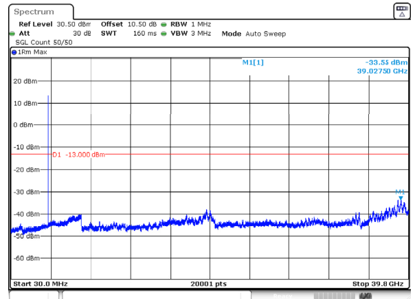
n77_3_30MHz_30kHz_3715MHz_DFT-s-OFDM QPSK_RB1@0 -33.55dBm
