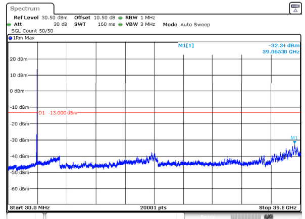
n77_3_90MHz_30kHz_3840MHz_DFT-s-OFDM QPSK_RB1@244 -32.34dBm
