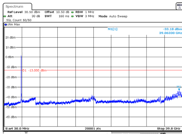
n77_3_70MHz_30kHz_3840MHz_DFT-s-OFDM QPSK_RB180@0 -33.18dBm
