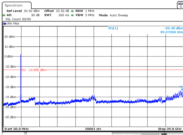
n77_3_50MHz_30kHz_3840MHz_DFT-s-OFDM QPSK_RB128@0 -33.40dBm
