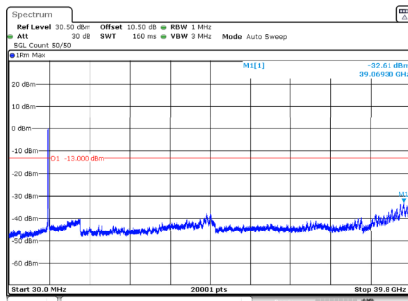
n77_3_80MHz_30kHz_3840MHz_DFT-s-OFDM QPSK_RB216@0 -32.61dBm
