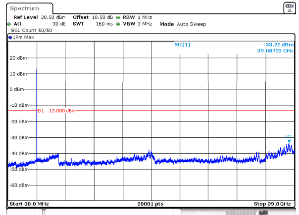
n77_3_40MHz_30kHz_3960MHz_DFT-s-OFDM QPSK_RB1@0 -33.22dBm
