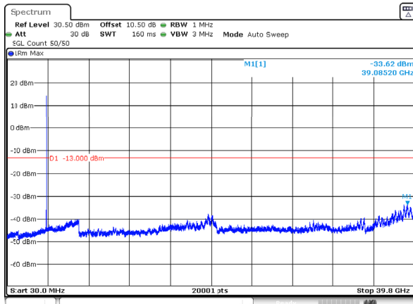
n77_3_50MHz_30kHz_3840MHz_DFT-s-OFDM QPSK_RB1@132 -33.62dBm
