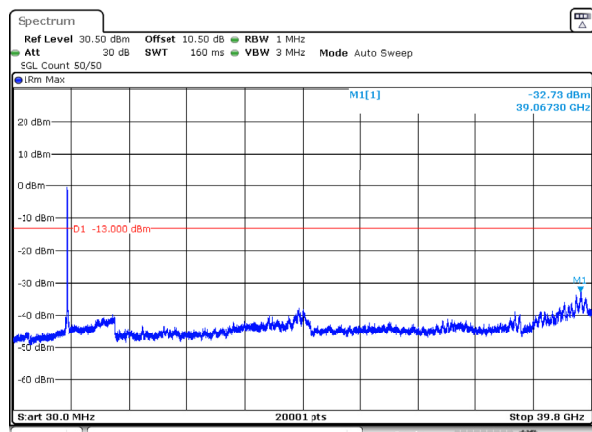
n77_3_80MHz_30kHz_3740MHz_DFT-s-OFDM QPSK_RB216@0 -32.73dBm
