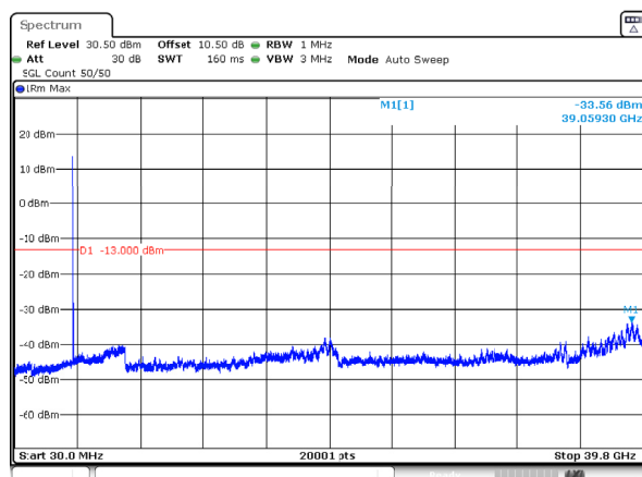
n77_3_70MHz_30kHz_3735MHz_DFT-s-OFDM QPSK_RB1@0 -33.56dBm
