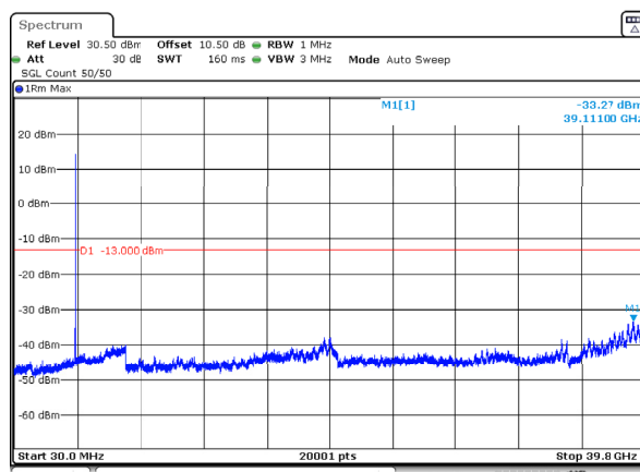
n77_3_60MHz_30kHz_3840MHz_DFT-s-OFDM QPSK_RB1@161 -33.27dBm
