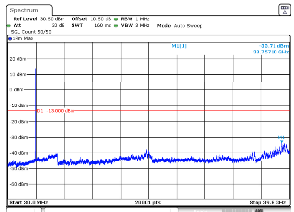
n77_3_40MHz_30kHz_3840MHz_DFT-s-OFDM QPSK_RB1@105 -33.71dBm
