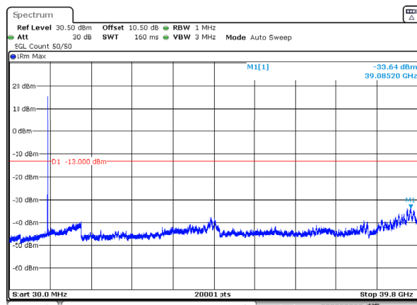
n77_3_60MHz_30kHz_3730MHz_DFT-s-OFDM QPSK_RB1@161 -33.64dBm
