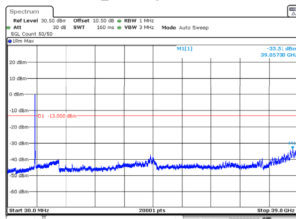
n77_3_70MHz_30kHz_3735MHz_DFT-s-OFDM QPSK_RB180@0 -33.51dBm
