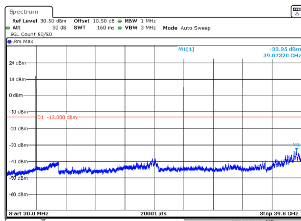
n77_3_70MHz_30kHz_3945MHz_DFT-s-OFDM QPSK_RB1@0 -33.35dBm
