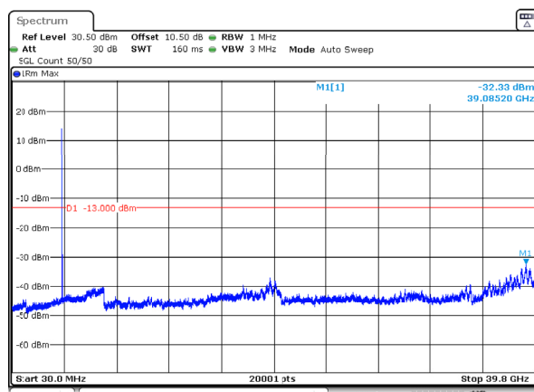
n77_3_60MHz_30kHz_3840MHz_DFT-s-OFDM QPSK_RB1@0 -32.33dBm
