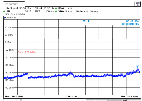
n77_3_50MHz_30kHz_3840MHz_DFT-s-OFDM QPSK_RB1@0 -33.43dBm
