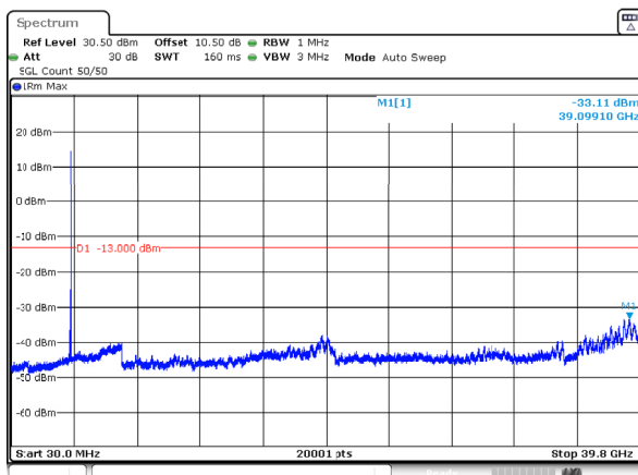
n77_3_90MHz_30kHz_3745MHz_DFT-s-OFDM QPSK_RB1@244 -33.11dBm
