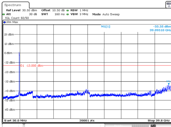
n77_3_90MHz_30kHz_3840MHz_DFT-s-OFDM QPSK_RB243@0 -33.35dBm
