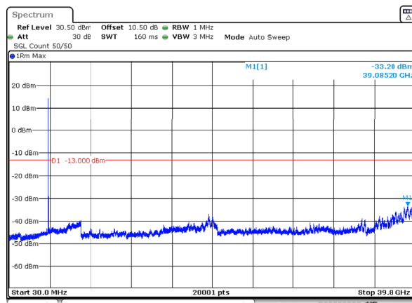
n77_3_80MHz_30kHz_3840MHz_DFT-s-OFDM QPSK_RB1@0 -33.20dBm
