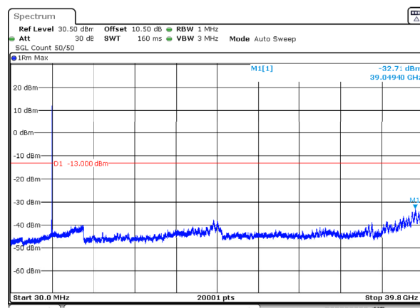
n77_3_70MHz_30kHz_3945MHz_DFT-s-OFDM QPSK_RB1@188 -32.71dBm
