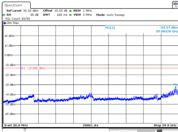
n77_3_40MHz_30kHz_3960MHz_DFT-s-OFDM QPSK_RB1@105 -33.37dBm
