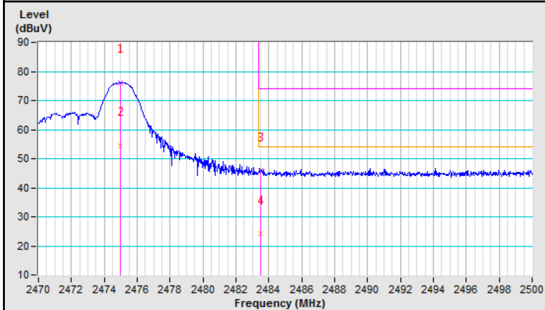
2475MHz Vertical
