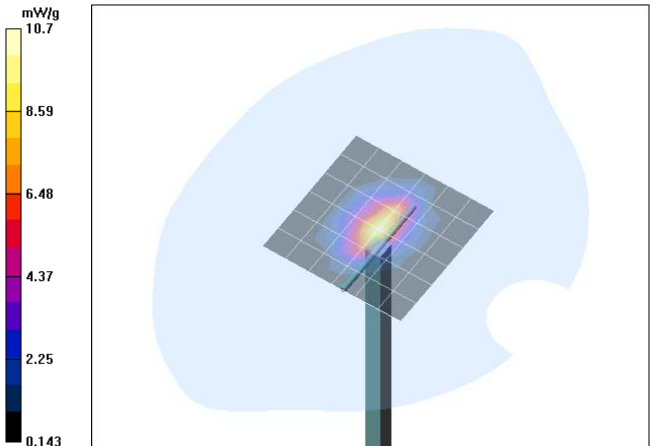
Fig. 10: Validation measurement 1900 MHz Head (March 04, 2005), coarse grid. Ambient Temperature: 22.0° C, Liquid Temperature: 21.0° C.
