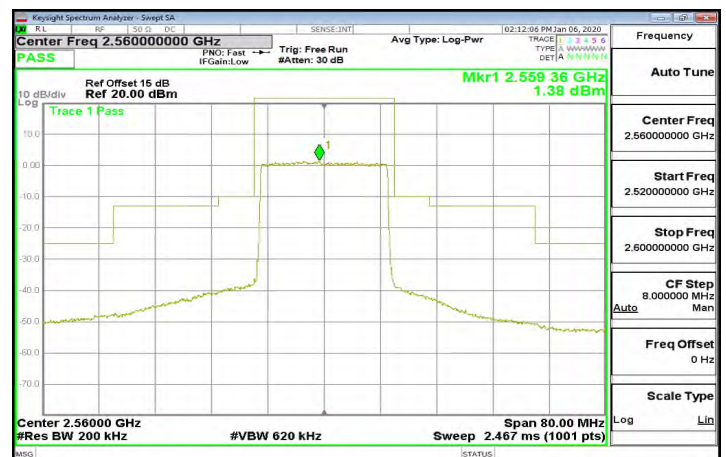
Band7_20MHz_64QAM_100_0_CH21350
