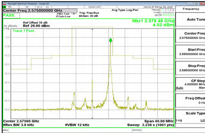
Band38_10MHz_QPSK_1_49_CH38000
