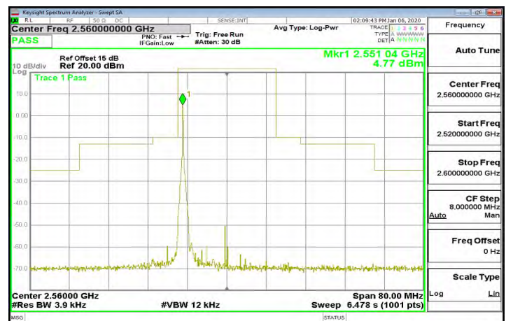
Band7_20MHz_64QAM_1_0_CH21350
