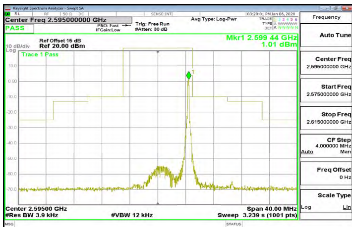
Band38_10MHz_64QAM_1_49_CH38200
