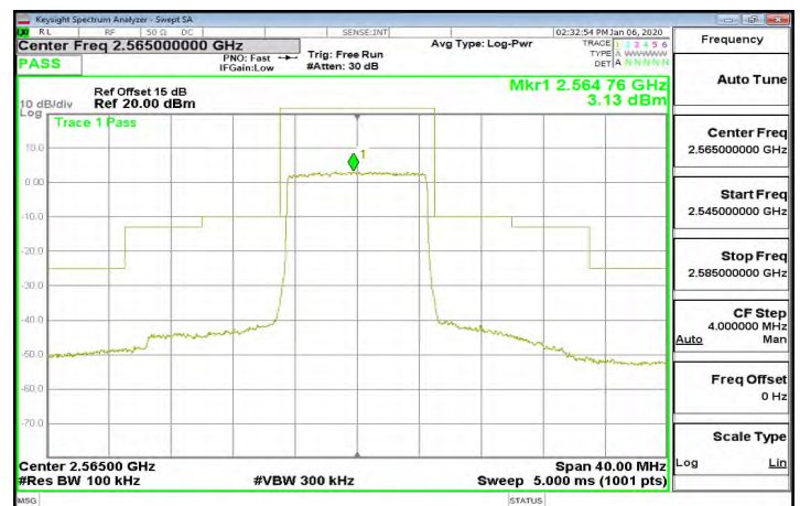
Band7_10MHz_QPSK_50_0_CH21400
