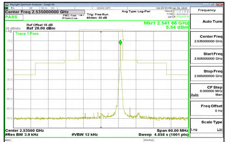
Band7_15MHz_64QAM_1_74_CH21375
