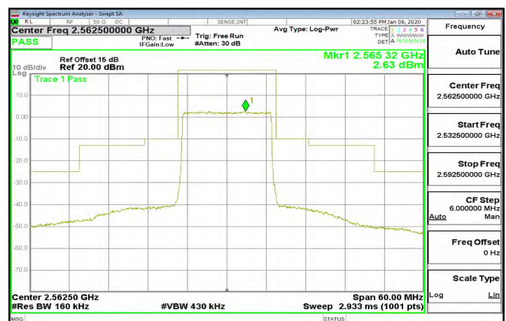
Band7_15MHz_16QAM_75_0_CH21375
