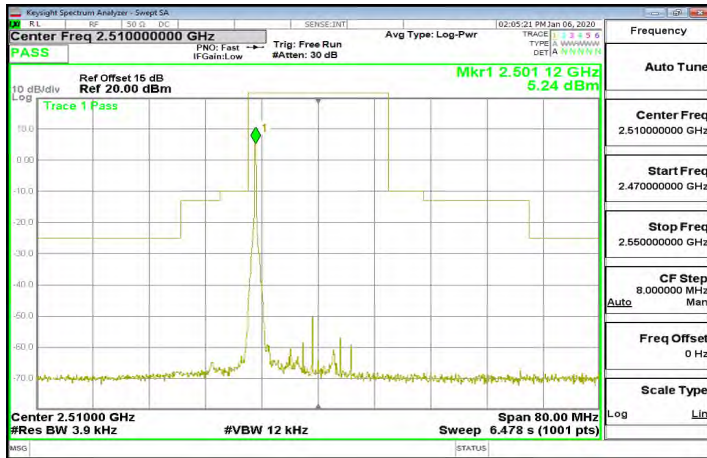
Band7_20MHz_16QAM_1_0_CH21100
