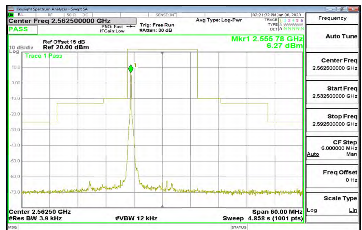
Band7_15MHz_16QAM_1_0_CH21375
