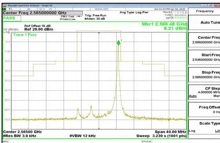
Band7_10MHz_QPSK_1_49_CH21400
