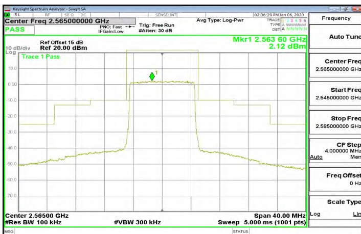
Band7_10MHz_16QAM_50_0_CH21400
