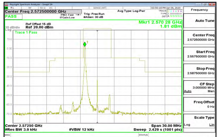
Band38_5MHz_16QAM_1_0_CH38000
