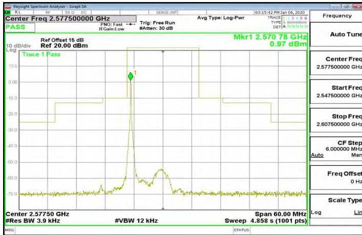
Band38_15MHz_64QAM_1_0_CH38000
