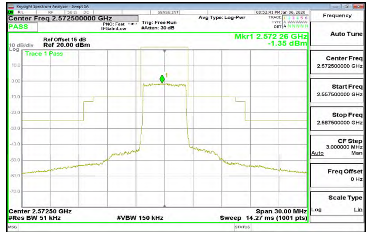
Band38_5MHz_16QAM_25_0_CH38000
