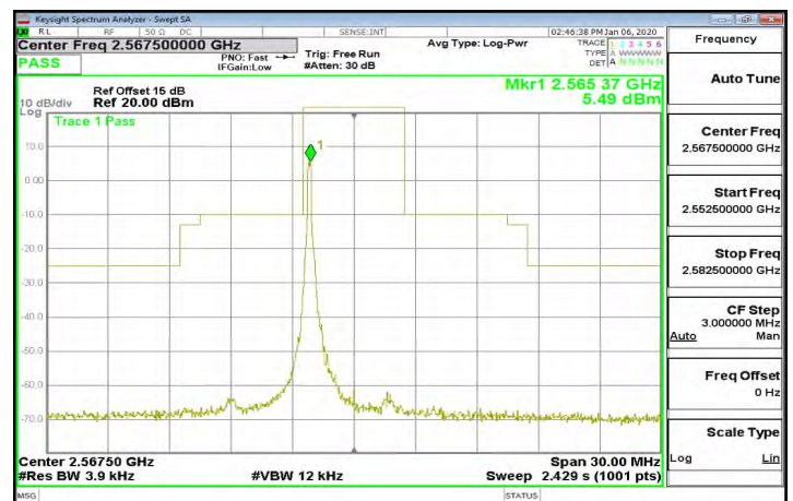
Band7_5MHz_16QAM_1_0_CH21425
