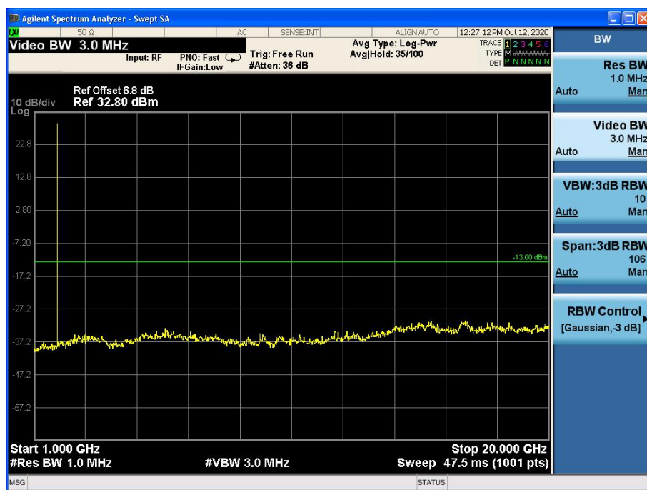
Channel 661, 1GHz~20GHz
