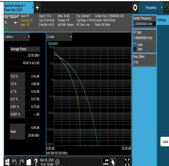
NTVN-N41-PC3-30-60-L-DFT-QPSK-Outer Full-PASS
