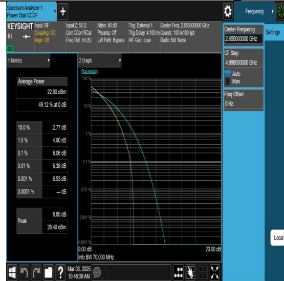
NTNV-N41-PC3-30-70-H-DFT-QPSK-Outer Full-PASS
