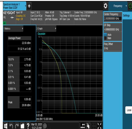
NTV-N41-PC3-30-15-L-DFT-QPSK-Outer Full-PASS
