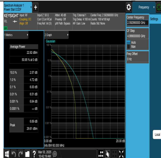
NTVN-N41-PC3-30-60-M-DFT-QPSK-Outer Full-PASS
