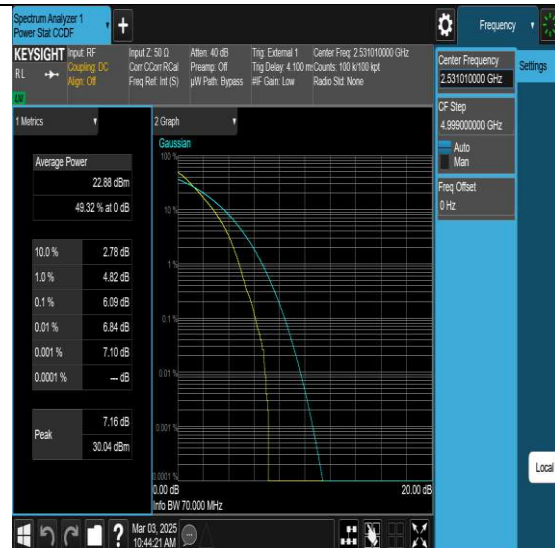
NTNV-N41-PC3-30-70-L-DFT-QPSK-Outer Full-PASS
