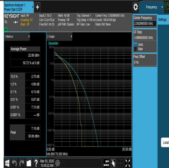
NTNV-N41-PC3-30-70-M-DFT-QPSK-Outer Full-PASS
