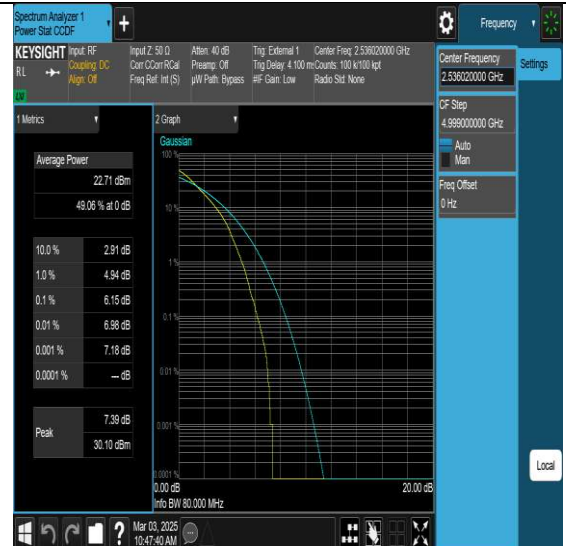
NTVN-N41-PC3-30-80-L-DFT-QPSK-Outer Full-PASS
