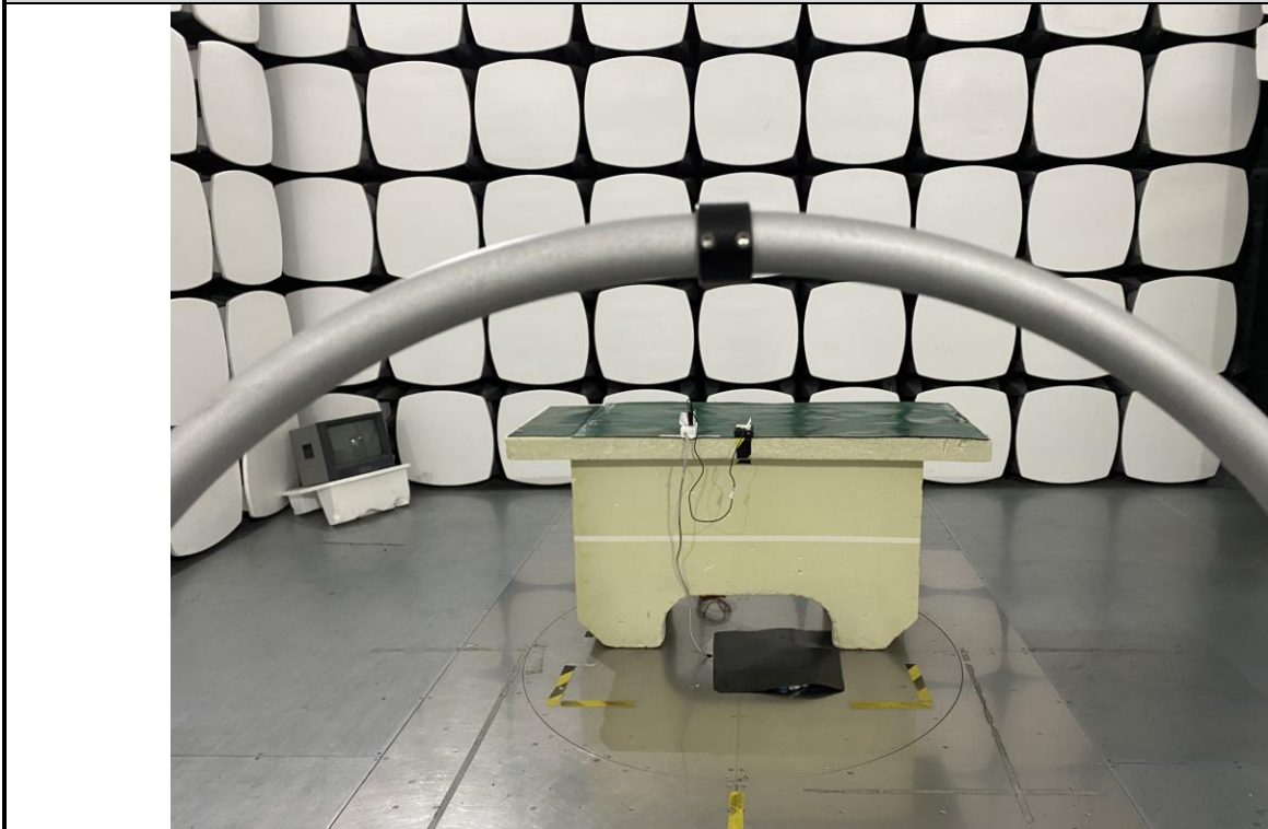
Radiated emission Test Setup (9 kHz to 30 MHz)
