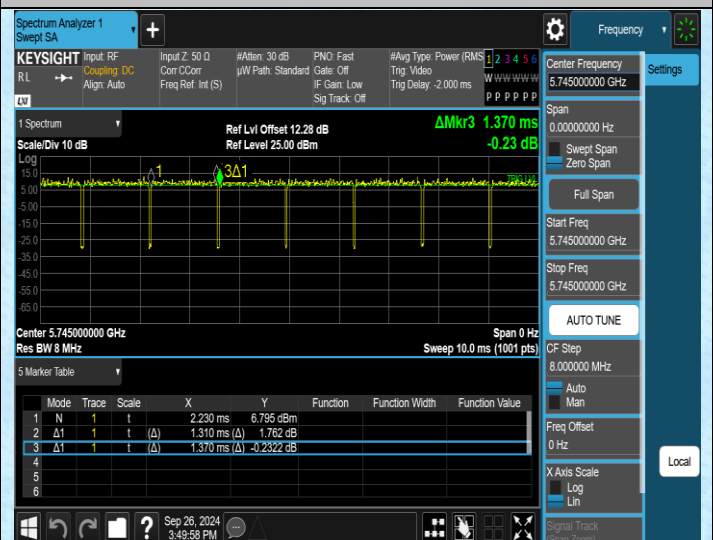
NTNV-11AC20MIMO-Ant2-5745
