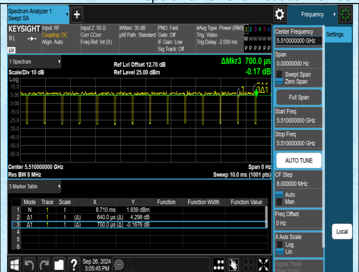
NTNV-11N40MIMO-Ant2-5510
