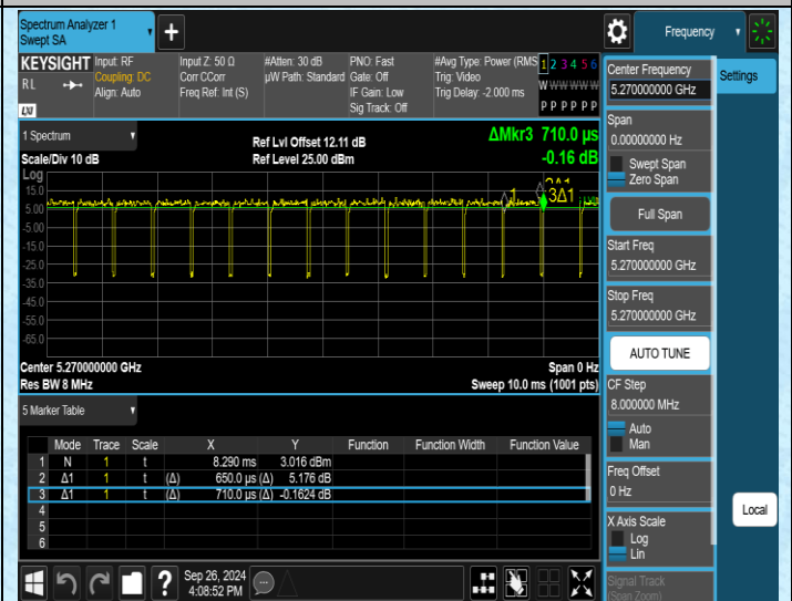
NTNV-11AC40MIMO-Ant2-5270
