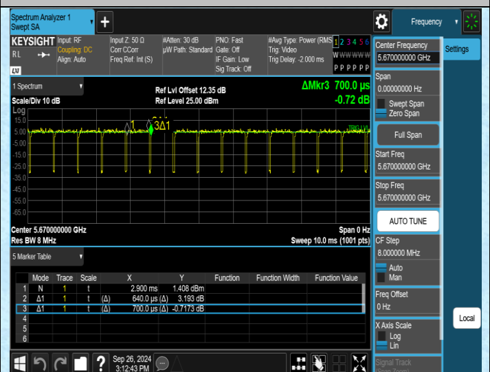
NTNV-11N40MIMO-Ant2-5670
