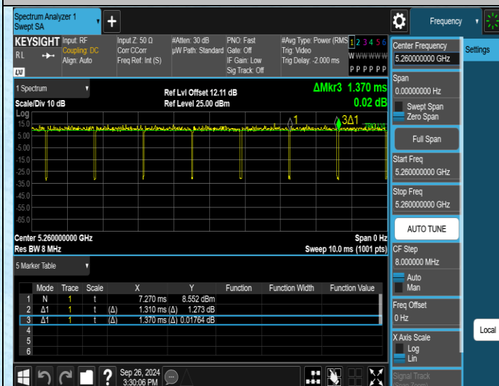
NTNV-11AC20MIMO-Ant1-5260
