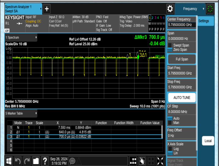
NTNV-11N40MIMO-Ant2-5795
