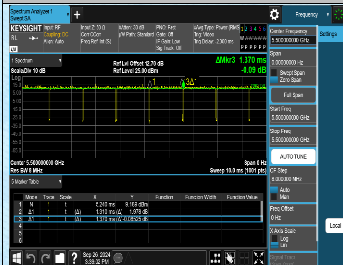
NTNV-11AC20MIMO-Ant1-5500
