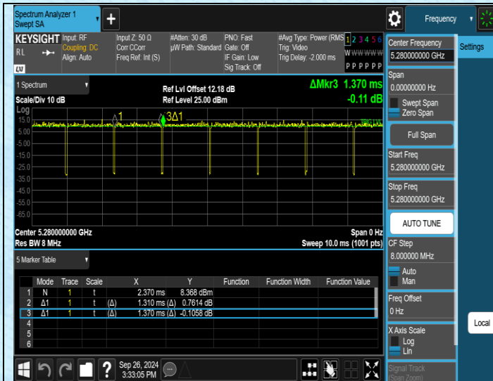
NTNV-11AC20MIMO-Ant1-5280
