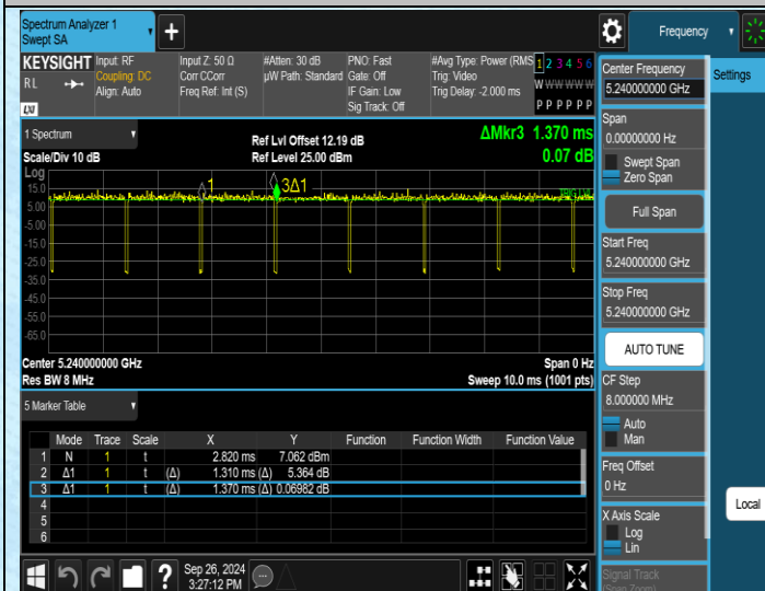
NTNV-11AC20MIMO-Ant1-5240
