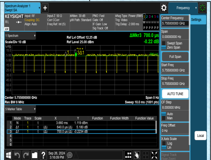
NTNV-11N40MIMO-Ant2-5755
