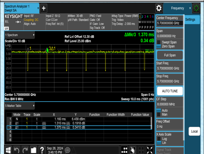
NTNV-11AC20MIMO-Ant2-5700
