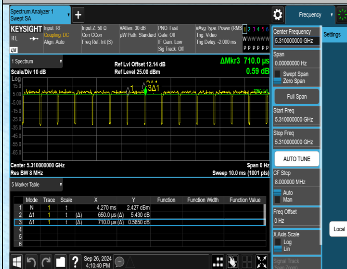
NTNV-11AC40MIMO-Ant1-5310
