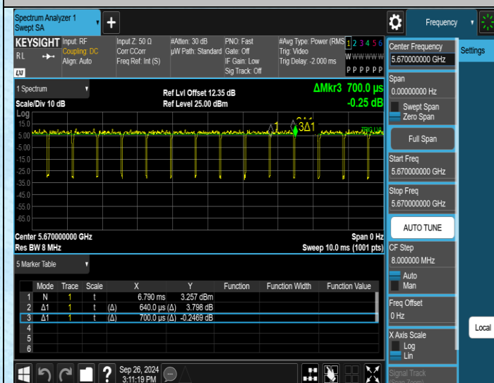
NTNV-11N40MIMO-Ant1-5670
