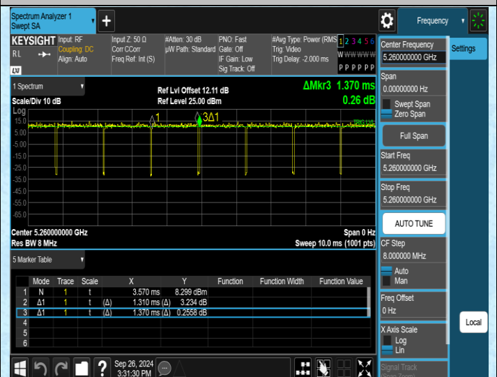
NTNV-11AC20MIMO-Ant2-5260
