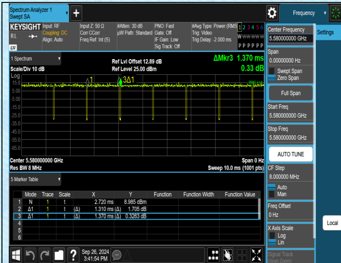
NTNV-11AC20MIMO-Ant1-5580
