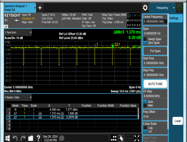
NTNV-11AC20MIMO-Ant2-5180
