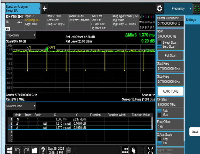
NTNV-11AC20MIMO-Ant1-5745
