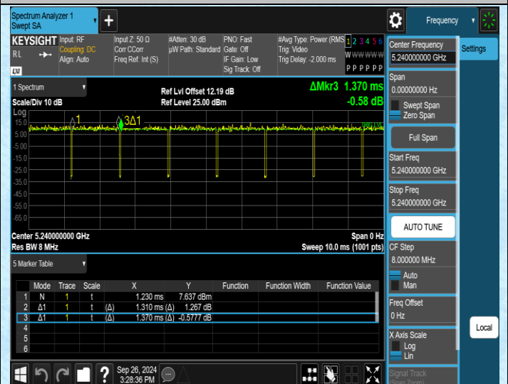
NTNV-11AC20MIMO-Ant2-5240
