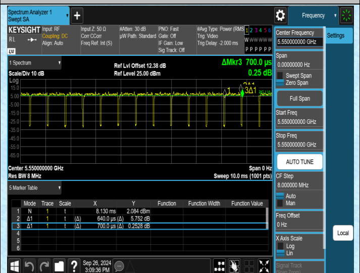
NTNV-11N40MIMO-Ant2-5550
