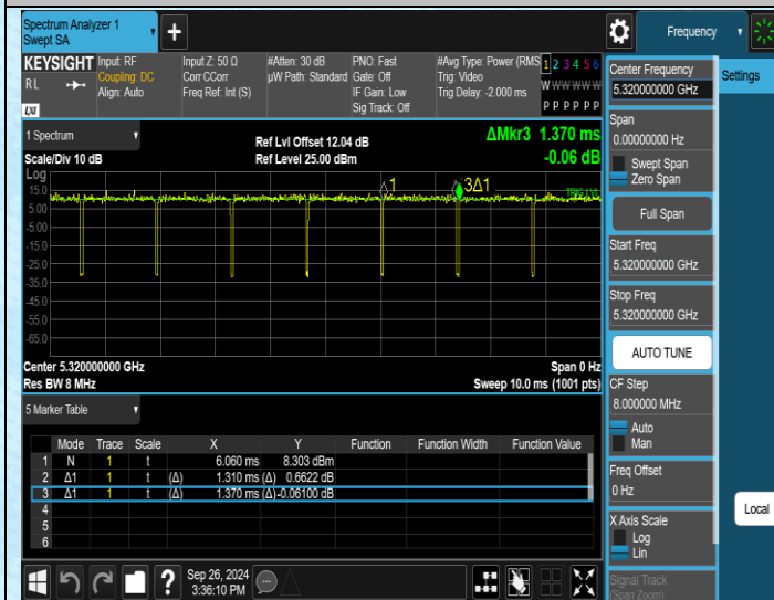
NTNV-11AC20MIMO-Ant1-5320
