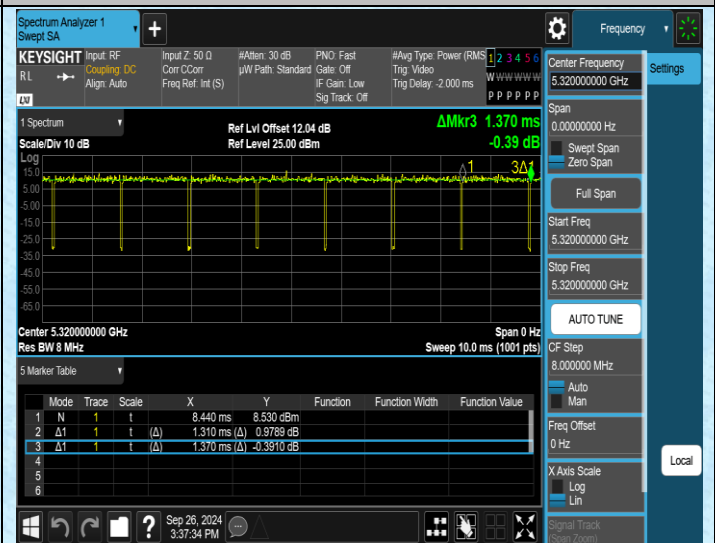
NTNV-11AC20MIMO-Ant2-5320
