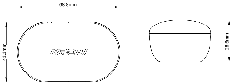
Charging box
