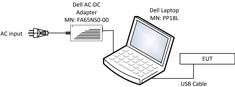
Figure 3.6-2: AC conducted Emissions Setup diagram
