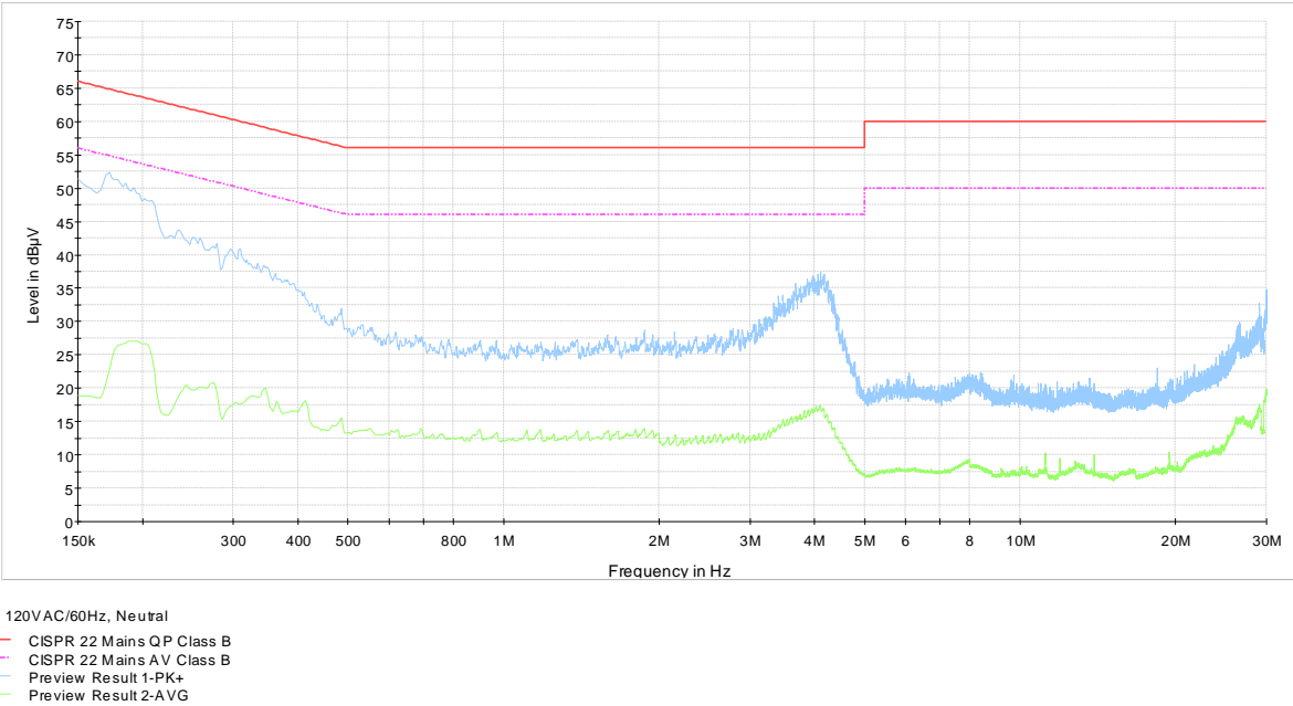
Figure 8.1-2 Conducted emissions on neutral line
