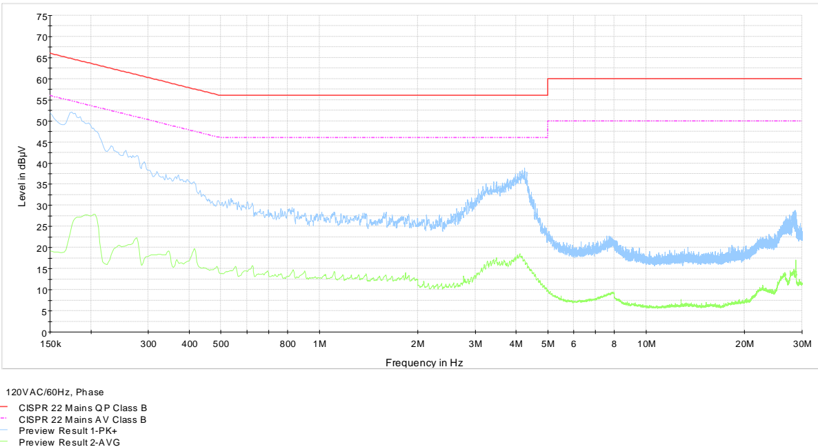
Figure 8.1-1 Conducted emissions on phase line
