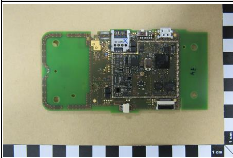
PCB BOTTOM WITHOUT SHIELDING
