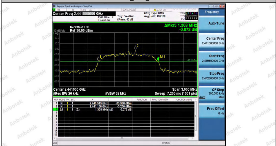
2DH5_Ant1_2441
