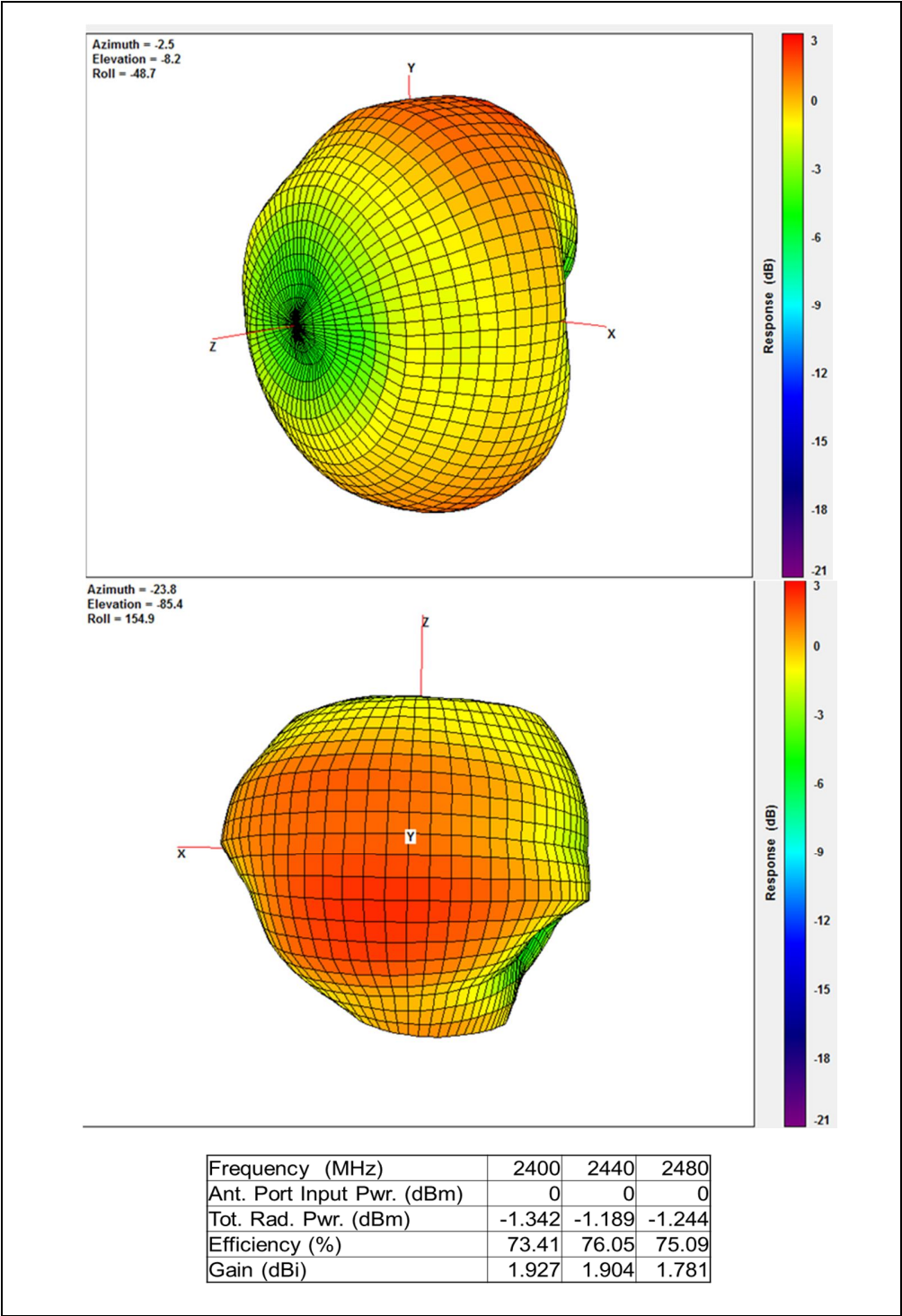
FIGURE 1-1: BM64 ANTENNA RADIATION PATTERN
