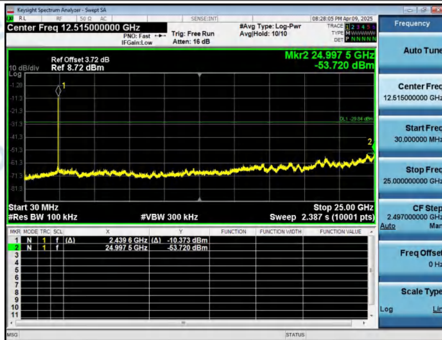
1_Reference_Level_NVNT_ANT1_802_11n(HT20)_2462
