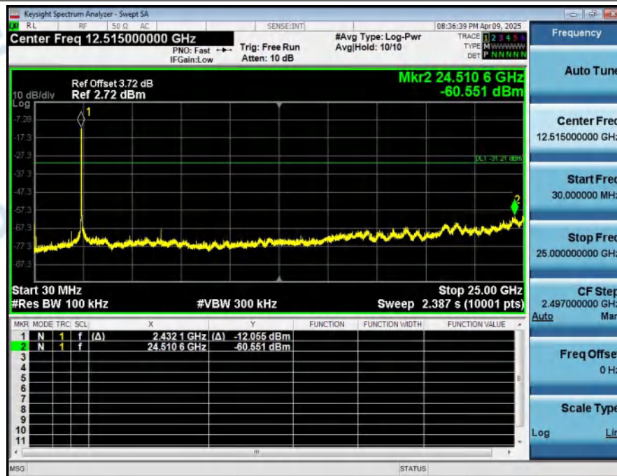
1_Reference_Level_NVNT_ANT1_802_11n(HT40)_2452
