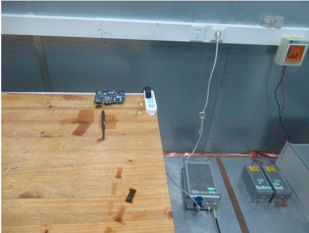
Picture 1: Conducted Emissions Test Setup
