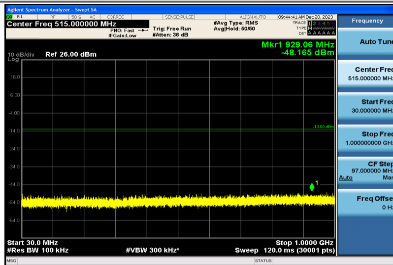
Band2-1.4MHz-16QAM-19193-1RB#0-30~1000MHz
