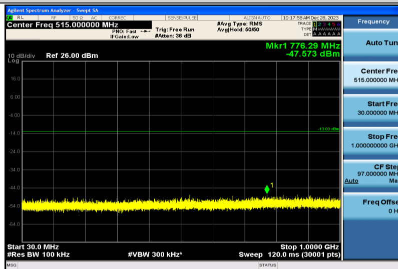
Band2-5MHz-16QAM-18900-1RB#0-30~1000MHz
