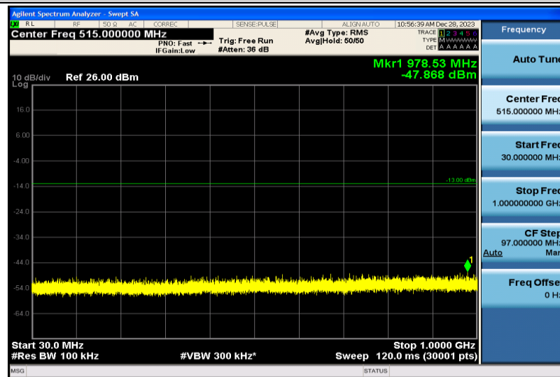
Band2-15MHz-QPSK-19125-1RB#0-30~1000MHz
