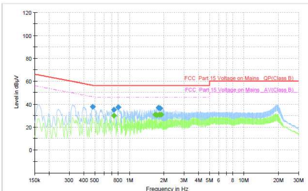
Figure 9: Spectral Diagrams, Conducted Emission, 150KHz - 30MHz, N, Model 62005000
