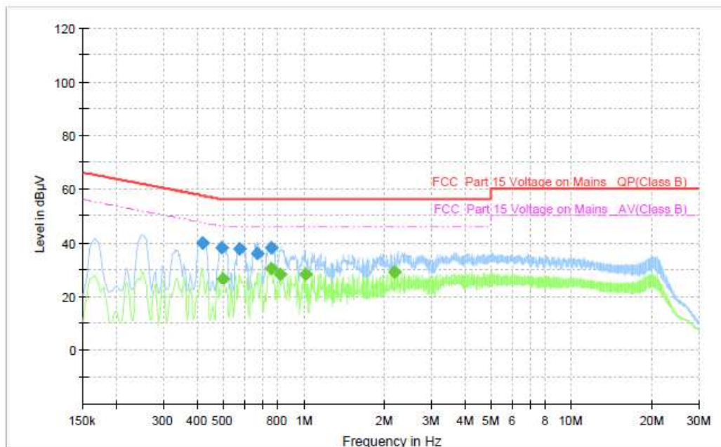
Figure 7: Spectral Diagrams, Conducted Emission, 150KHz - 30MHz, N, Model 62022000
