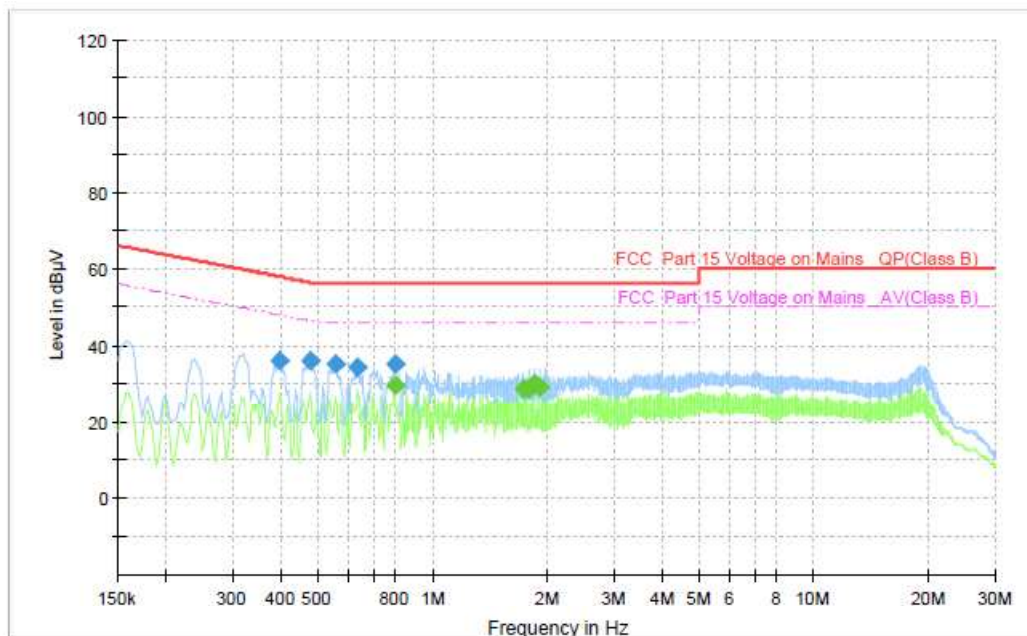
Figure 8: Spectral Diagrams, Conducted Emission, 150KHz - 30MHz, L, Model 62005000
