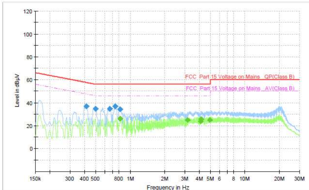
Figure 6: Spectral Diagrams, Conducted Emission, 150KHz - 30MHz, L, Model 62022000
