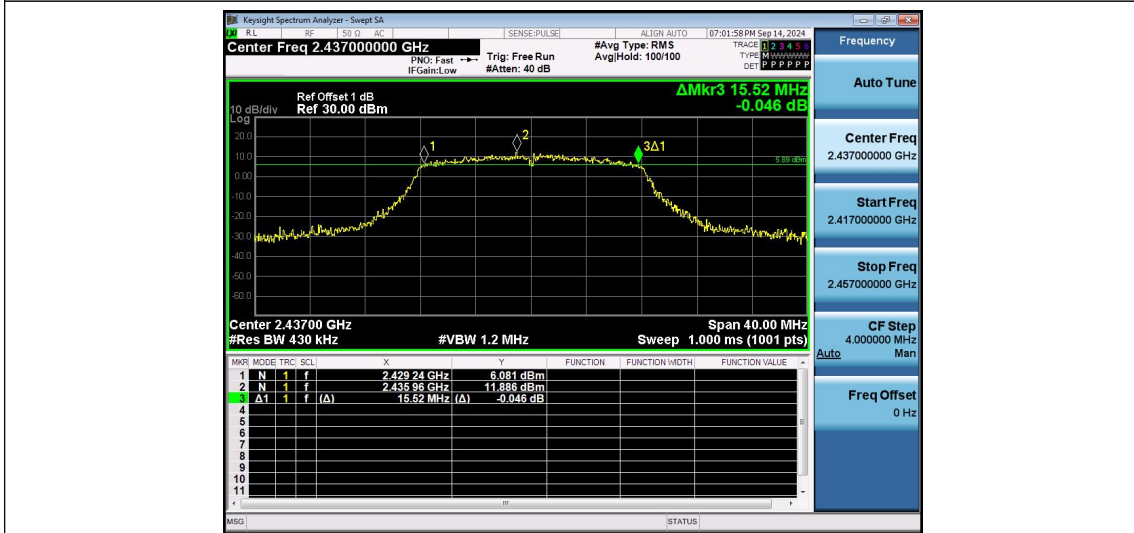
802.11g-Ant1-2437-PASS
