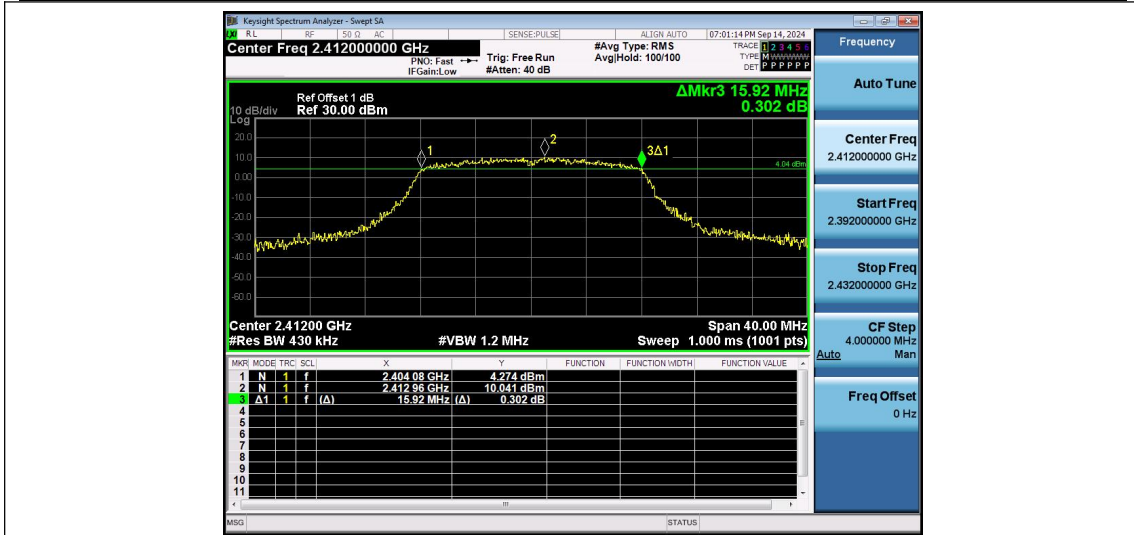
802.11g-Ant1-2412-PASS
