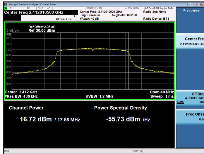
802.11n(HT20)SISO-Ant1-2412-PASS
