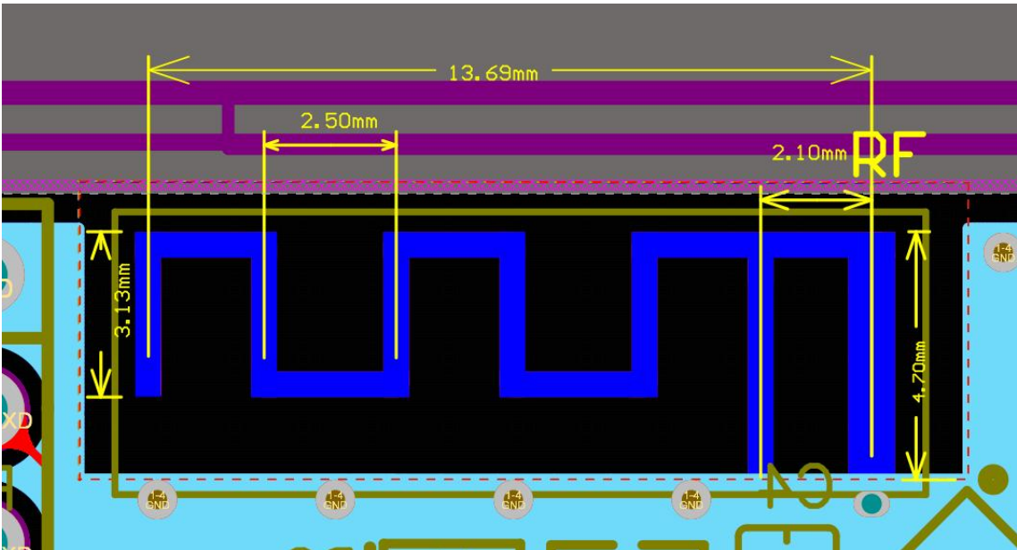
Antenna Photo & Length (mm)
