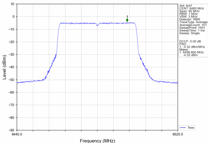
802.11ax(HEW40)_MCH_6485MHz_RU484_Left_Ant1_NTNV
