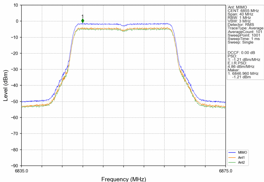
802.11ax(HEW20)_HCH_6855MHz_RU242_Left_MIMO_NTNV
