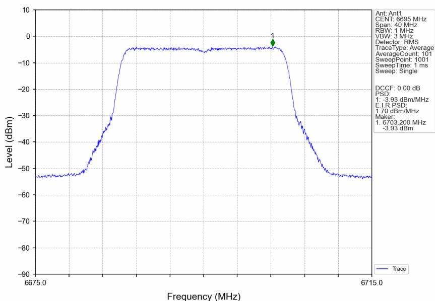
802.11ax(HEW20)_MCH_6695MHz_RU242_Left_Ant1_NTNV
