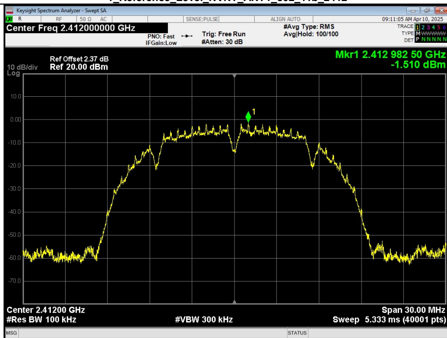
2 Bandedge_NVNT_ANT1_802_11b_2412
