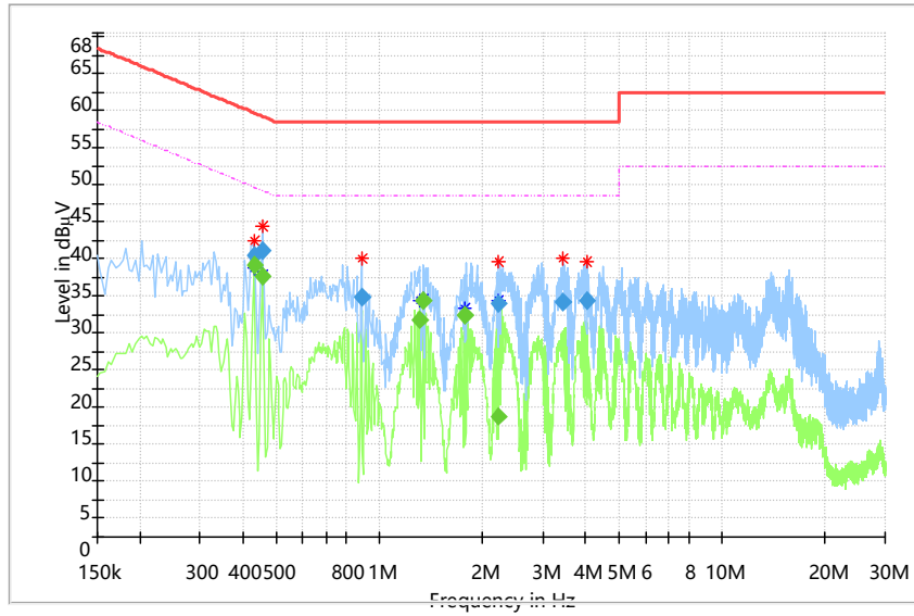
Full Spectrum
