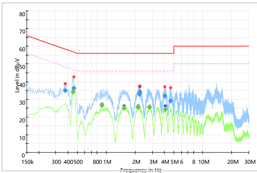
Full Spectrum
