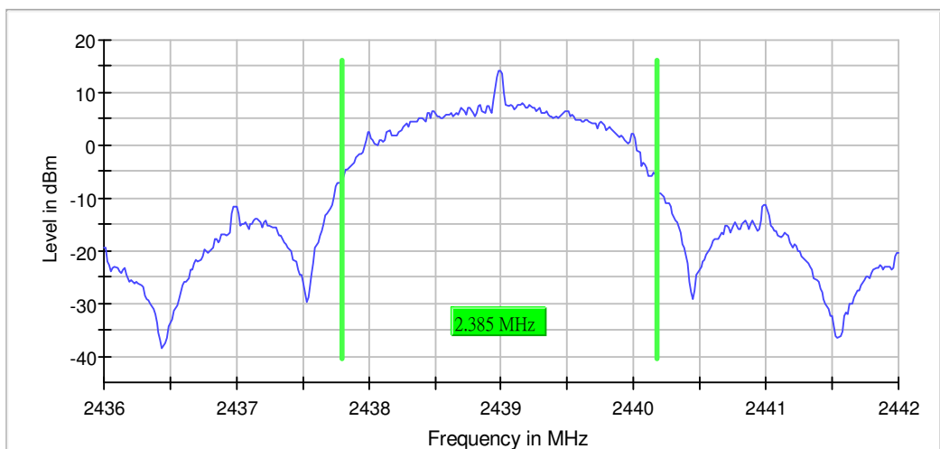
20 dB Bandwidth
