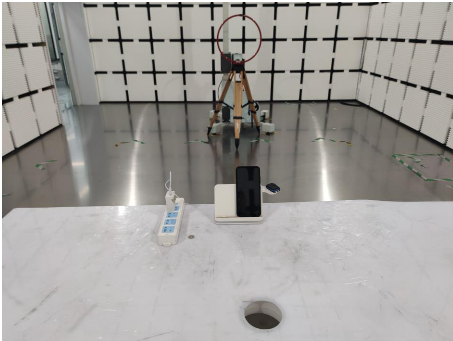
Radiation (9KHz-30MHz)
