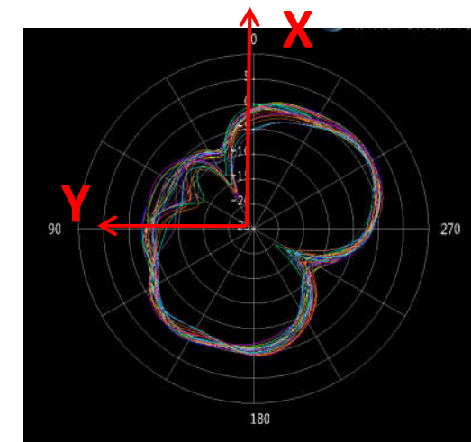
H (Theta=90)
