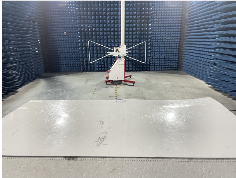
Test Model No.: Stellar Pro-266R-N Radiated Emission
