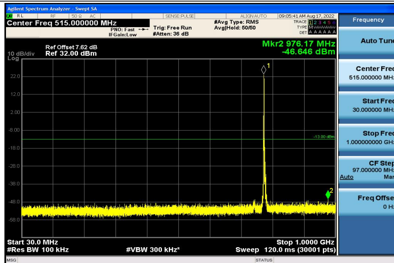
Band13-5MHz-QPSK-23205-1RB#0-30~1000MHz
