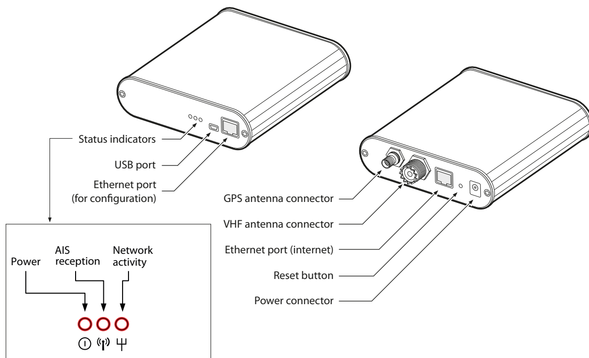
Figure 5 Coast Station connections
