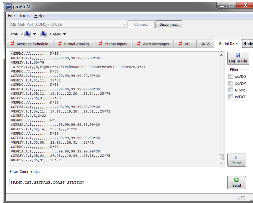
Figure 8 Configuration of Coast Station name in AIS receiver mode
