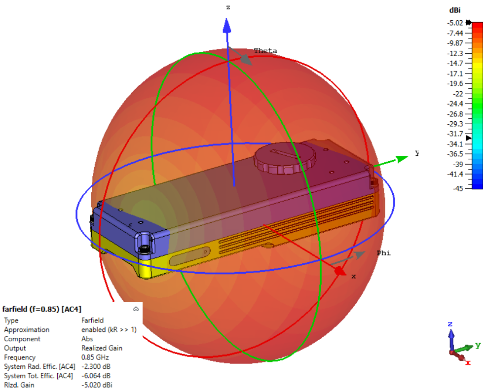
Radiation pattern @ 850MHz
