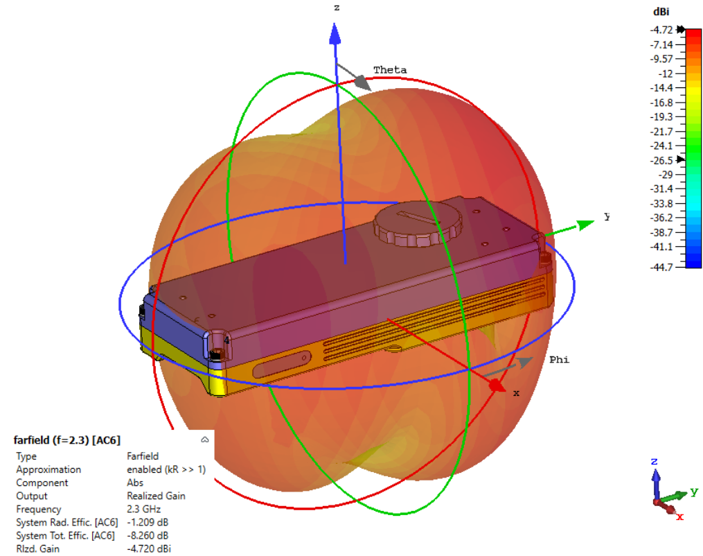
Radiation pattern @ 2300MHz
