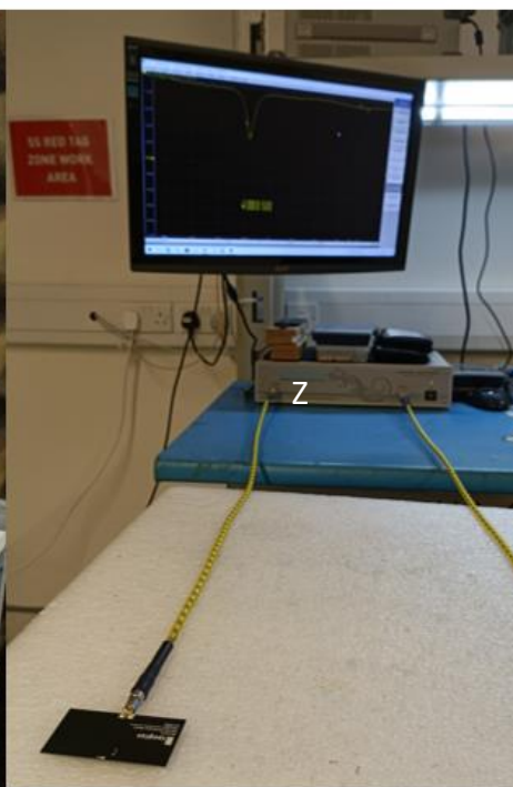
VNA Setup
