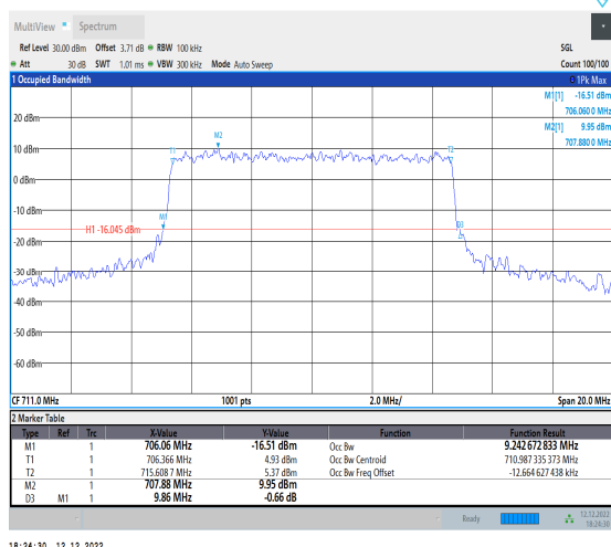
1-N12-15-10-H-8-CP-64QAM-Outer_Full-52@0-Ant1 -9.243-9.860-≤10-PASS
