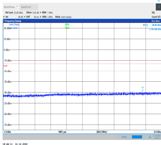
1-N12-15-15-H-1-DFT-PI2BPSK-Inner_1RB_Left-1@ 1-1000-3000-Ant1-2762.50--38.89--13-PASS
