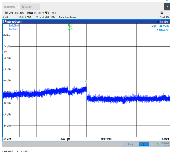
1-N12-15-15-L-1-DFT-PI2BPSK-Inner_1RB_Left-1 @ 1-3000-12000-Ant1-7482.00--44.27--13-PASS
