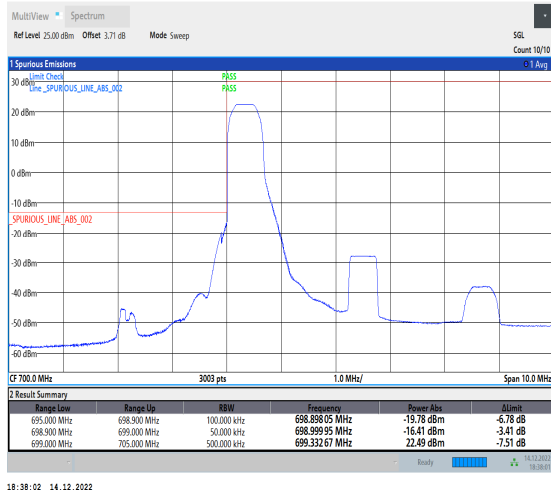
1-N12-15-5-L-1-DFT-PI2BPSK-Edge_1RB_Left-1@0-A nt1-1--PASS-see graph
