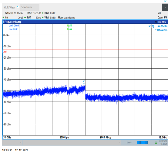
1-N12-15-15-M-1-DFT-PI2BPSK-Inner_1RB_Left-1 @1-3000-12000-Ant1-7422.60--44.72--13-PASS
