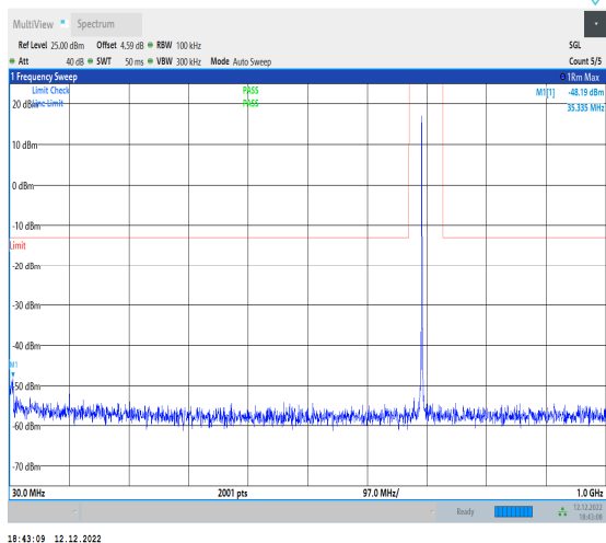
1-N12-15-15-M-1-DFT-PI2BPSK-Inner_1RB_Left-1 @1-30-1000-Ant1-35.34--48.19--13-PASS
