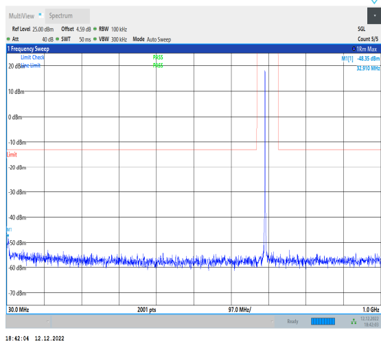
1-N12-15-15-L-1-DFT-PI2BPSK-Inner_1RB_Left-1 @1-30-1000-Ant1-32.91--48.35--13-PASS
