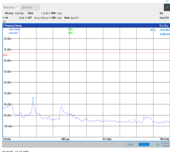
1-N12-15-15-M-1-DFT-PI2BPSK-Inner_1RB_Left-1 @ 1-0.009-0.15-Ant1-0.03--78.24--33-PASS
