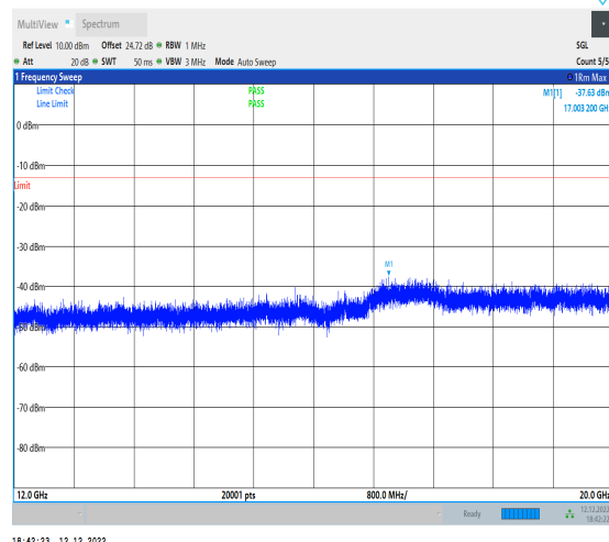
1-N12-15-15-L-1-DFT-PI2BPSK-Inner_1RB_Left-1@ 1-12000-20000-Ant1-17003.20--37.63--13-PASS
