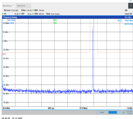
1-N12-15-15-H-1-DFT-PI2BPSK-Inner_1RB_Left-1 @1-30-1000-Ant1-30.97--49.81--13-PASS
