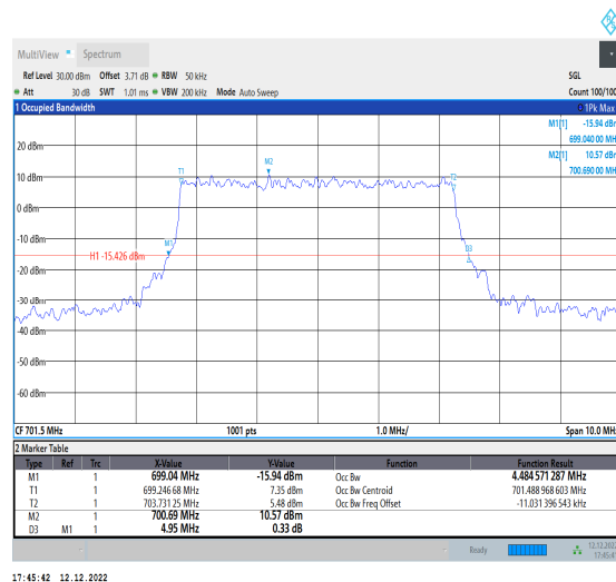
1-N12-15-5-L-4-DFT-64QAM-Outer_Full-25@0-Ant1-4 4.485-4.950-≤5-PASS
