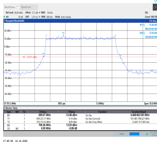
1-N12-15-5-L-2-DFT-PI2BPSK-Outer_Full-25@0-Ant1-4 1-4.468-4.990-≤5-PASS
