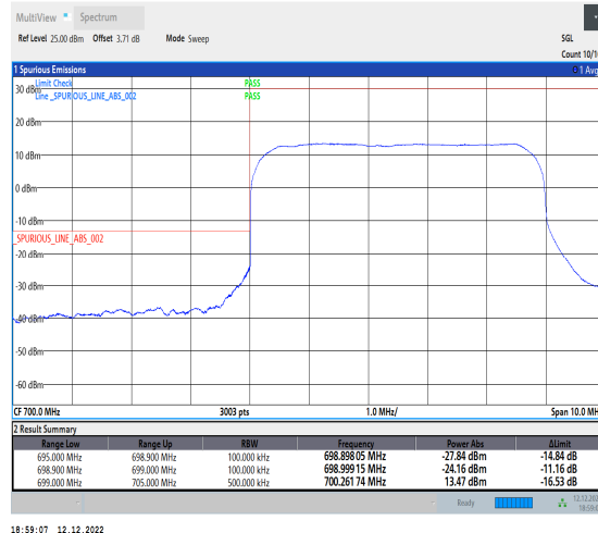
1-N12-15-5-L-3-DFT-PI2BPSK-Outer_Full-25@0-A nt1-1--PASS-see graph
