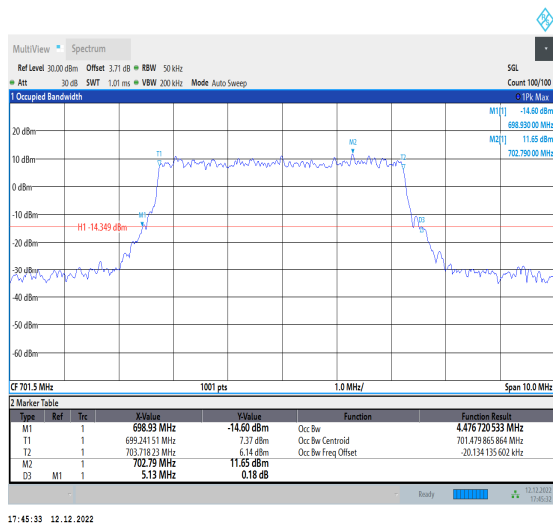
1-N12-15-5-L-3-DFT-16QAM-Outer_Full-25@0-Ant1-4 -4.477-5.130-≤5-PASS
