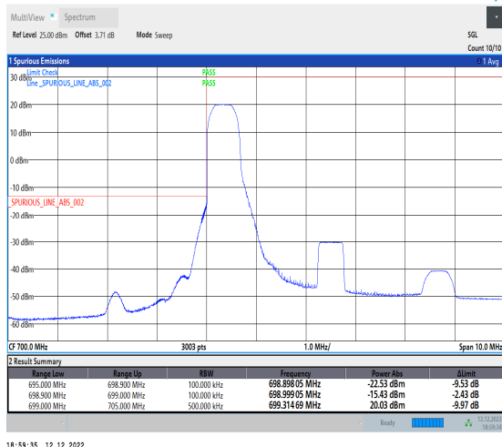
1-N12-15-5-L-4-CP-QPSK-Edge_1RB_Left-1@0-A nt1-1--PASS-see graph
