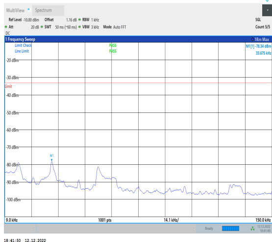
1-N12-15-15-L-1-DFT-PI2BPSK-Inner_1RB_Left-1 @1-0.009-0.15-Ant1-0.03--78.34--33-PASS
