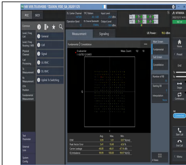
1-N12-15-15-M-5-DFT-256QAM-Outer_Full-75@0-Ant t1-see graph-PASS
