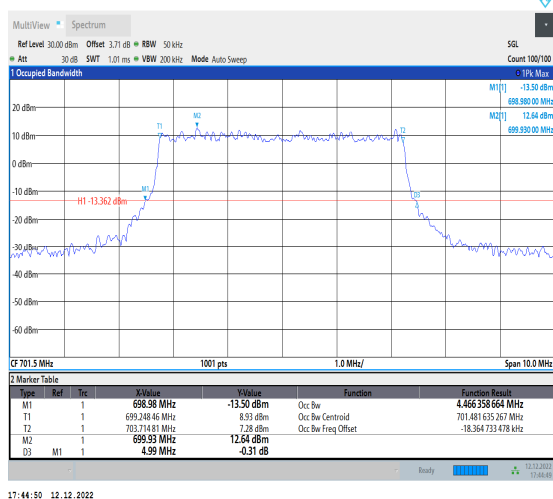
1-N12-15-5-L-1-DFT-QPSK-Outer_Full-25@0-Ant1-4 .466-4.990-≤5-PASS
