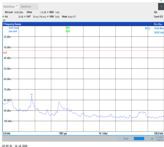
1-N12-15-15-H-1-DFT-PI2BPSK-Inner_1RB_Left-1 @1-0.009-0.15-Ant1-0.03--78.33--33-PASS
