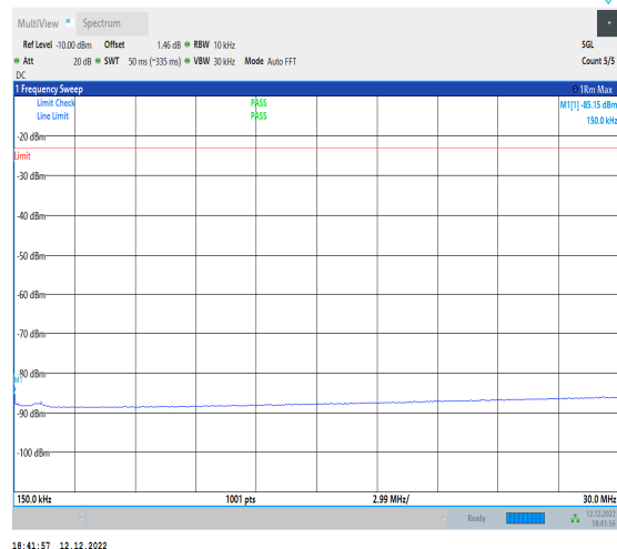
1-N12-15-15-L-1-DFT-PI2BPSK-Inner_1RB_Left-1@ 1-0.15-30-Ant1-0.15--85.15--23-PASS
