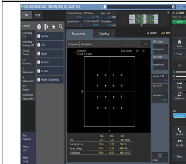
1-N12-15-15-M-7-CP-16QAM-Outer_Full-79@0-Ant1- see graph-PASS
