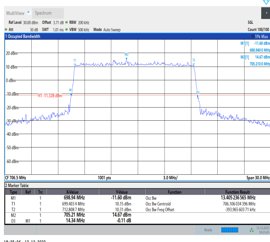
1-N12-15-15-L-1-DFT-QPSK-Outer_Full-75@0-Ant1- 13.405-14.340-≤15-PASS
