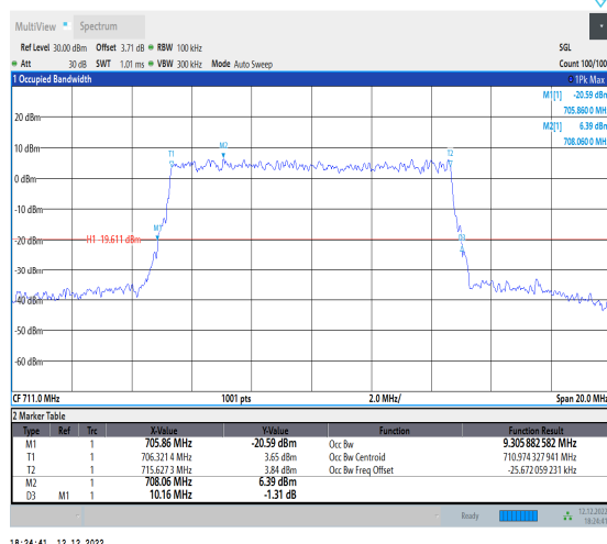
1-N12-15-10-H-9-CP-256QAM-Outer_Full-52@0-Ant1 1-9.306-10.160-≤10-PASS
