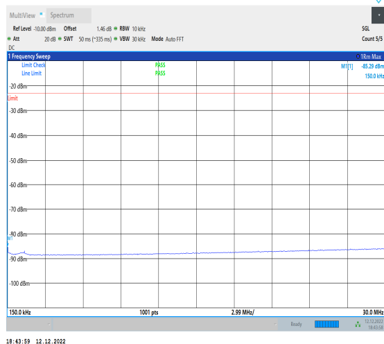
1-N12-15-15-H-1-DFT-PI2BPSK-Inner_1RB_Left-1@ 1-0.15-30-Ant1-0.15--85.29--23-PASS
