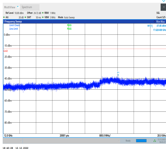
1-N12-15-15-M-1-DFT-PI2BPSK-Inner_1RB_Left-1@ 1-12000-20000-Ant1-17628.40--37.85--13-PASS
