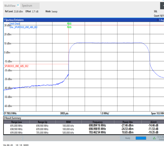
1-N12-15-5-L-6-CP-QPSK-Outer_Full-25@0-A nt1-1--PASS-see graph
