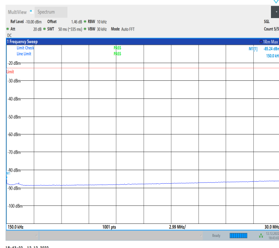
1-N12-15-15-M-1-DFT-PI2BPSK-Inner_1RB_Left-1@ 1-0.15-30-Ant1-0.15--85.24--23-PASS
