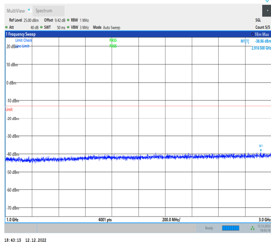
1-N12-15-15-M-1-DFT-PI2BPSK-Inner_1RB_Left-1@ 1-1000-3000-Ant1-2916.50--38.86--13-PASS
