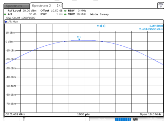
BLE_1M_Low_Channel
