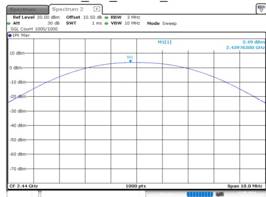
BLE_1M_Middle_Channel
