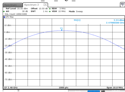
BLE_1M_High_Channel
